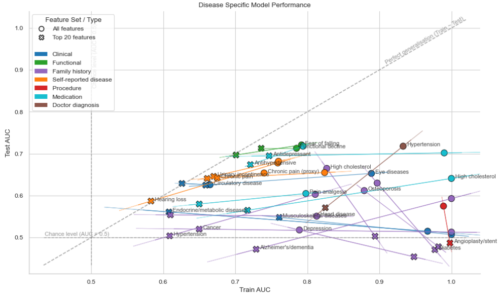
Figure 5.3: Train AUC vs Test AUC for all Track B disease specific models, coloured by outcome category. Circle markers represent all feature models and cross markers represent top-20 feature models, with a line connecting the two feature strategies per disease. The diagonal dashed line marks perfect generalisation (Train \approx Test). Dashed lines at 0.5 on both axes indicate chance level discrimination. Confidence ellipses illustrate within category spread.
