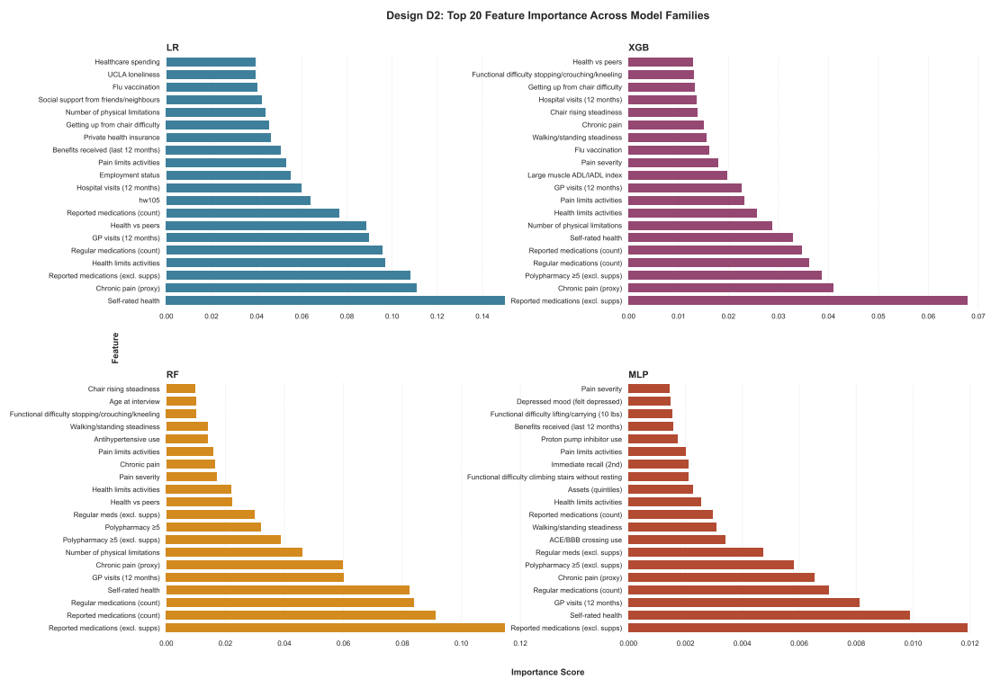
Figure J.2: Top 20 features by importance for D2.
