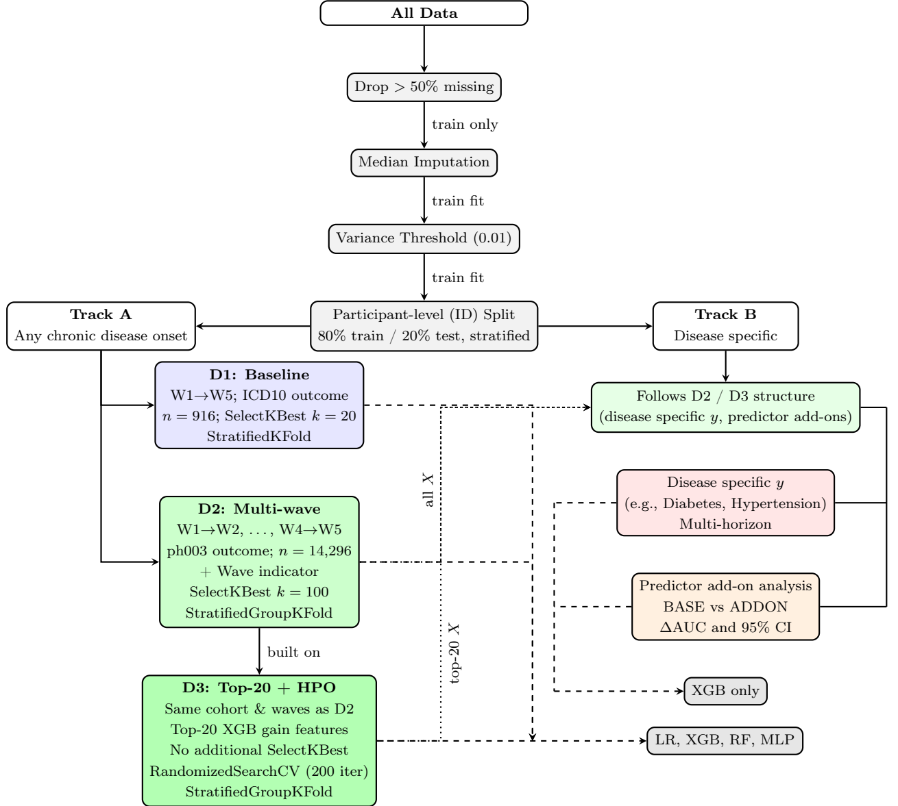
Figure 5.1: Pipeline overview: shared preprocessing applied to all data before branching into Track A (any chronic disease onset, D1/D2/D3) and Track B (disease specific, following D2/D3 structure). D3 is built directly on D2’s cohort and wave structure, adding feature reduction and HPO.
