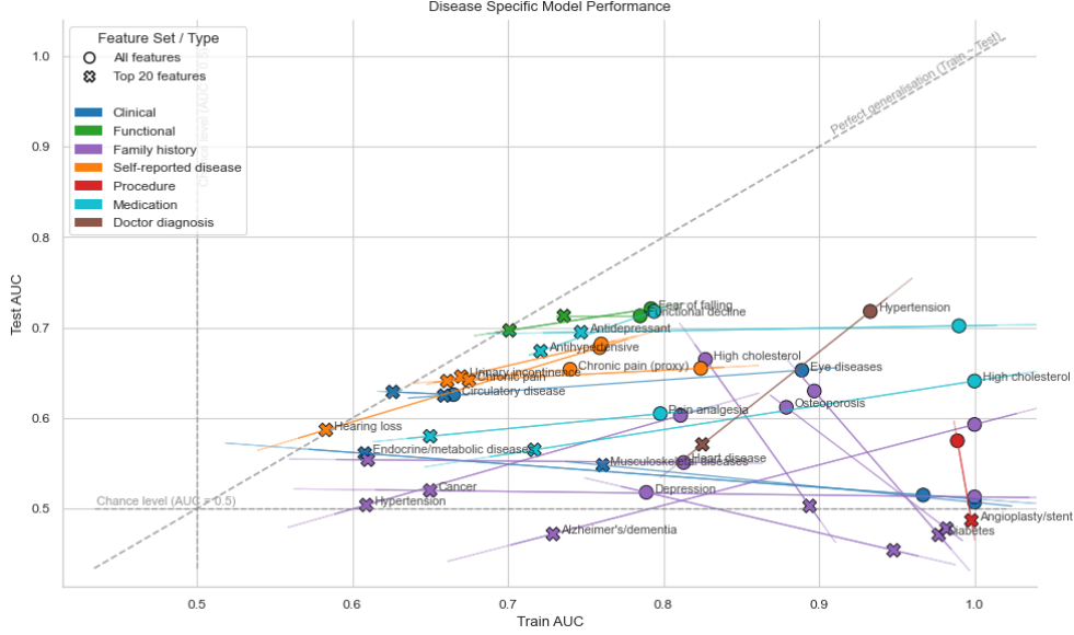
Figure 5.3: Train vs test AUC for all Track B models, coloured by outcome category.
