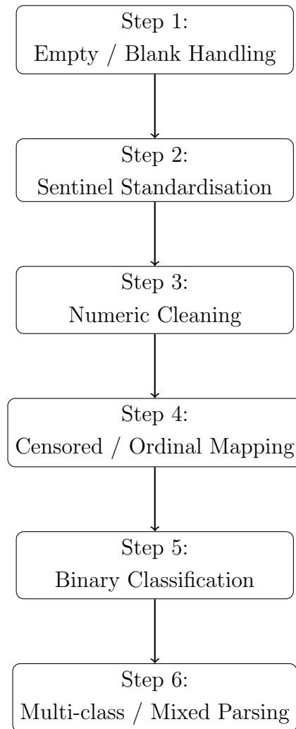
Figure 4.1: Flowchart of the Six Step Cleaning Pipeline applied to all TILDA waves. See full transformation tables in Appendix B.7 and D for detailed scenario progression code at each step.
