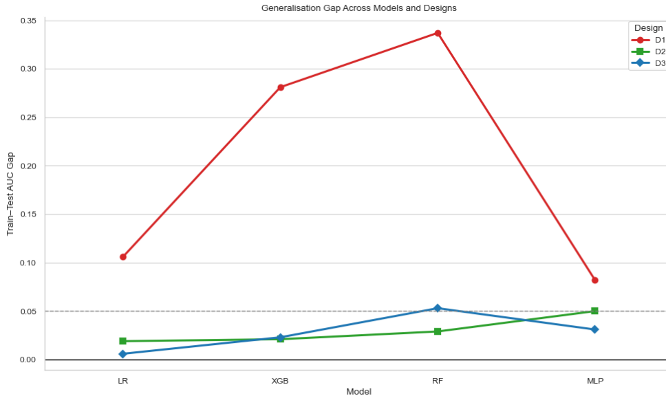
Figure 5.2: Train–test AUC generalisation gaps across models and designs.
