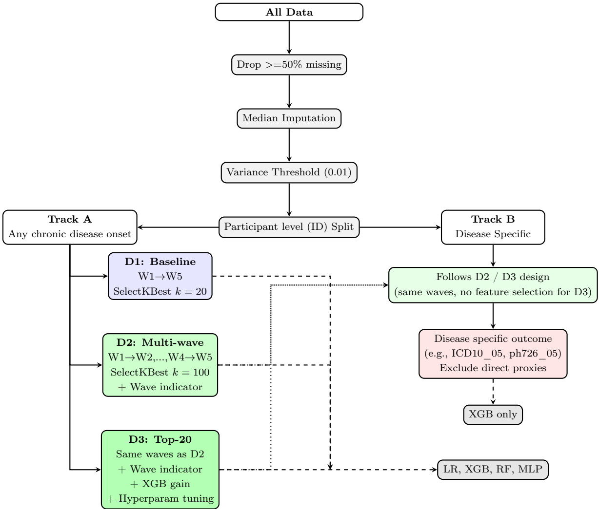
Figure 5.1: Pipeline overview: shared pipeline → separation into Track A (Any chronic disease with D1/D2/D3) and Track B (disease specific, following D2/D3 design).
