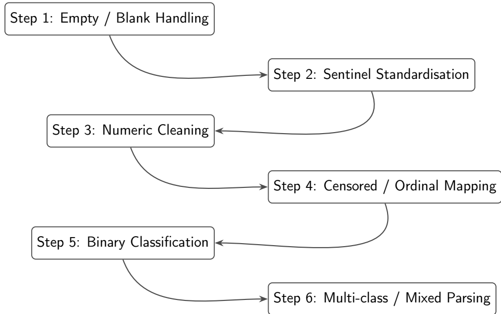
Figure 4.2: Flowchart of the final six-step cleaning pipeline applied to all TILDA waves. Detailed transformation tables are provided in Appendix B.7, and the corresponding implementation “.ipynb” script is documented in Appendix E at each scenario step.
