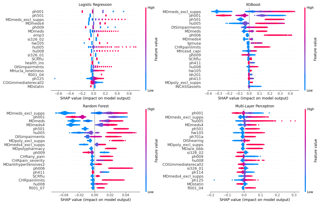
Figure K.2: SHAP value plot for Track A (any disease models D2).
