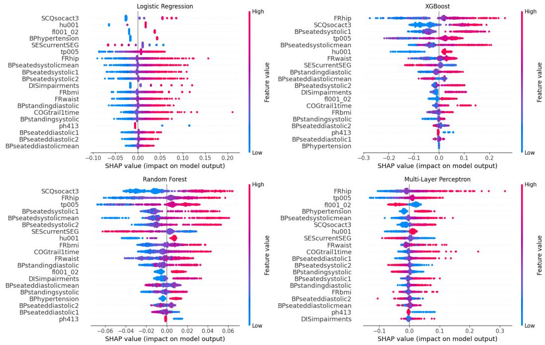
Figure K.1: SHAP value plot for Track A (any disease models D1).
