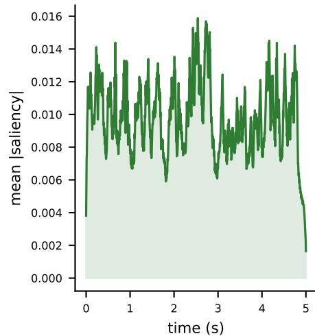
(c) Temporal profile
