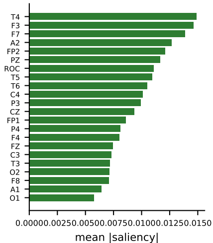
(b) Per-channel importance
