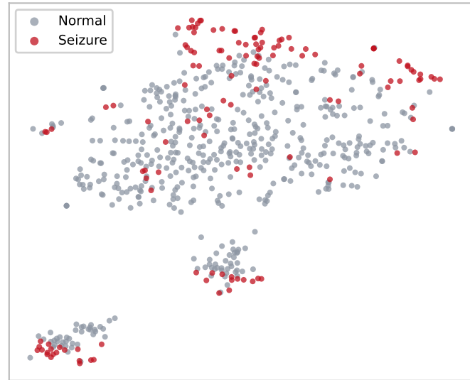
(c) Siena: finetuned + RL embedding (bal. kNN 0.71)
