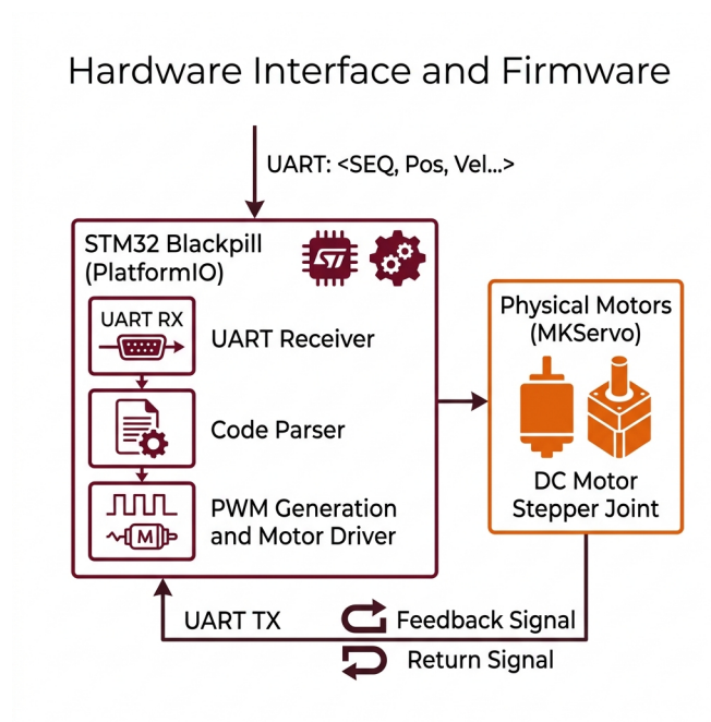
Figure 22: Hardware Layer
