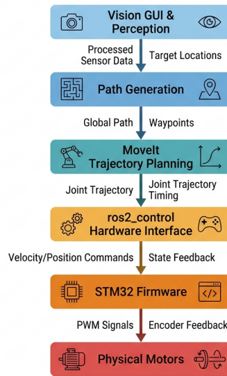
Figure 25: Full Architecture
