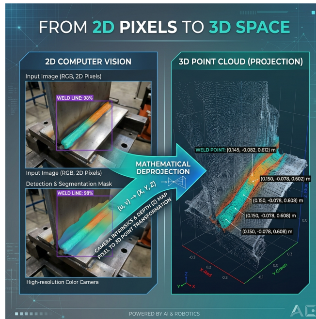
Figure 18: 2D to 3D Deprojection
