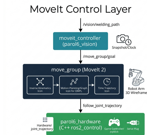
Figure 20: MoveIt Control
