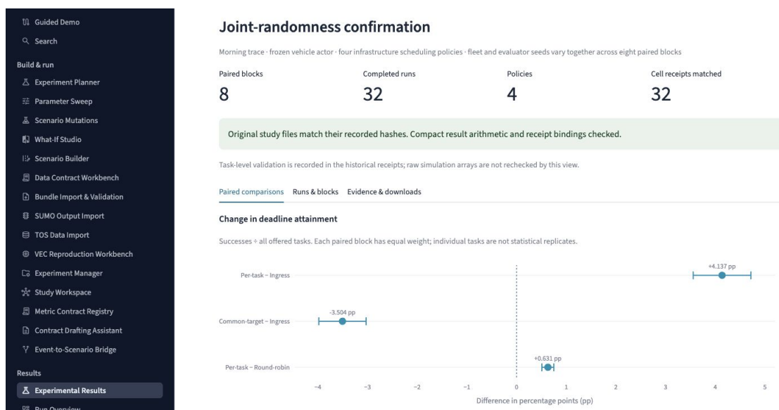
Figure 7: Workflow demonstration of the completed joint-randomness study in TrafficTwin. The interface imports the archived CELL_RESULTS.csv , PAIRED_EFFECTS.csv and receipts, displaying 32 cells across eight paired blocks and the three declared contrasts. File hashes, compact arithmetic and receipt bindings are checked; task-level validation remains the historical receipts' record, and raw simulation arrays are not rechecked. The screenshot demonstrates inspection of existing results, not original experimental execution through the platform, independent scientific validation or a user study [S16], [S17]. Reading: follow the completed campaign's outputs into the results view while retaining their original evidence boundaries.
