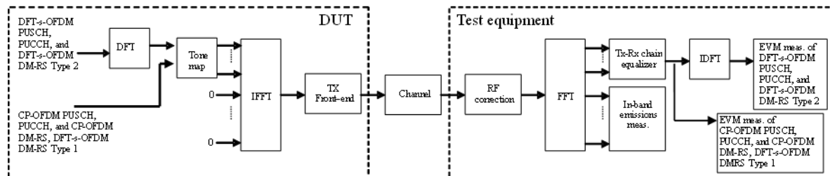
Figure F.1-1: EVM measurement points
