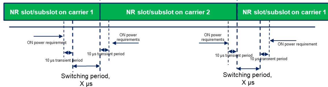
Figure 6.3A.3.3.2-1a: Time mask for switching between UL carrier 1 and UL Carrier 2, where the switching period is located in carrier 1
