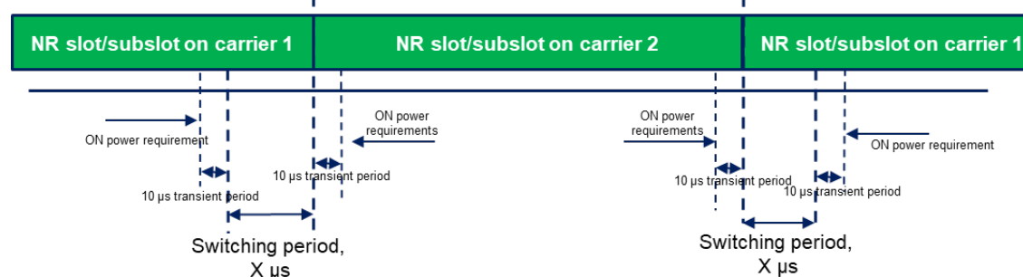
Figure 6.3C.3.1-1a: Time mask for switching between SUL carrier 1 and UL Carrier 2, where the switching period is located in carrier 1
