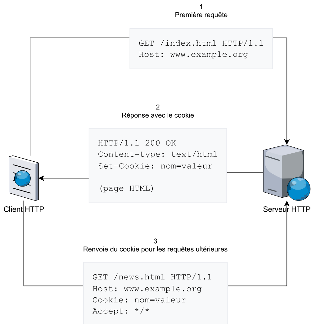
Figure 2.6. Les cookies HTTP
