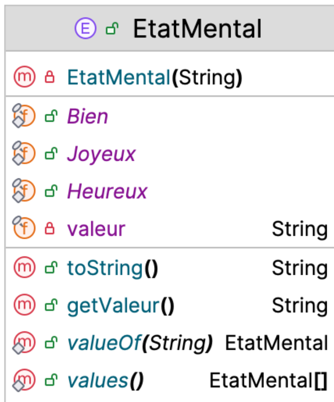
Figure 2.2. EtatMental
