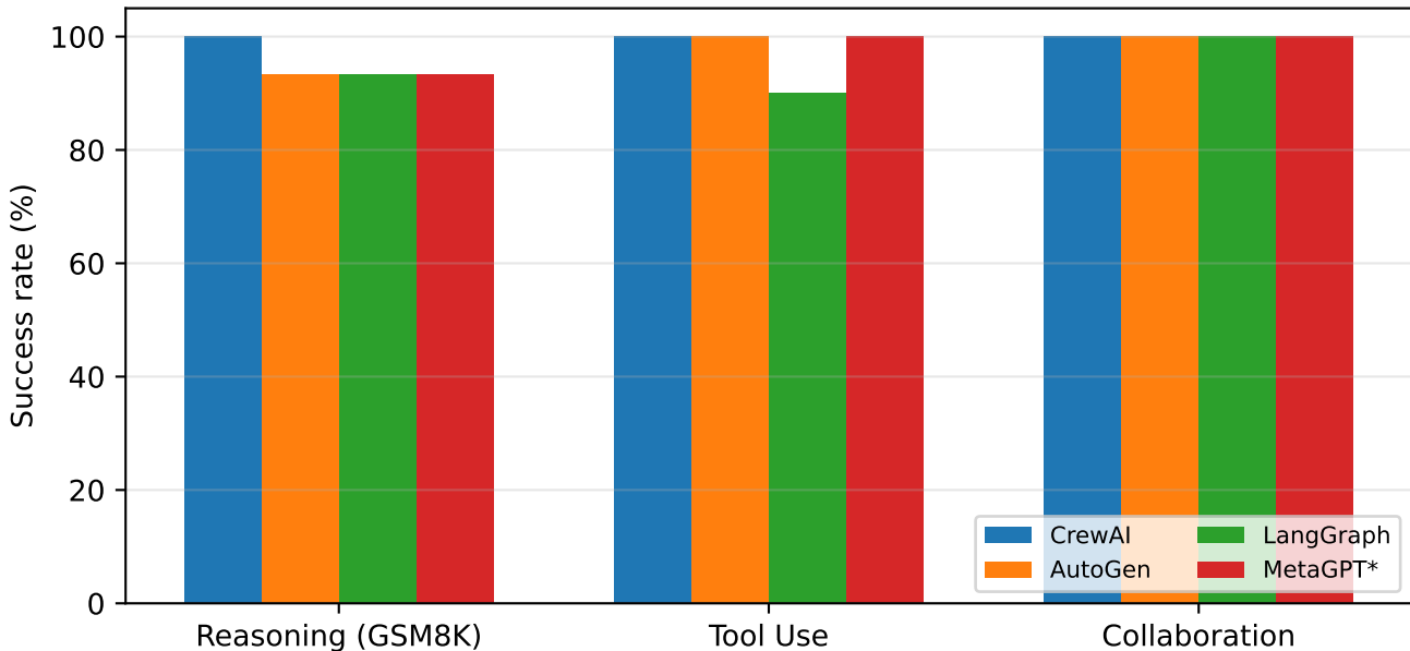
Per-task success rate by framework (gpt-4o-mini backbone)
