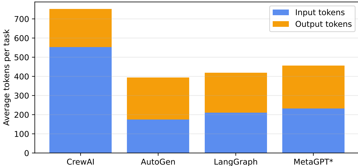
Token consumption per framework (mean across all tasks)
