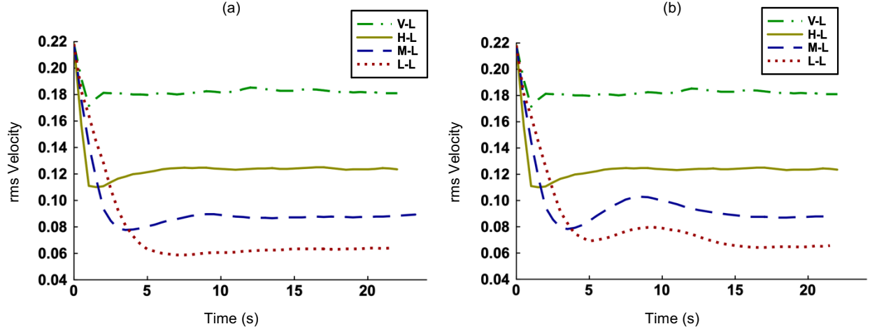
FIG. 21 Time evolution of the rms velocities in (a) Study I, and (b) Study II. ‘V’, ‘H’, ‘M’, and ‘L’ before dash (-) stand for ‘very high’, ‘high’, ‘medium’, and ‘low’ turbulence levels.
