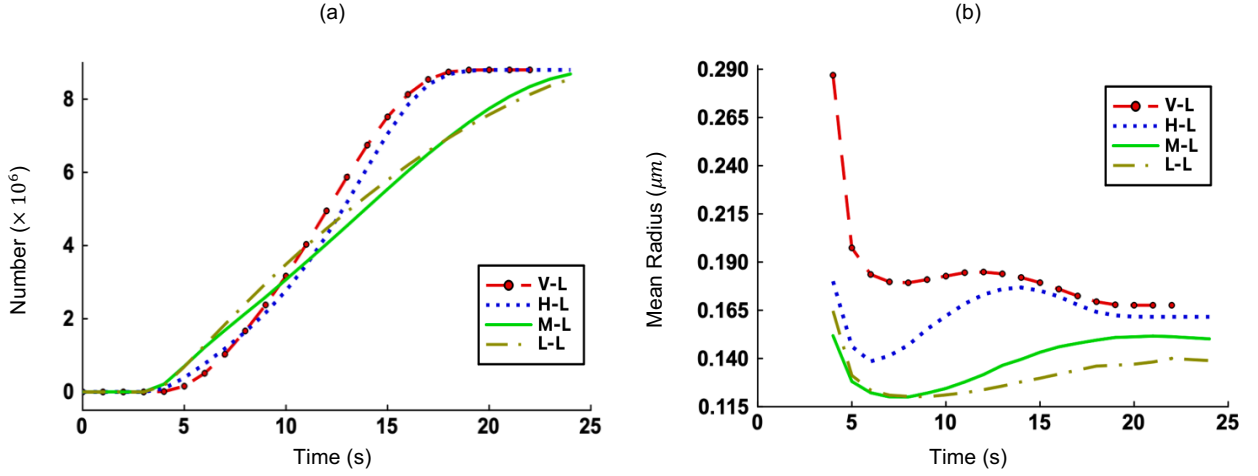
FIG. 19 Evolution of (a) number of aerosol particles, and (b) their mean radius. ‘V’, ‘H’, ‘M’, and ‘L’ before dash (-) stand for ‘very high’, ‘high’, ‘medium’, and ‘low’ turbulence levels.
