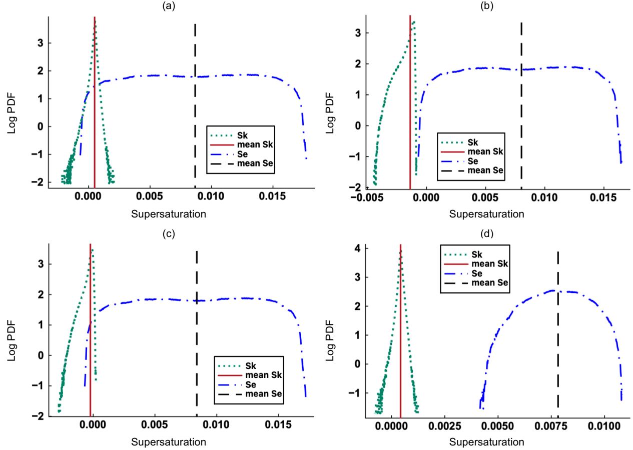
FIG. 14 Log PDFs of instantaneous supersaturation for Cases (a) H-L, (b) H-L', and (c) H-L'', at 3.5 s in Study I. The subplot (d) is analogous for Case H-L at 6 s. The vertical lines indicate the mean values of the respective PDFs.
