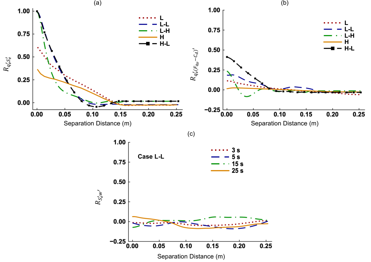
FIG. 6 (a) Correlation coefficient between fluctuations in the water vapor and supersaturation ( R_{q'_v S'_e} ). (b) Correlation coefficient between fluctuations in the q_v and (F_{q_v} - C_d) which is denoted by R_{q'_v (F_{q_v} - C_d)'} . The plots represent the five cases in Scenario I at 25 s. (c) Correlation coefficient between fluctuations in the S_e and w ( R_{S'_e w'} ) for Case L-L in Scenario I at selected times.
