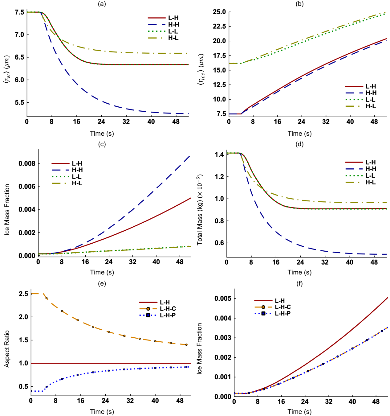
187 Figure 2. Time evolution of the (a) mean radius of cloud droplets, (b) mean radius of ice 188 crystals, (c) ice mass fraction and (d) total mass of particles, for Cases L-H, H-H, L-L, and H-L. 189 Time evolution of the (e) ice crystal aspect ratio and (f) ice mass fraction, for Cases L-H, L-H-C, 190 and L-H-P.
