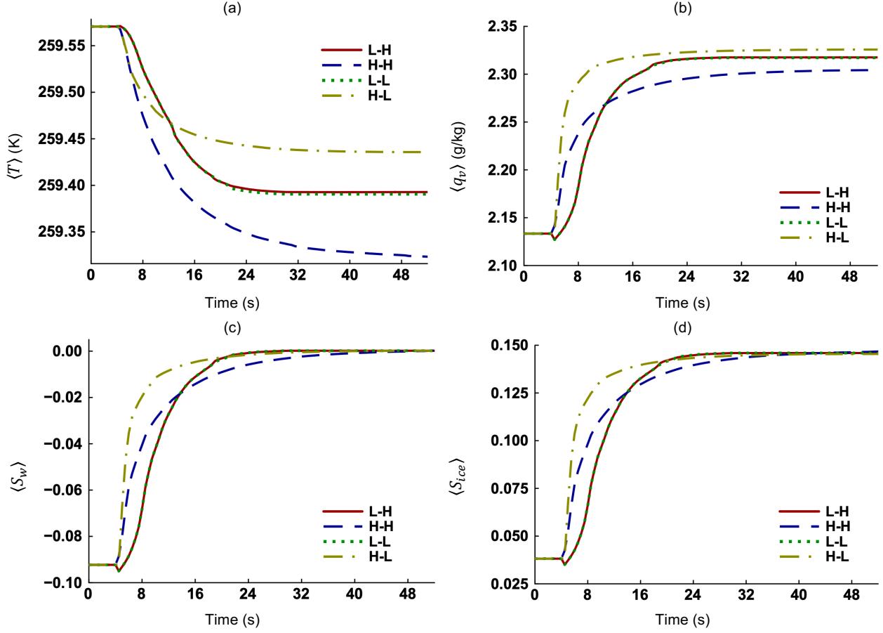
Figure 1. Time evolution of the (a) mean temperature, (b) mean water vapor mixing ratio, (c) mean environmental supersaturation with respect to water and (d) mean environmental supersaturation with respect to ice.
