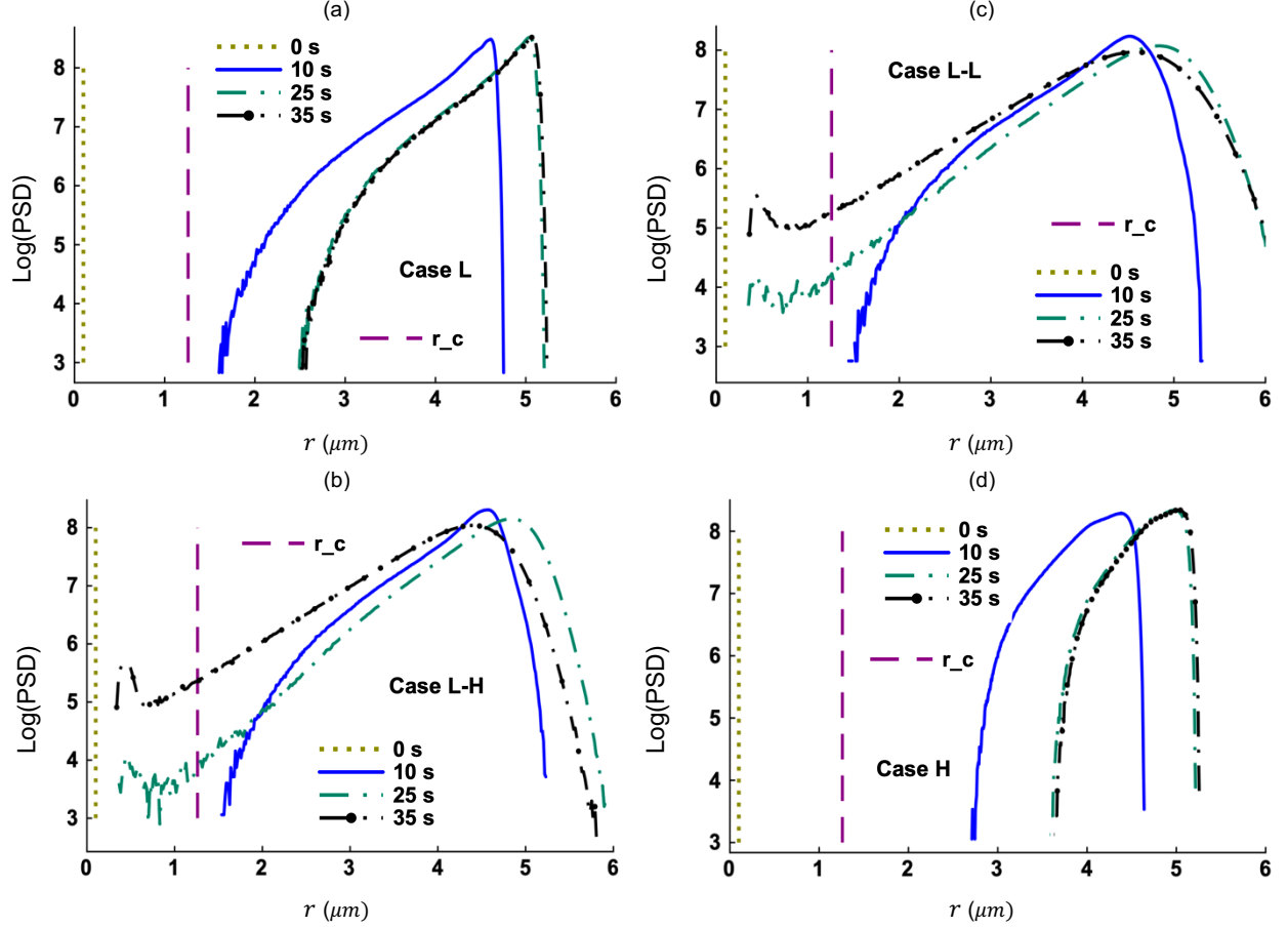
FIG. 10 Particle size distributions (PSDs) for (a) Case L, (b) Case L-H, (c) Case L-L, and (d) Case H at selected times in Scenario I. The ordinate is on a base-10 logarithmic scale. The critical radius ( r_c ) is shown in the dashed vertical line. The r in the abscissa includes both aerosol and cloud particles. The unit of PSD is \mu\text{m}^{-1}\text{cm}^{-3} .
