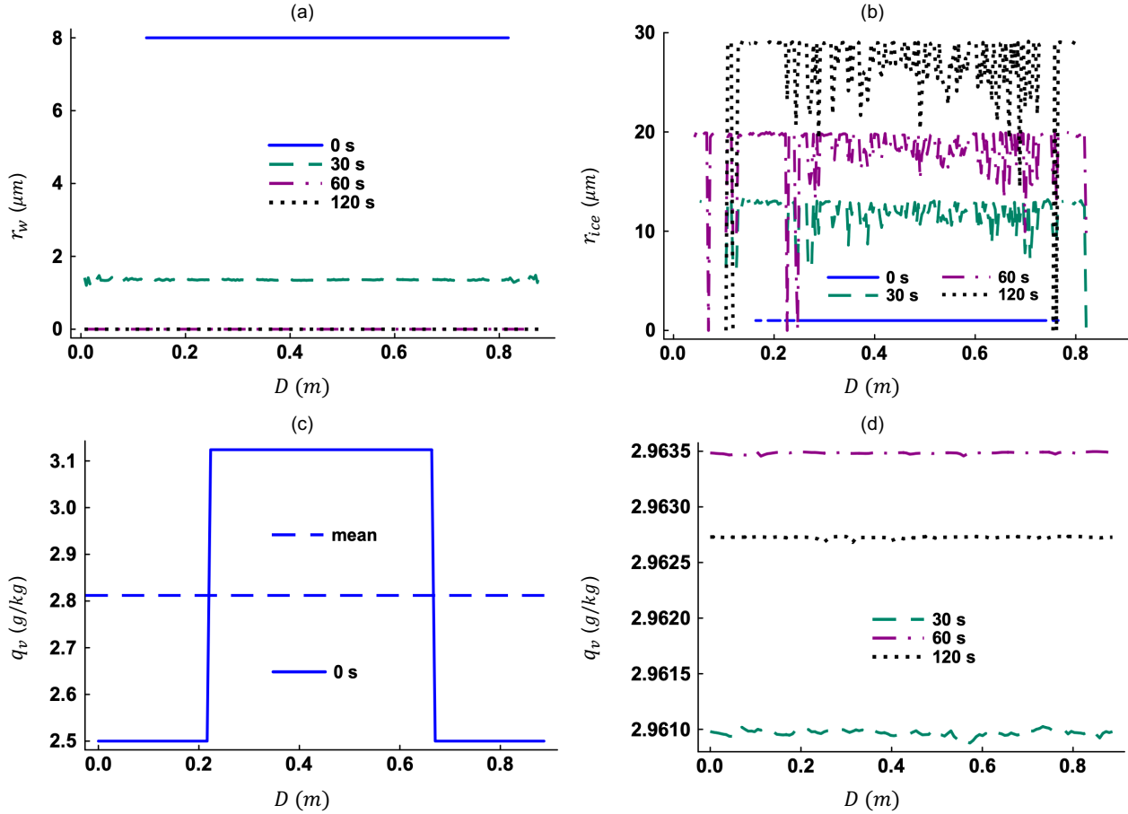
Figure 3. The spatial distributions of the (a) r_w and (b) r_{ice} at selected times. The spatial distributions of the q_v at (c) 0 s and at (d) other selected times. Note that D is the main diagonal of our 3D domain. These results represent Case H-S-L.
