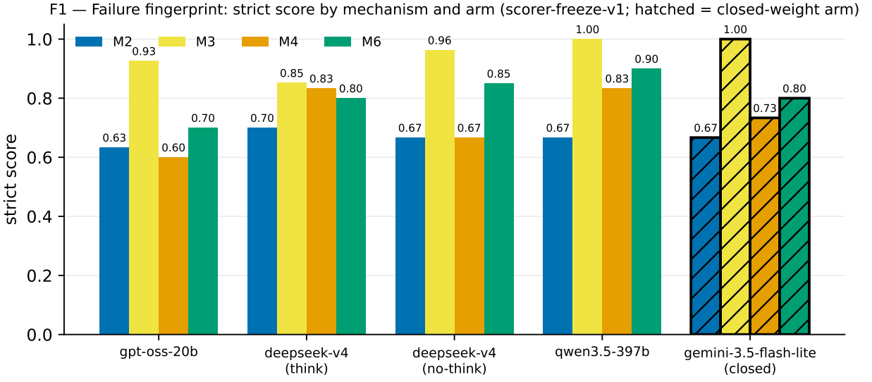
Figure 1: F1: strict-score fingerprints per arm and mechanism.
