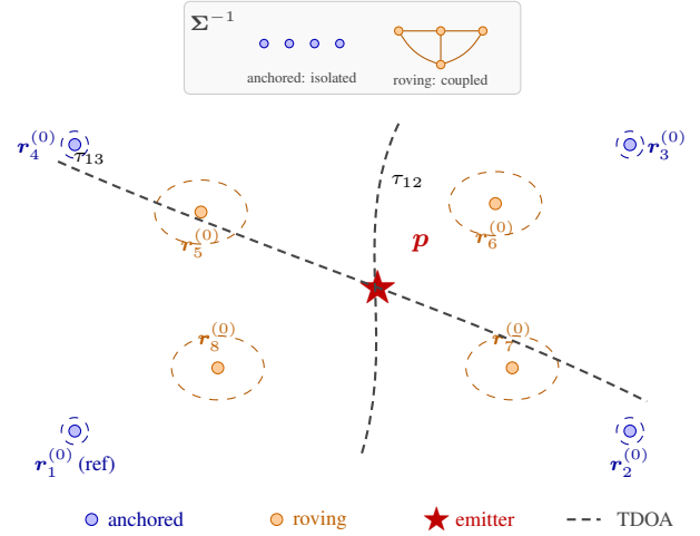
Fig. 1. Multistatic TDOA geometry with uncertain sensor poses ( N_r = 8 , heterogeneous regime of Section VI-B): four anchored receivers (blue, \sigma_{\text{anch}} = 0.1\text{ m} ) and four roving receivers (orange, \sigma_{\text{rov}} \sim 10\text{ m} ), with \mathbf{r}_1^{(0)} the TDOA reference. Grey curves sketch two constant-TDOA hyperbolic loci \tau_{12} , \tau_{13} through \mathbf{p} . Inset: sparsity of \Sigma^{-1} —anchored receivers isolated, roving receivers edge-coupled by shared-GNSS and swarm-frame correlations; its kernel jointly with \mathbf{1}_{N_r} \otimes \mathbf{I}_D governs identifiability via Theorem 1.
