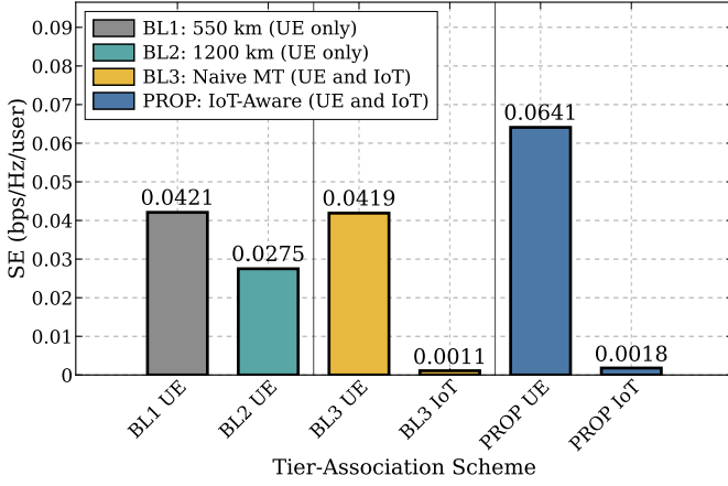
Fig. 3: Comparison of per-device average spectral efficiency. The proposed method significantly outperforms static baselines by intelligently balancing link quality against cross-tier resource loads.
