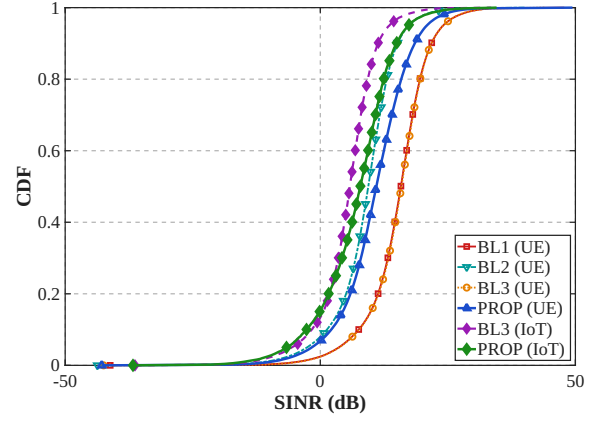
(a) SINR CDF for UE and IoT devices under the evaluated tier-association schemes.
