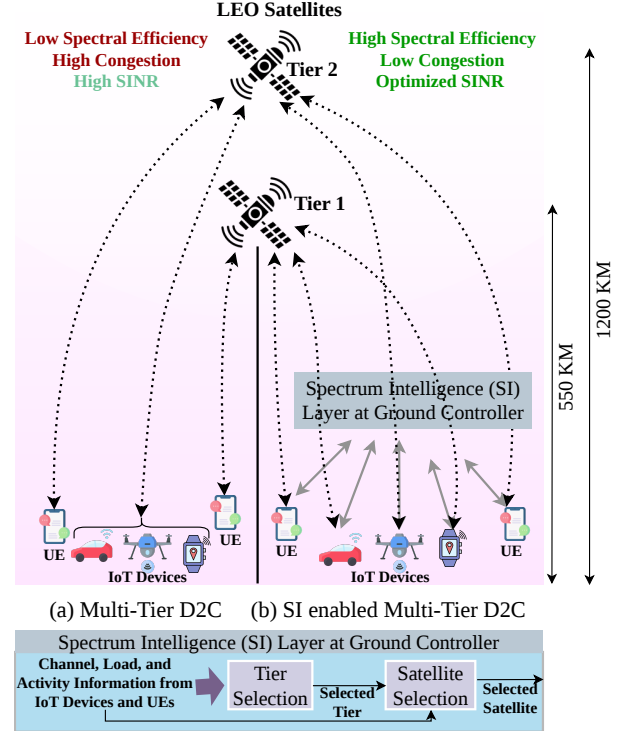
Fig. 1: Conceptual overview of the proposed architecture. (a) A baseline multi-tier D2C network suffering from load imbalances, spectrum congestion, and sub-optimal link efficiency. (b) The proposed multi-tier D2C framework utilizing a spectrum intelligence layer at the ground controller, which dynamically utilizes device telemetry to optimize Tier and Satellite selection.
