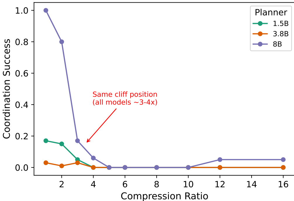
Model Size Affects Ceiling, Not Cliff Position
