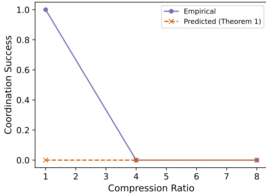
Predicted vs Empirical Cliff
