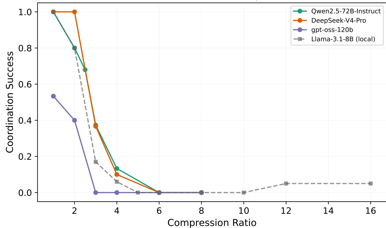
Frontier Model Cliff Comparison
