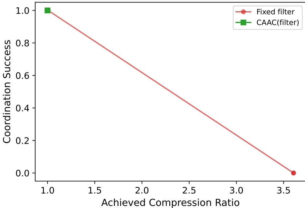
CAAC vs Fixed-Ratio Compression
