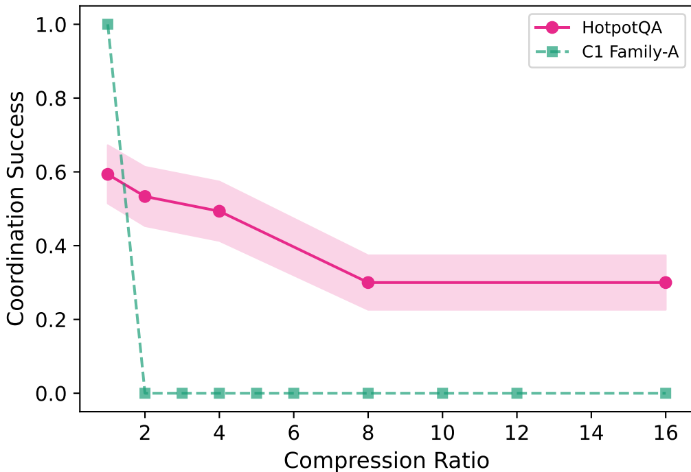
HotpotQA vs C1: Coordination Cliff Comparison
