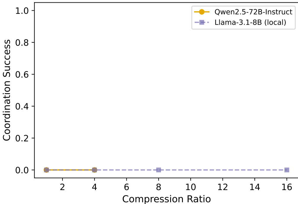
Frontier vs Local: Coordination Cliff
