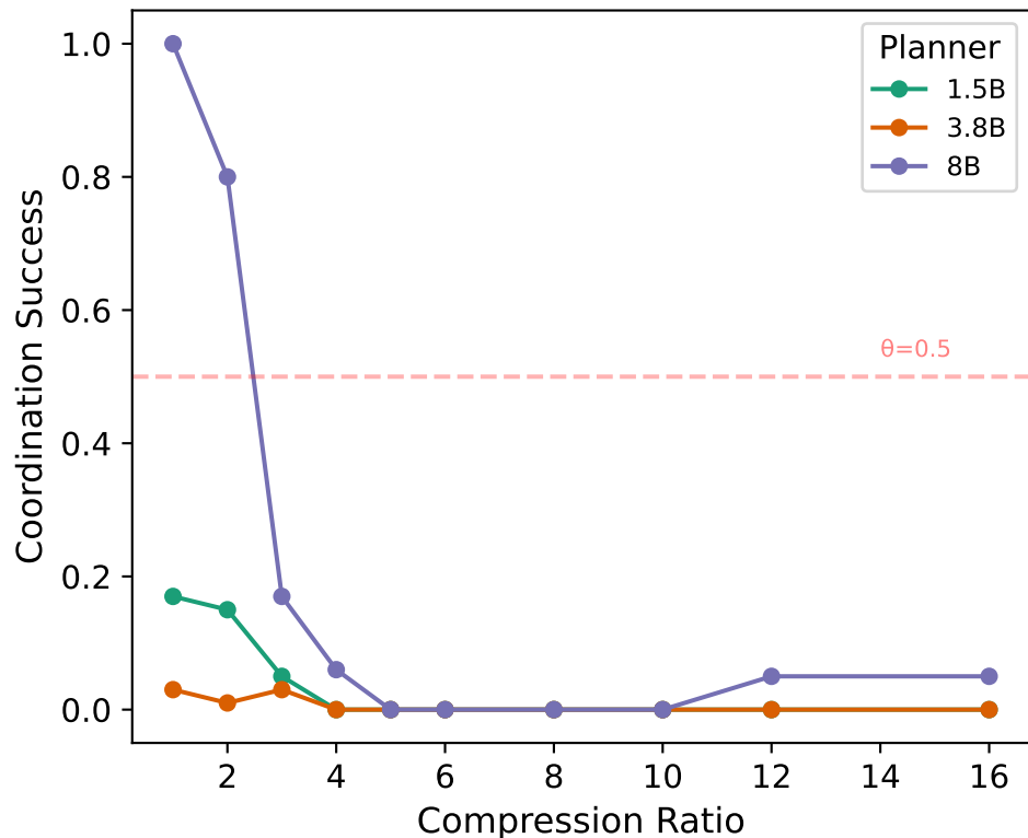
Cliff Position Is Model-Invariant
