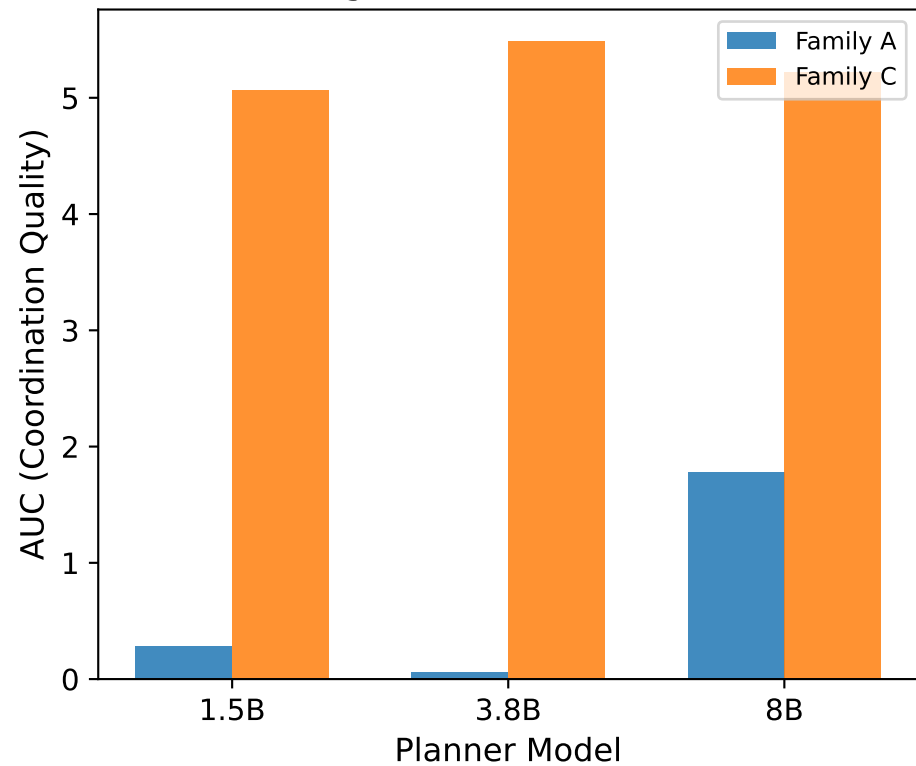
Ceiling Scales with Model Size
