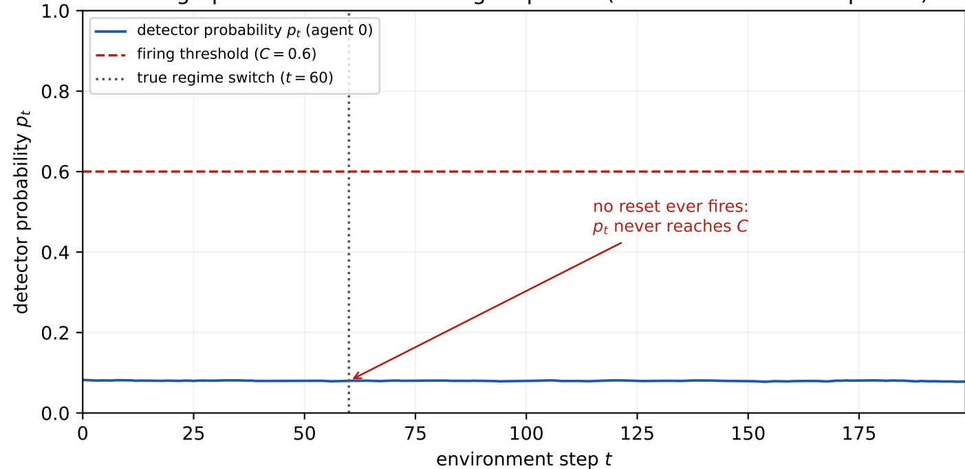
Change-point detection on a single episode (no detection in this episode)
