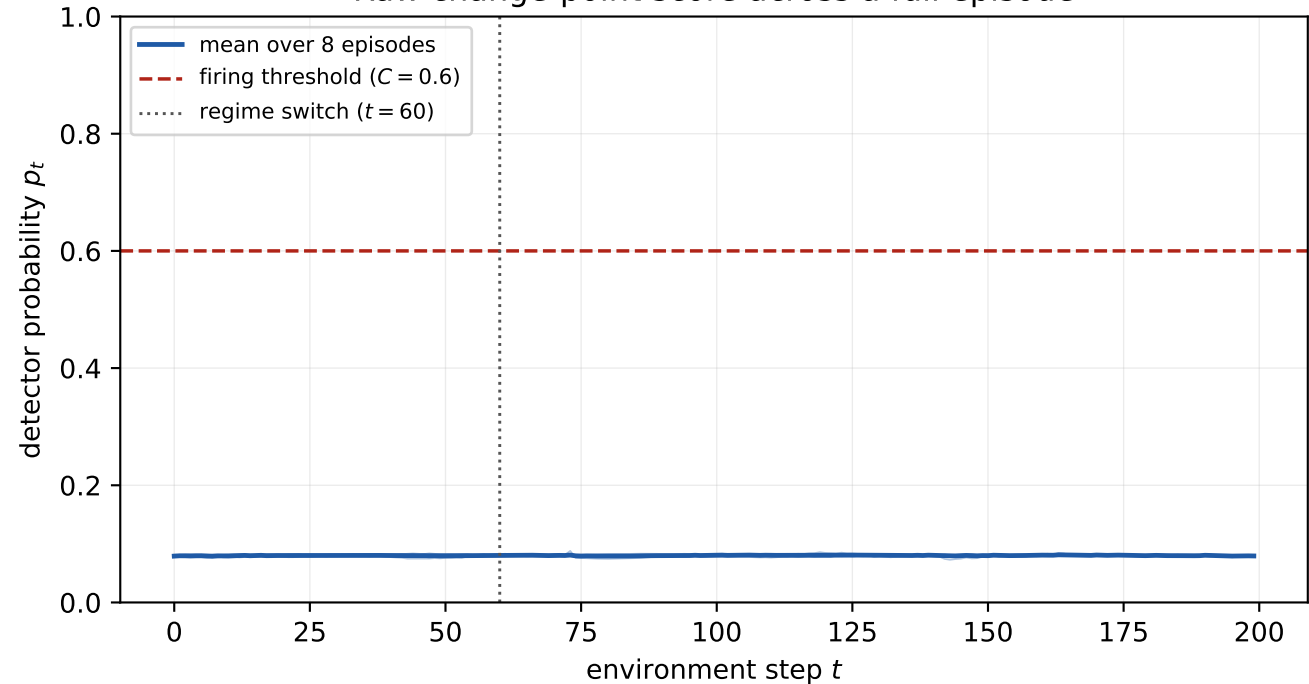
Raw change-point score across a full episode
