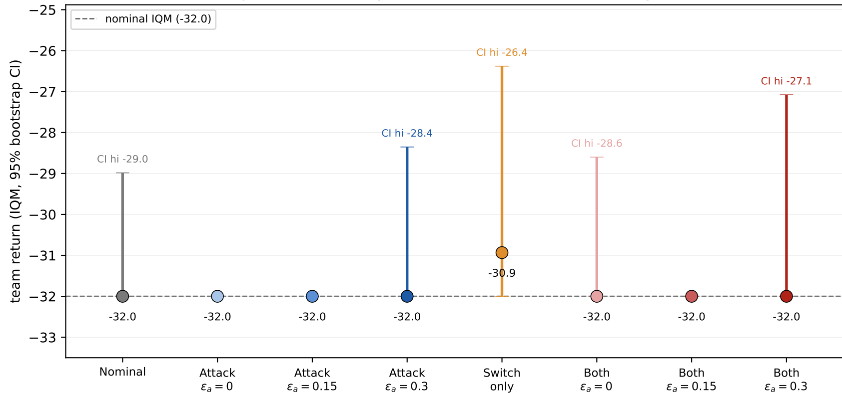
Nominal performance vs. performance under attack and regime switch
