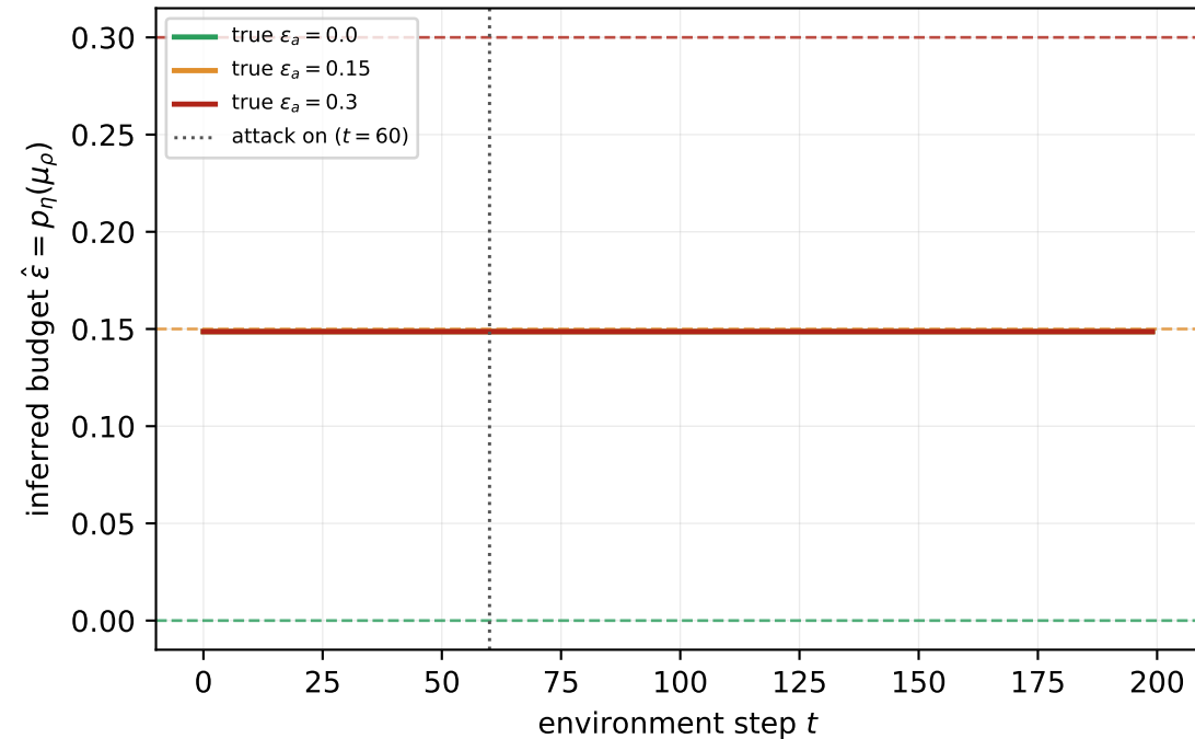
(a) Inferred vs. true perturbation budget
