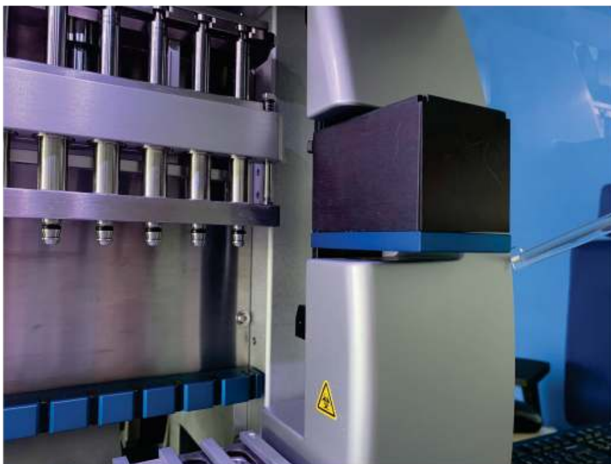
Figure 18. Camera module.
