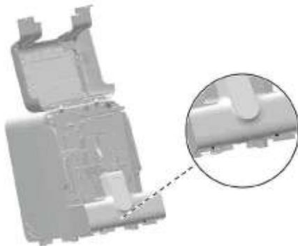
Figure7-183 Removing the right cover
