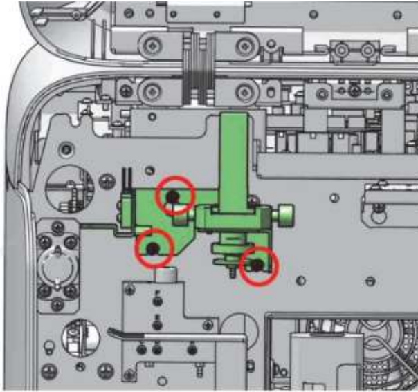
Figure7–571 Diagram of Screw Fixing Location of the Flyorescence Dye Pump Asm (Exclude RET)
