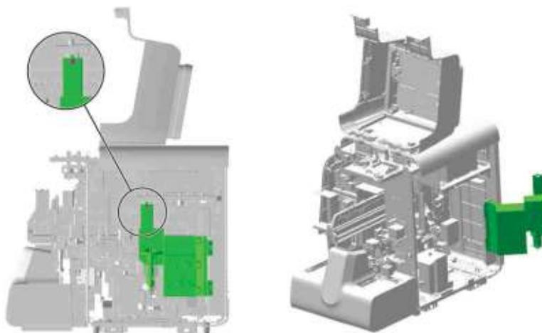
Figure7-127 Opening the right cover assembly
