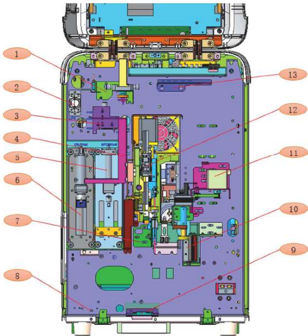
Figure2–5 Front View of the Analyzer (Front Cover Open)
