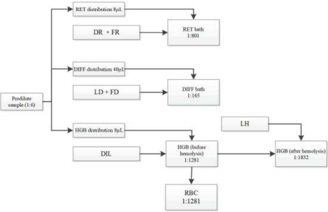
Figure2–14 Prediluted Sample Dilution Flowchart
