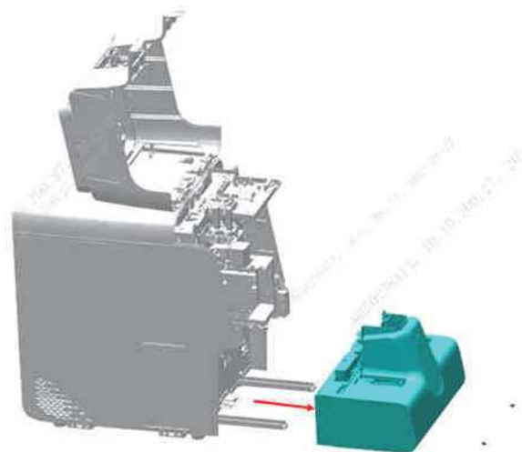
Figure7–279 Removing the autoloader assembly
