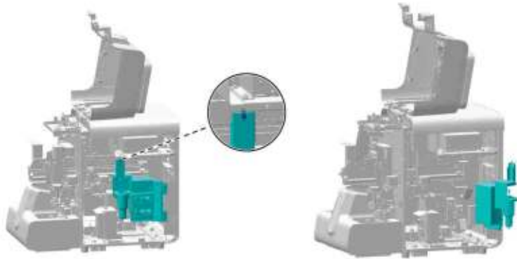
Figure7-112 Opening the right cover assembly
