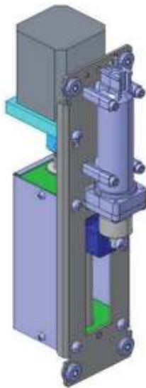
Figure7-442 Photo of 10 mL lead screw driving syringe assembly
