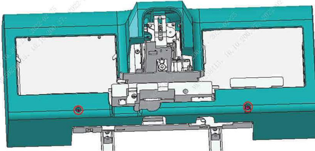
Figure7–267 Removing autoloader front cover assembly (10x5)
