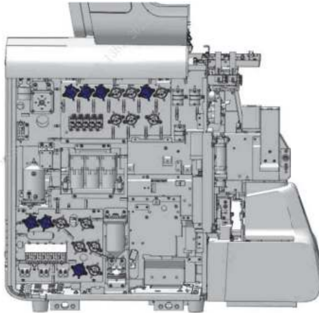
Figure7–518 Diagram A for Location of Three-way Valve (PEIZH)
