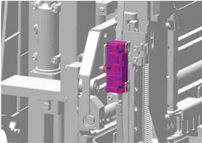
Figure7–89 Positions of the set screws of the ESR flexible board
