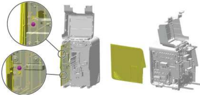
Figure7–108 Removing the left cover
