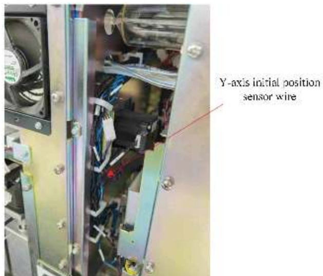
Figure7-72 Removing the Y-direction initial position sensor wires of sampling
