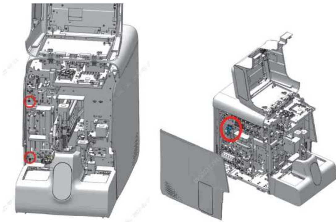
Figure7-545 Removing the covers
