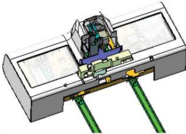
Figure7–344 Diagram of Location of Autoloader, Closed-Sampling Model (10x5) (Excluding Capillary Blood Mixing) in the Main Unit
