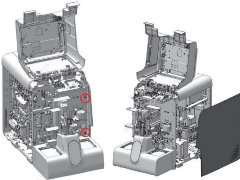
Figure7–524 Diagram C of Location of Two-way Valve (PEIZH)
