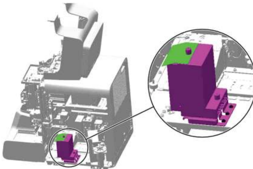
Figure7–382 Removing the shielding cover of the sheath fluid impedance assembly
