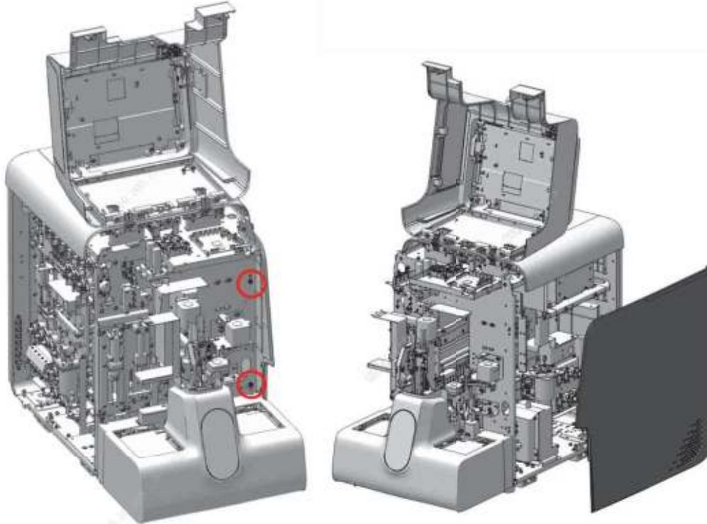
Figure7-483 Diagram for Location of Removing the Covers
