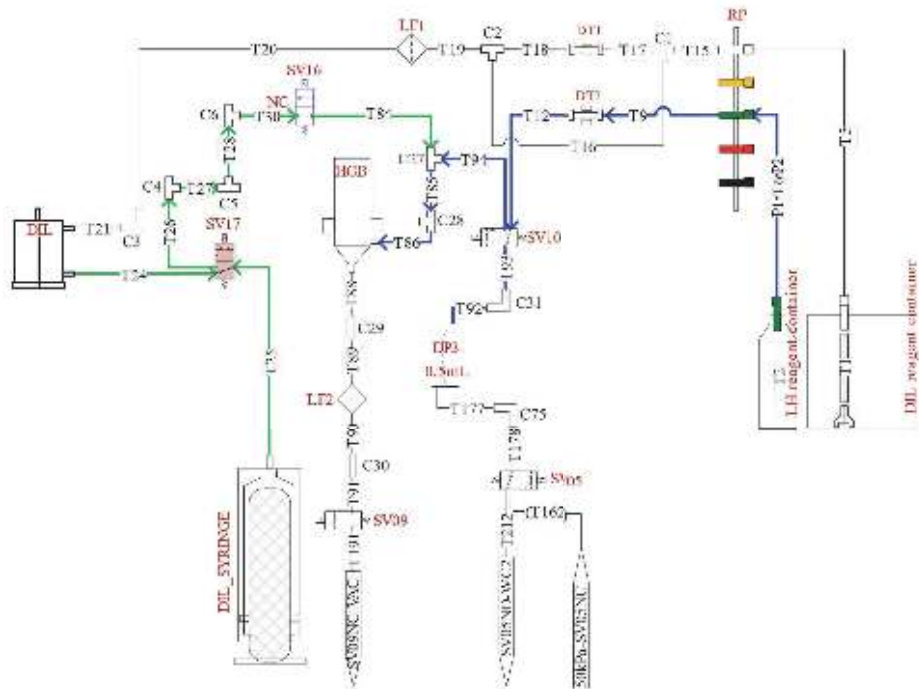
Figure2-34 RBC Measurement Channel
