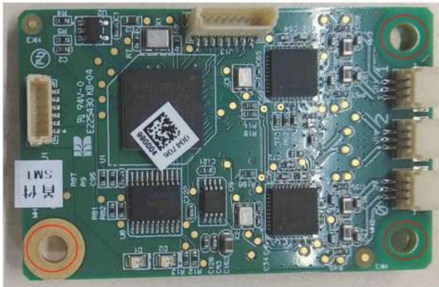
Figure7–622 Diagram of RFID Card Reader Screw Installation Positions
