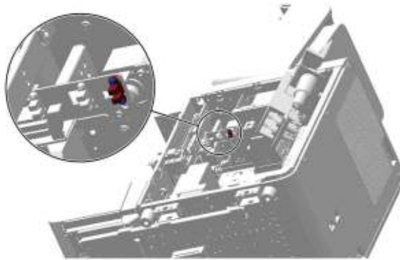
Figure7–84 Positions of the set screws of the detecting sensor
