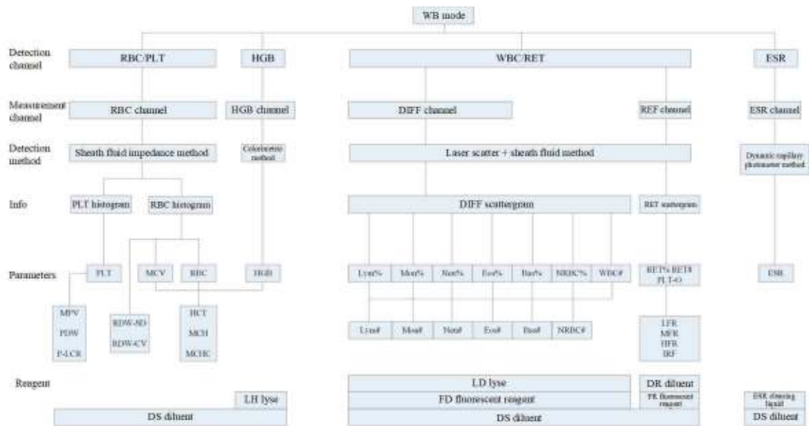
Figure2–12 Analysis Flowchart
