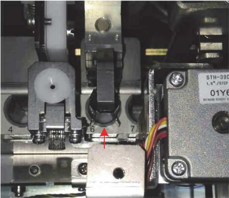
Figure7–248 Confirming the Mixing Mechanism Position in the Left-to-right Direction
