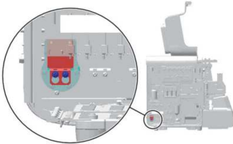
Figure7–470 Positions of set screws of the diaphragm pump adapter bracket
