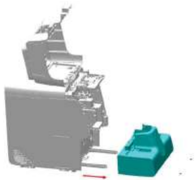
Figure7-184 Figure 1 - Removing the tube gripper
