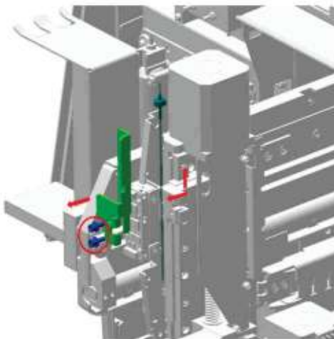
Figure7–156 Removing the piercing probe
