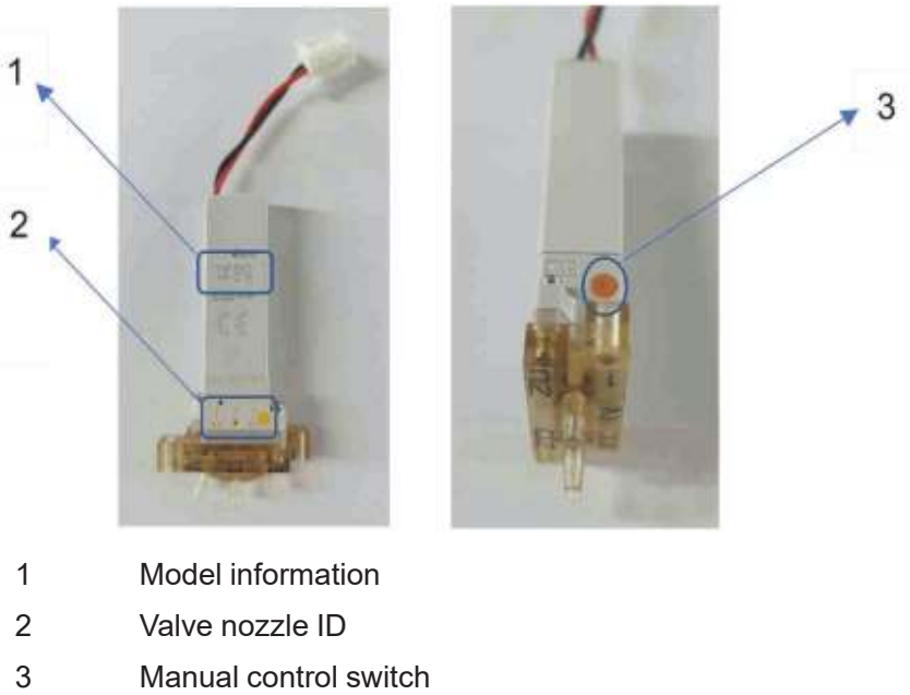
Figure2–17 SMC Valve
