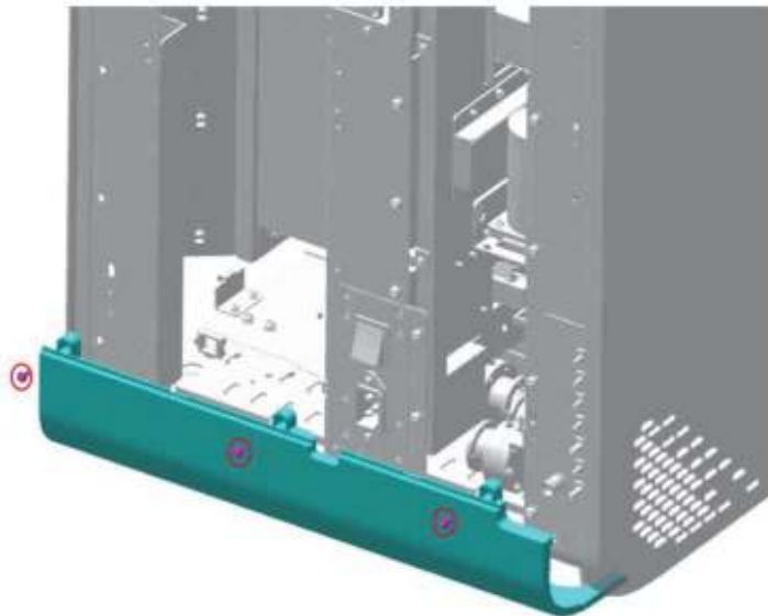
Figure7–660 Removing the Bottom Shell
