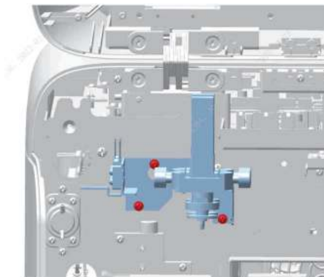
Figure7–570 Diagram of Screw Fixing Location of the Flyorescence Dye Pump Asm (Include RET)
