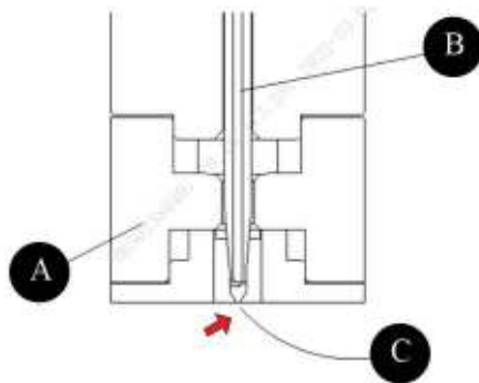
Figure7–36 Sampling probe tip Pos. (Adjustment target position/observation position)
