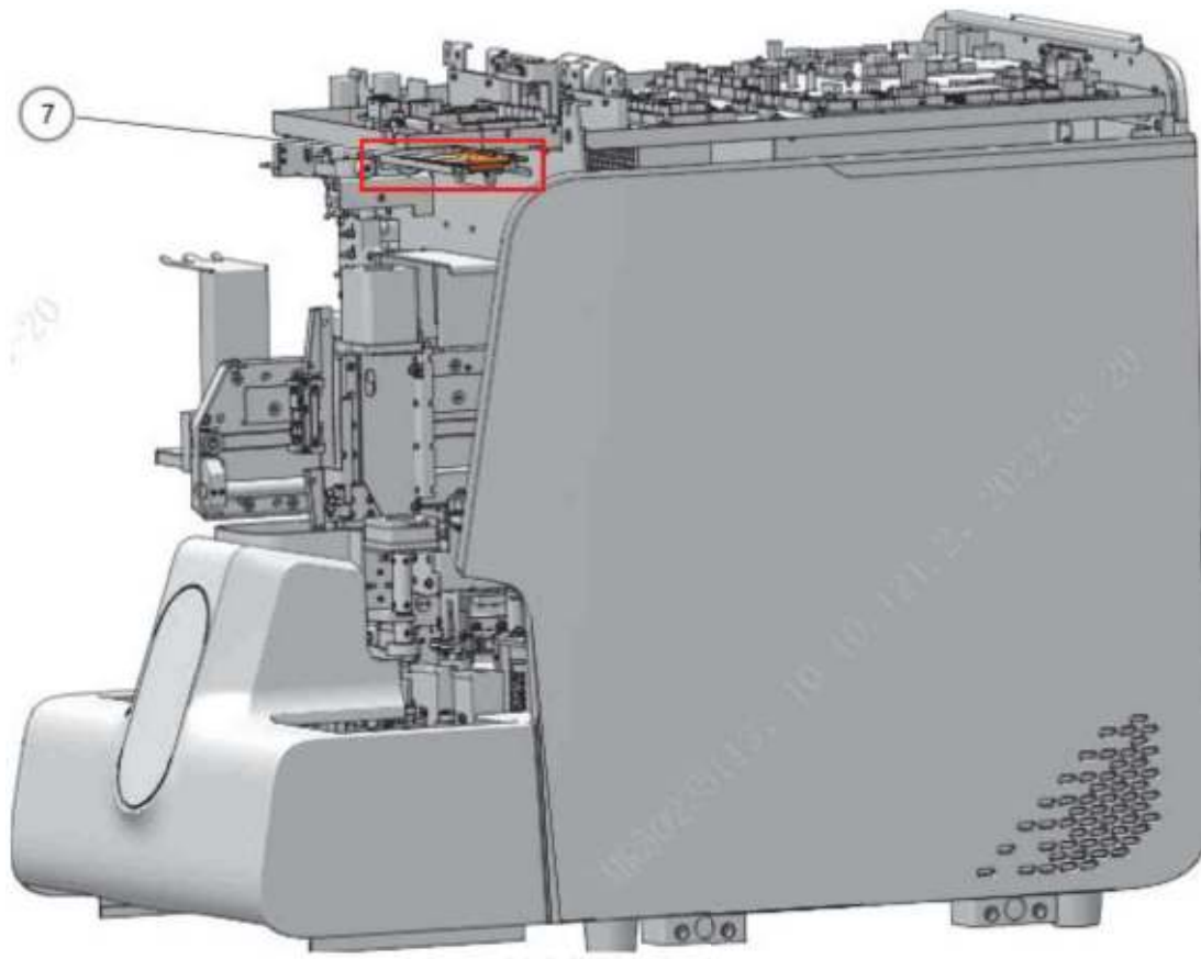
Figure7-601 Diagram of Board Position
