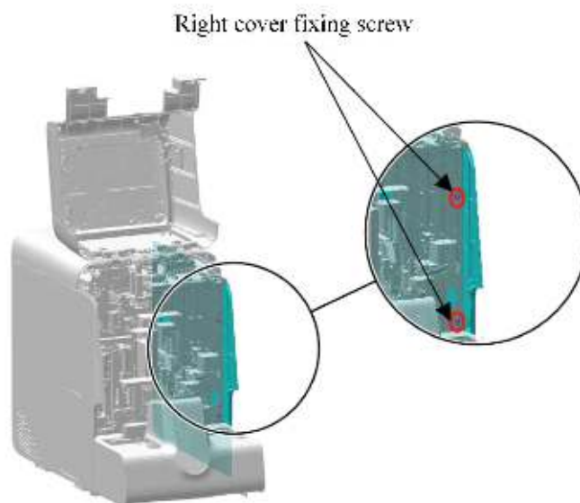
Figure7–657 Diagram of Removing the Right Cover
