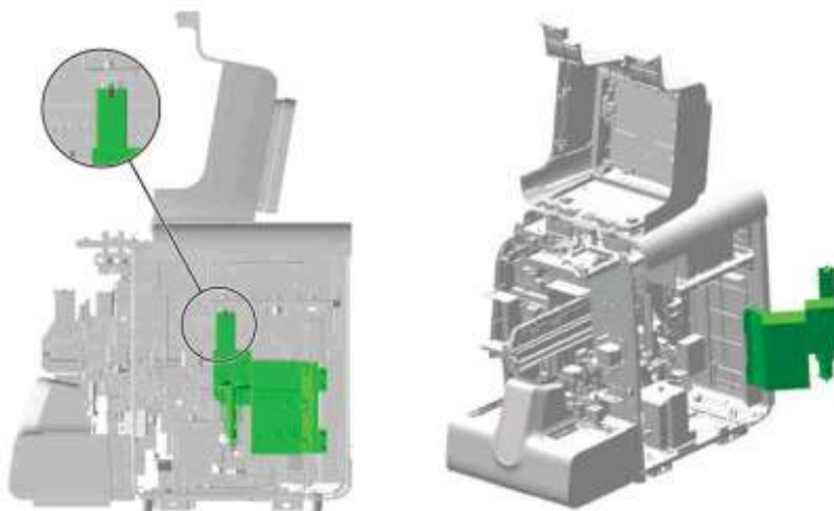
Figure7-132 Opening the right cover assembly
