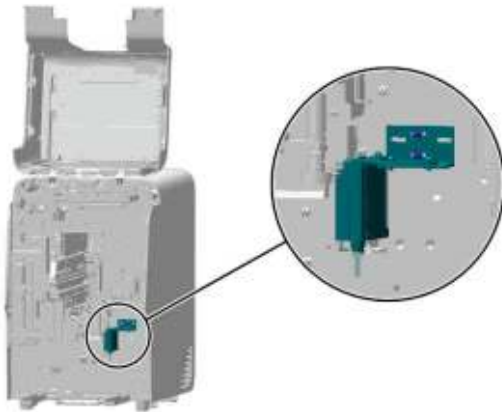
Figure7-185 Figure 2 - Removing the tube gripper
