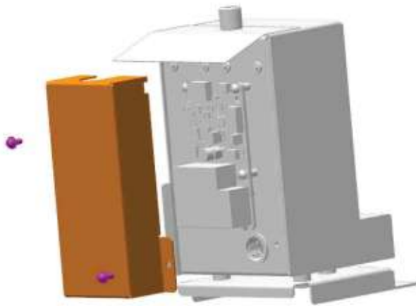
Figure7–399 Diagram of Removing the Shielding Cover of Impedance Signal Board
