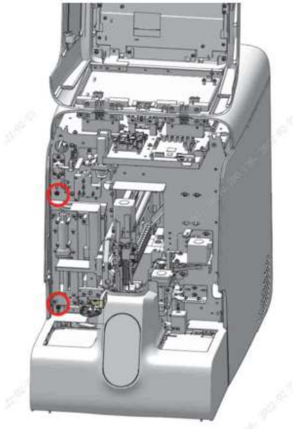
Figure7–554 Diagram B of Location of the Filter Assembly
