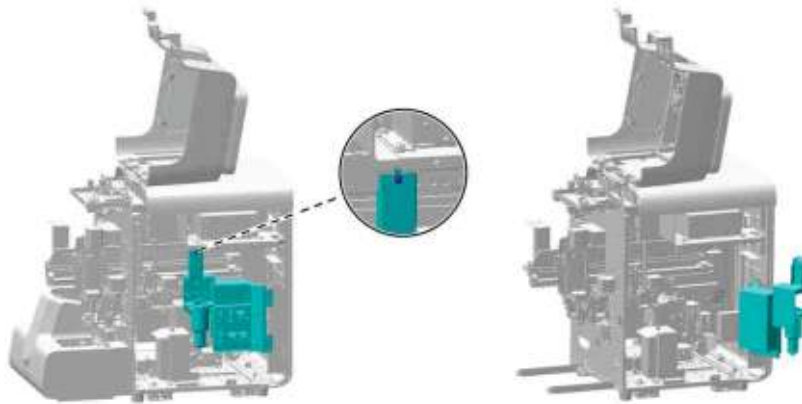
Figure7–381 Opening the right cover assembly
