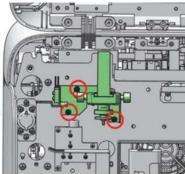
Figure7–578 Diagram A of Screw Fixing Location of the Flyorescence Dye Pump Asm (Exclude RET)
