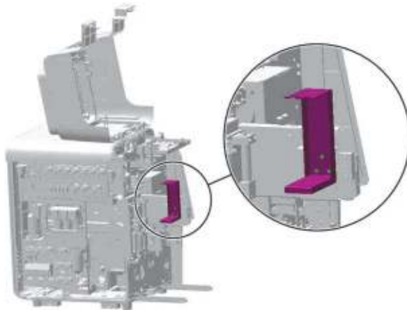
Figure7–480 Diagram of Removing the Left Cover
