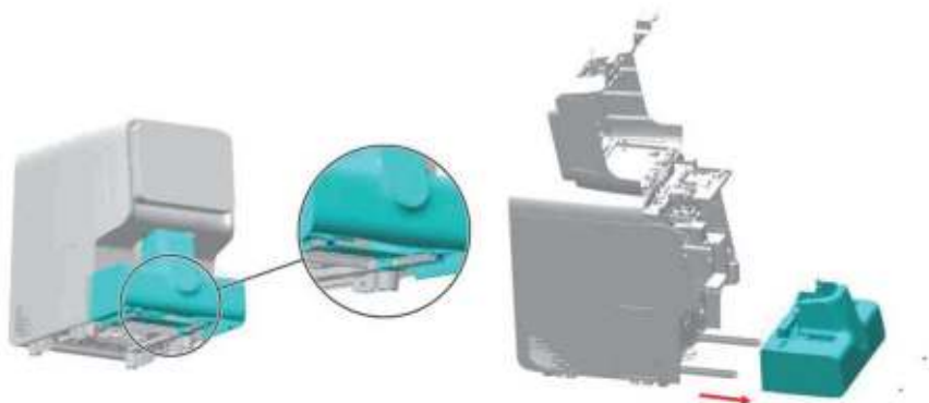
Figure7–443 Removing the autoloader
