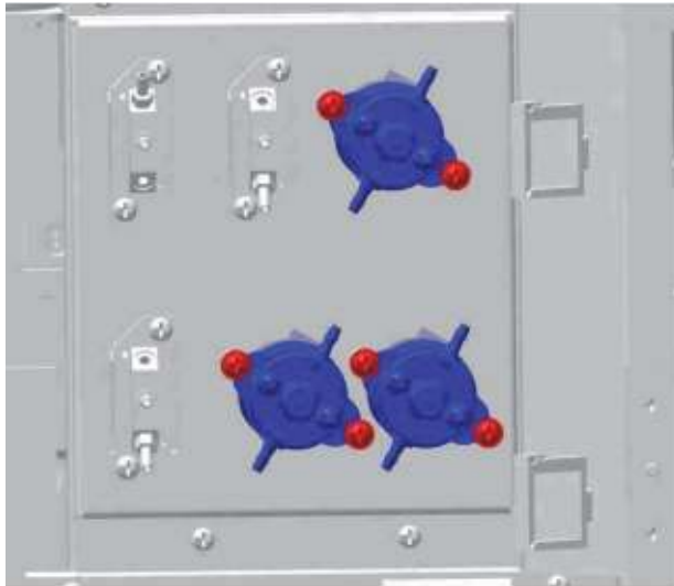
Figure7–525 Positions of set screws of two-way valve (PEIZH)
