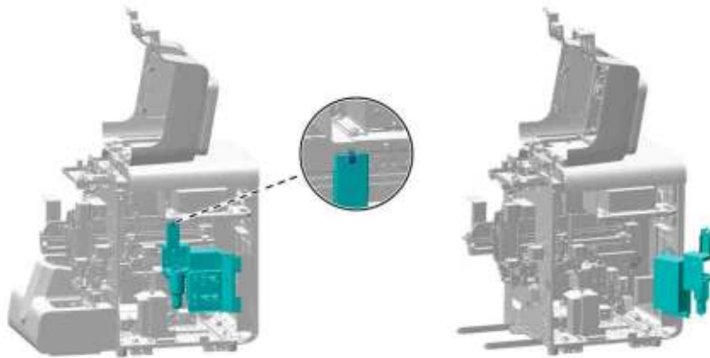
Figure7–367 Opening the right cover assembly
