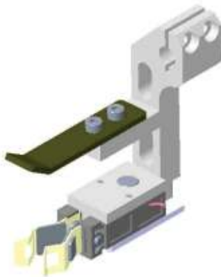
Figure7-168 Photo of Tube Gripper
