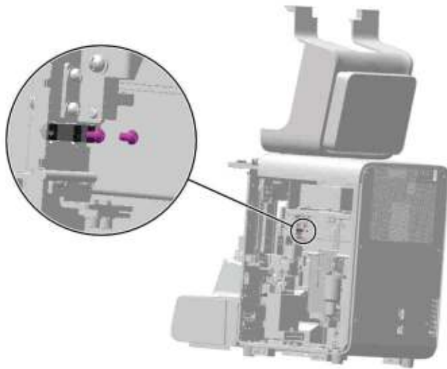
Figure7–114 Removing the sensor fixing plate
