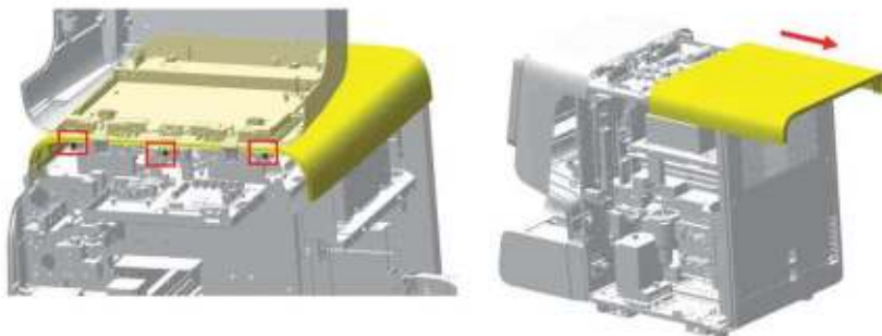
Figure7-630 Diagram of Removing the Top Cover
