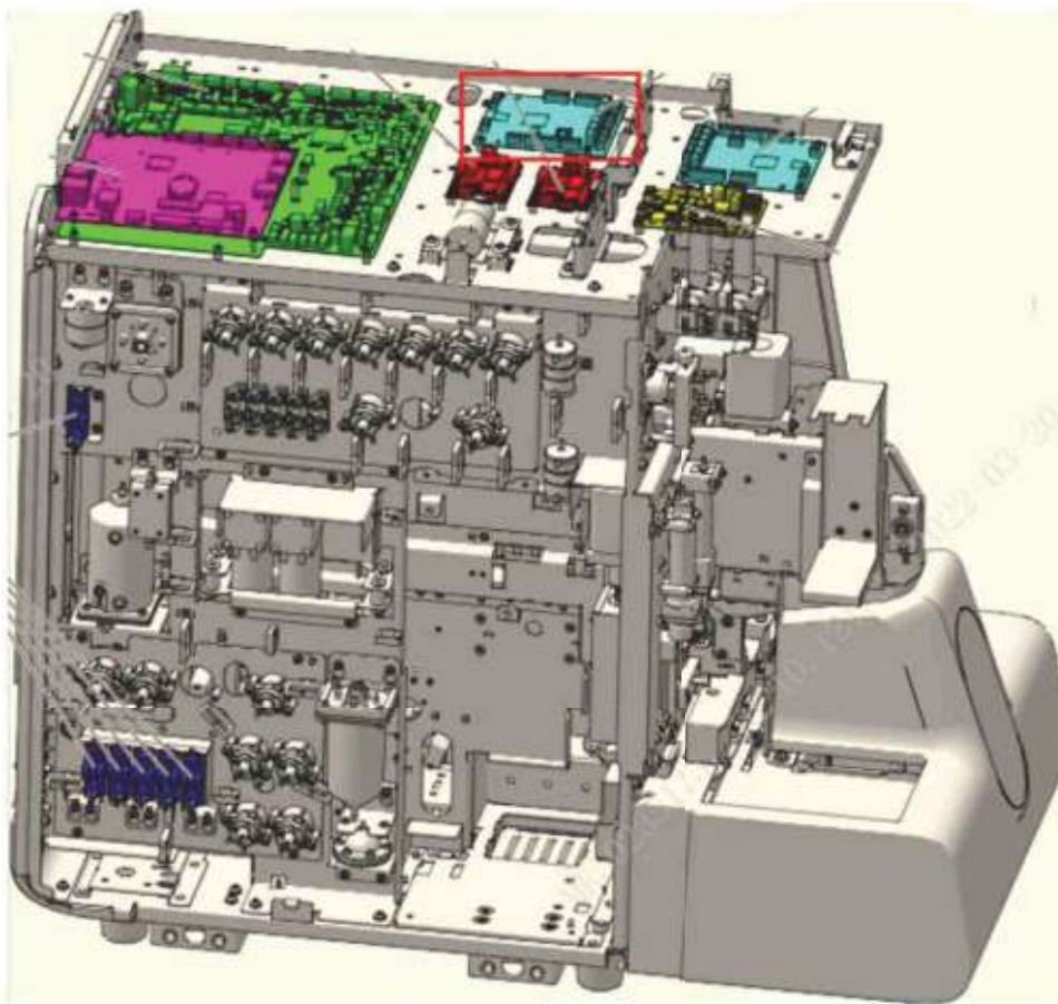
Figure7–606 Diagram of Board Position
