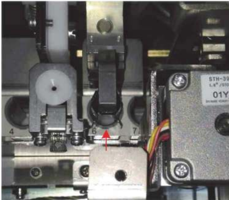
Figure7-317 Observing the Mixing Gripper Position
