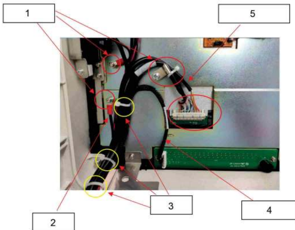
Figure7-14 Display backlight cable, indicator board cable, and grounding cable
