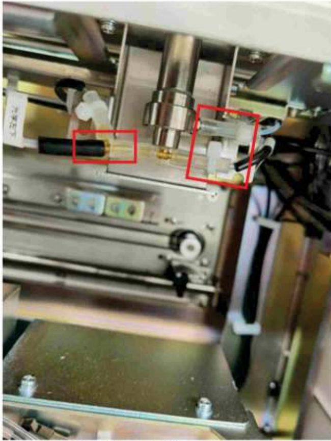
Figure7-413 Diagram of Removing the Tube of the Optical System Flow Cell
