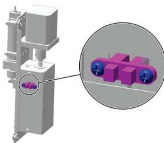
Figure7–110 Positions of the set screws of the Photoelectric Position Sensor
