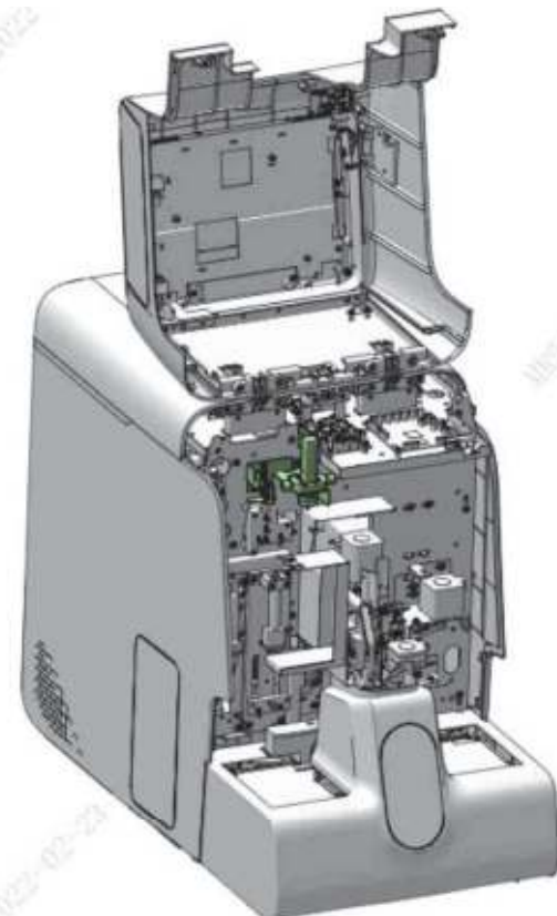
Figure7–576 Diagram B of Location of the Flyorescence Dye Pump Asm (Exclude RET)
