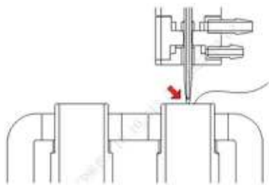
Figure7–40 Observation position of the sampling probe relative to the reaction bath
