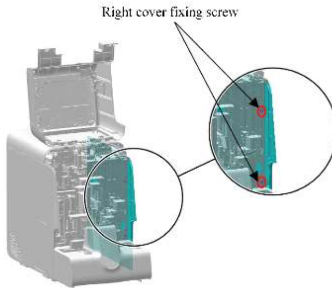
Figure7-629 Removing the right cover
