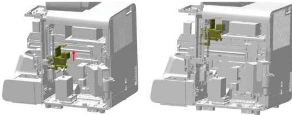
Figure7-141 Binding after lifting the mix Y-direction Assembly
