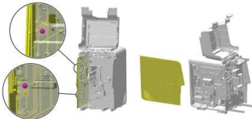
Figure7-116 Removing the left cover
