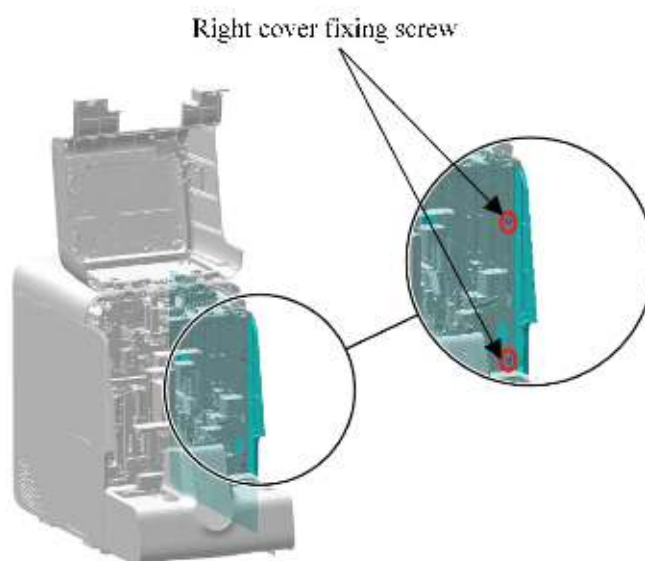
Figure7–499 Diagram of Removing the Right Cover
