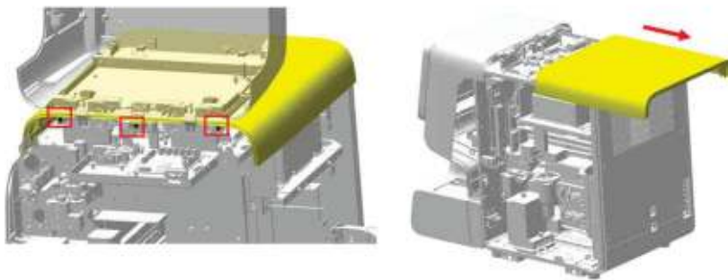
Figure7-411 Diagram of Removing the Top Cover
