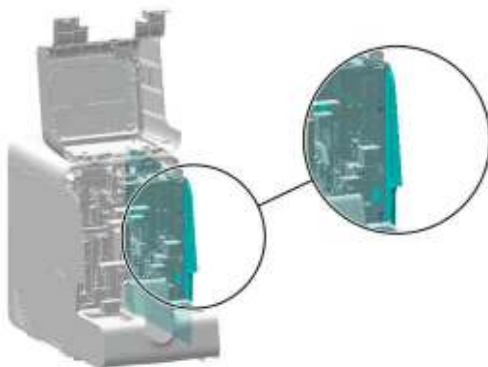
Figure7–111 Removing the right cover
