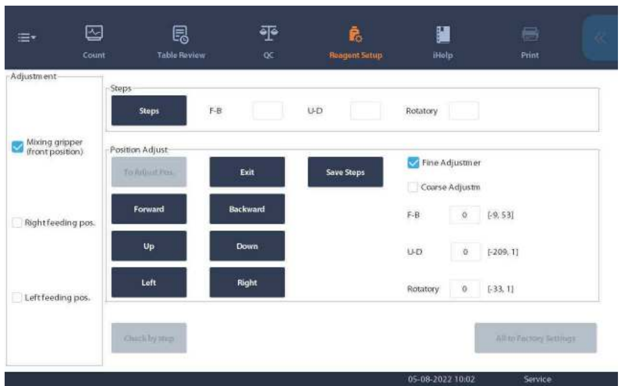
Figure7–316 Observing the Mixing Gripper Position
