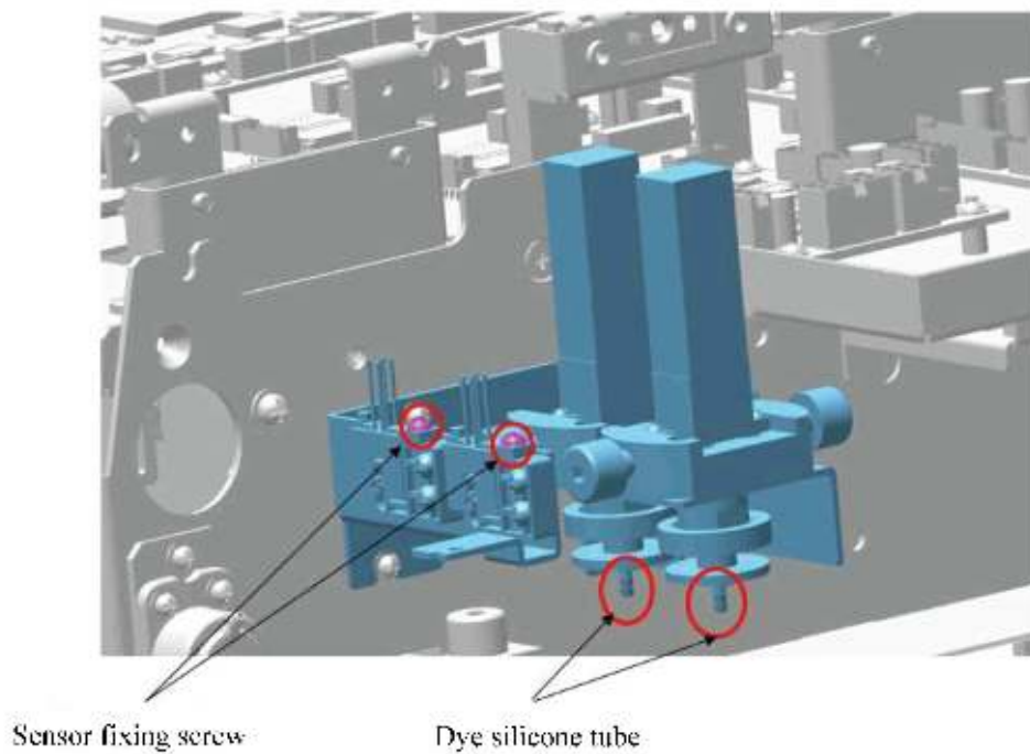
Figure7–563 Diagram of Removing the Rubber Tube of Flyorescence Dye Pump Asm (Include ERT)
