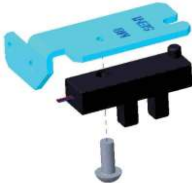
Figure7–74 Removing the Y-direction initial position sensor
