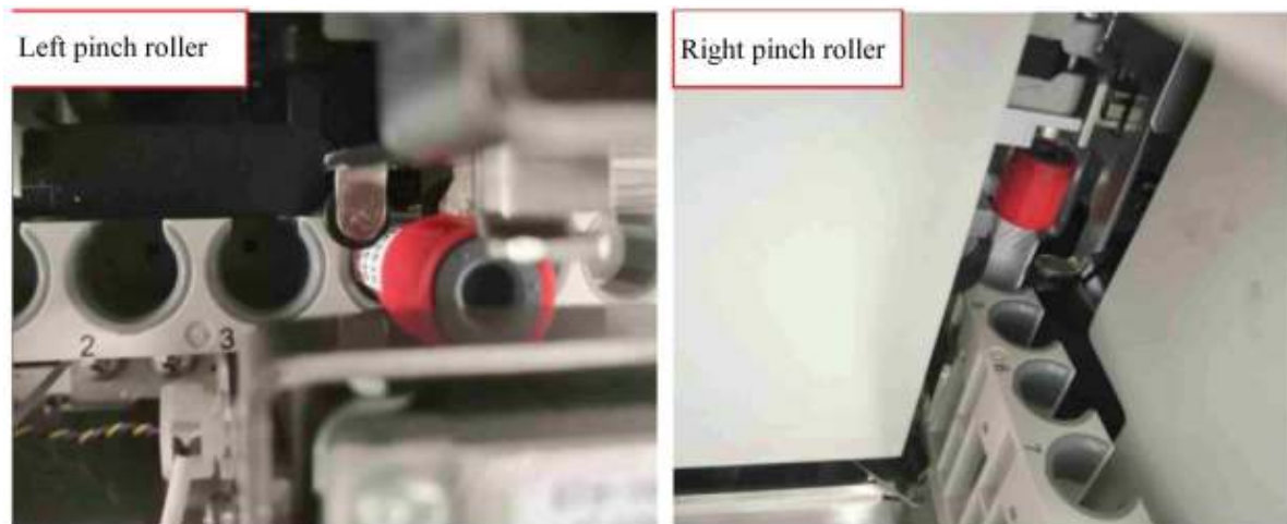
Figure3–44 Ideal Position of the Pincher Roller of the Rotatory Compressing Assembly Relative to the Tube Rack
