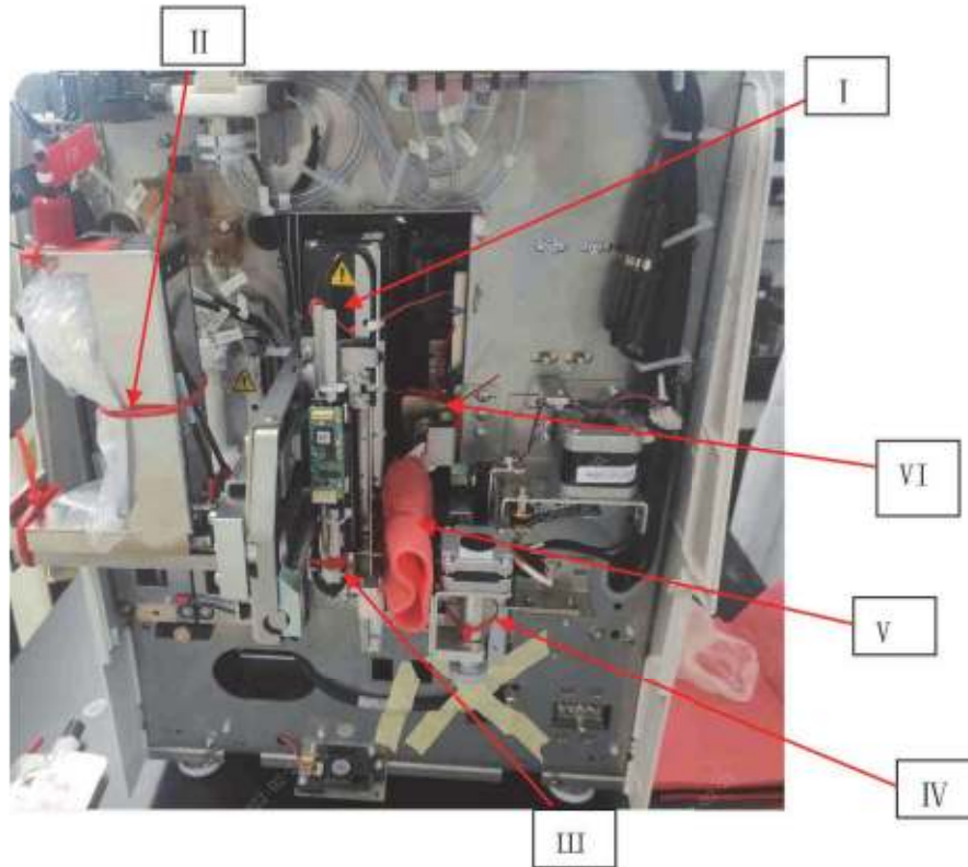
Figure9–11 Layout of wire ties
