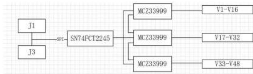
Figure7–608 Functional block diagram of valve driver board
