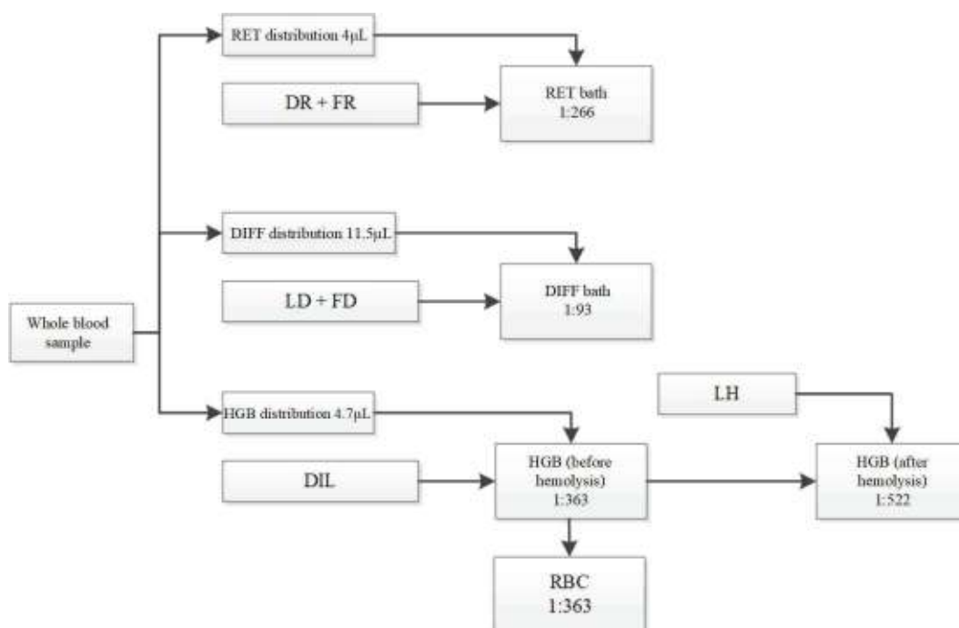
Figure2–13 WB Sample Dilution Flowchart
