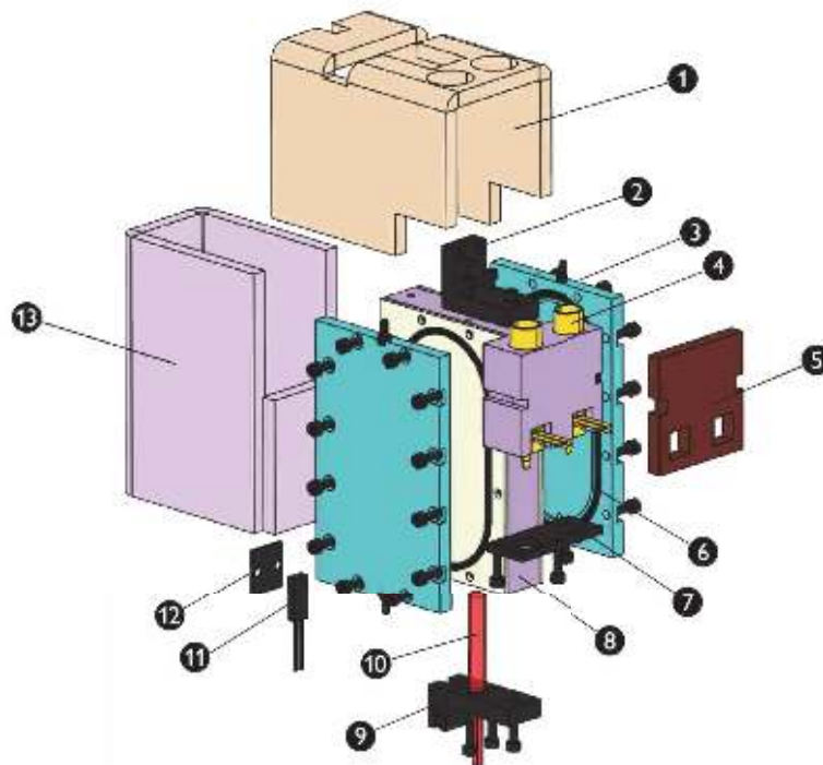
Figure2–49 Figure: Exploded View of Blood Routine Reaction Bath Assembly Structure
