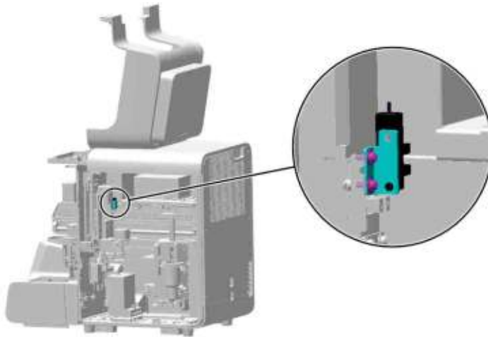
Figure7-78 Removing the sensor fixing plate
