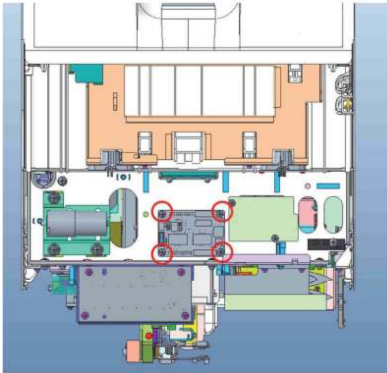
Figure7-611 Positions of screws of the valve drive board
