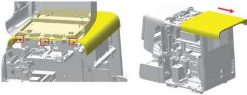
Figure7–650 Diagram of Removing the Top Cover
