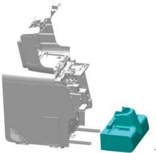
Figure7-21 Figure 2 - Removing Procedure of the Autoloader
