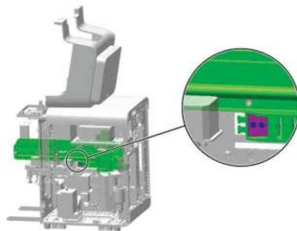
Figure7–32 Removing the end of sampling drag chain
