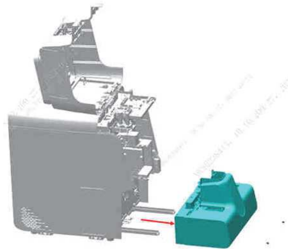
Figure7–221 Removing the 5x6 closed autoloader (FRU)
