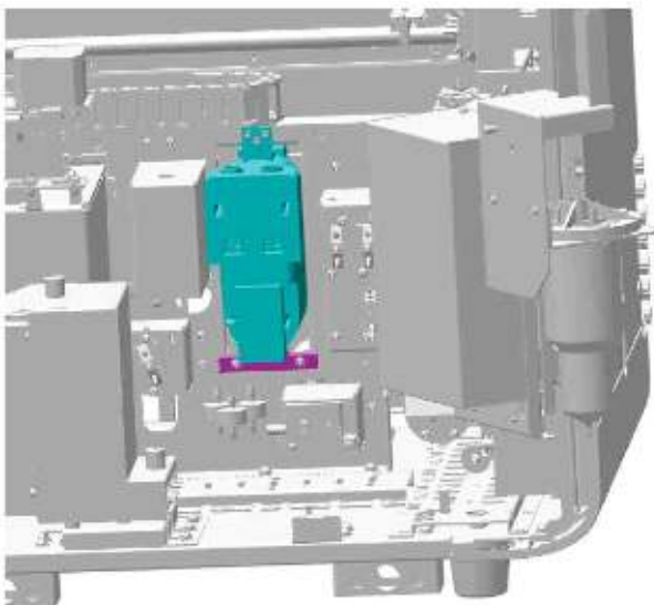
Figure7–371 Diagram of Separating the Reaction Bath Assembly from the Reaction Bath Fixing Block
