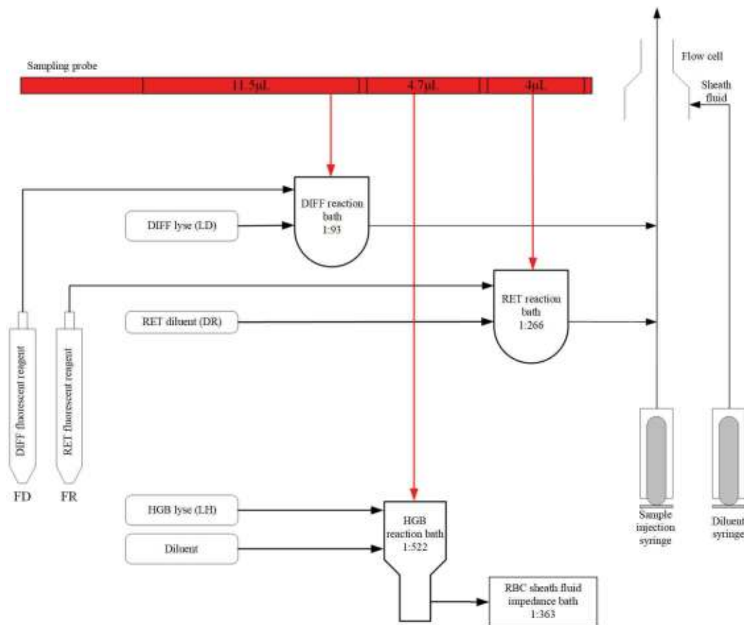
Figure2–11 Measurement Procedure of Each Channel
