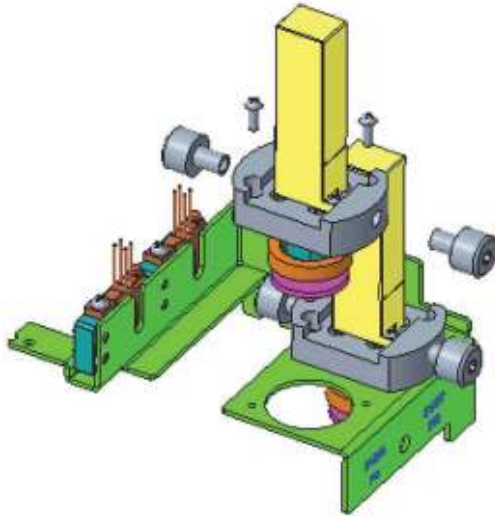
Figure7–580 Diagram of Removing 20 \mu L Metering Pump Assembly (Exclude RET)
