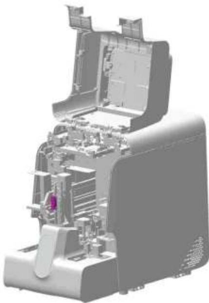
Figure7–88 Position of ESR measurement assembly
