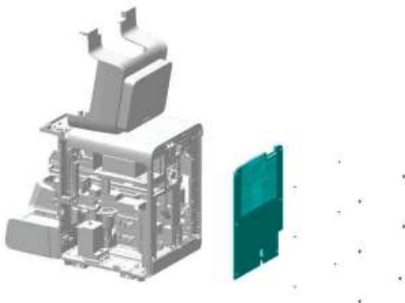
Figure7–70 Removing procedure of the rear panel
