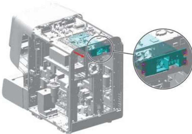
Figure7–655 Diagram of Removing the Power Supply Assembly
