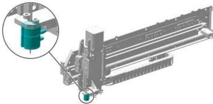
Figure7–149 Location of Probe Wipe 2 on the Sampling Assembly
