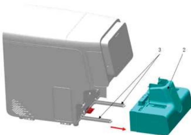
Figure7–4 Diagram 2 for Maintenance Procedure of Trumpet Assembly
