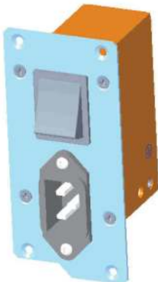
Figure7–656 Photo of Power Supply Assembly
