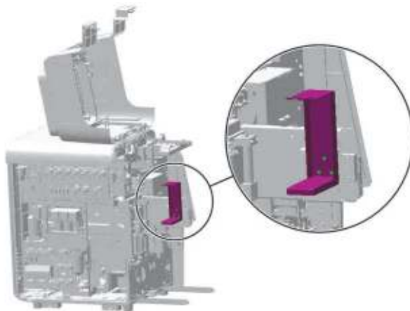
Figure7-476 Diagram of Removing the Left Cover
