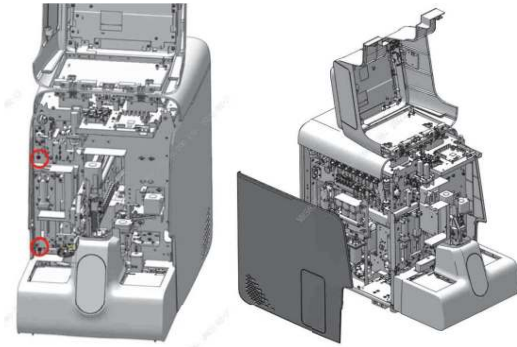
Figure7–522 Diagram A of Removing the Left Cover
