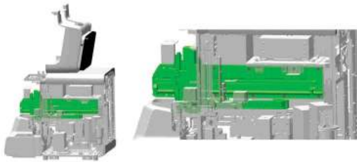
Figure7–33 Removing the sampling assembly body
