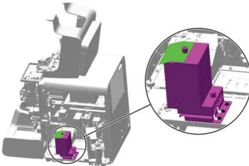
Figure7–392 Removing the shielding cover of the sheath fluid impedance assembly
