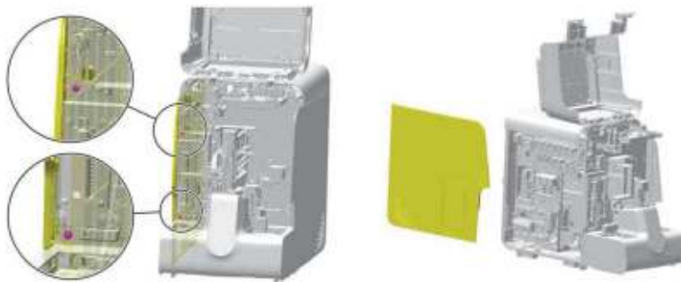
Figure7–440 Diagram of Removing the Left Cover
