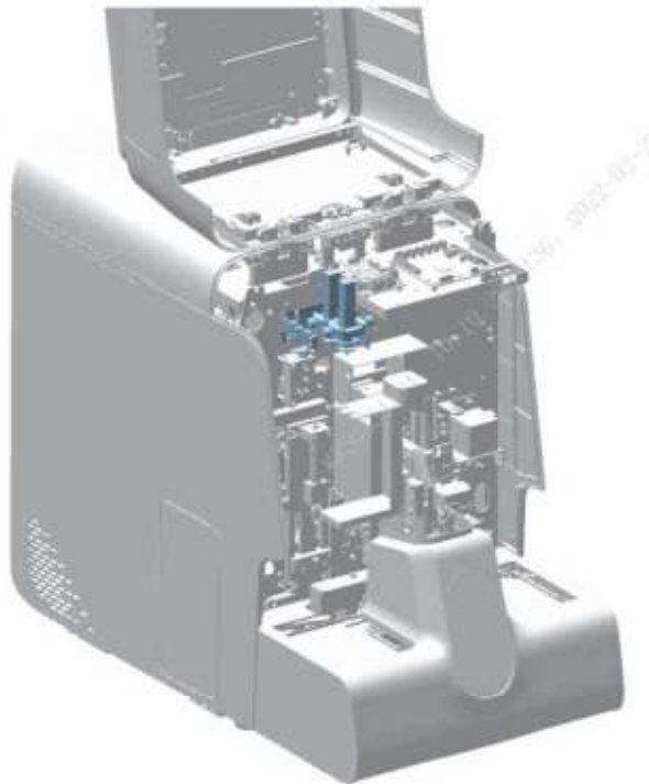
Figure7–576 Diagram B of Location of the Flyorescence Dye Pump Asm (Exclude RET)
