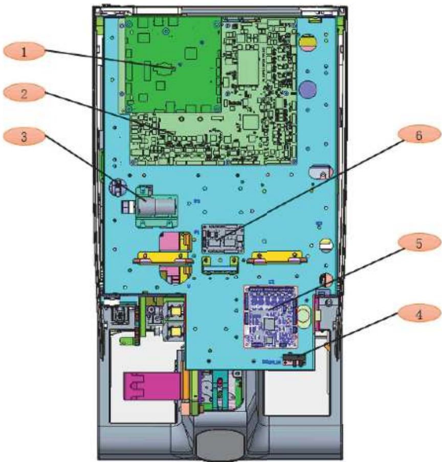
Figure2–9 Vertical View of the analyzer (Top Cover Open)
