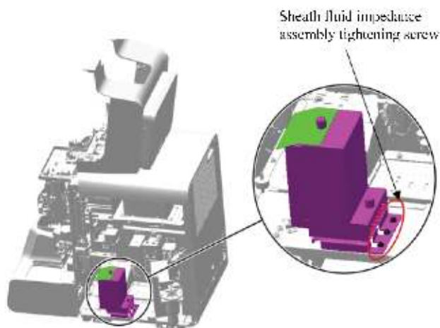
Figure7–398 Removing the shielding cover of the sheath fluid impedance assembly
