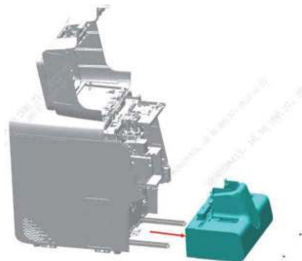
Figure7–257 Removing the autoloader assembly
