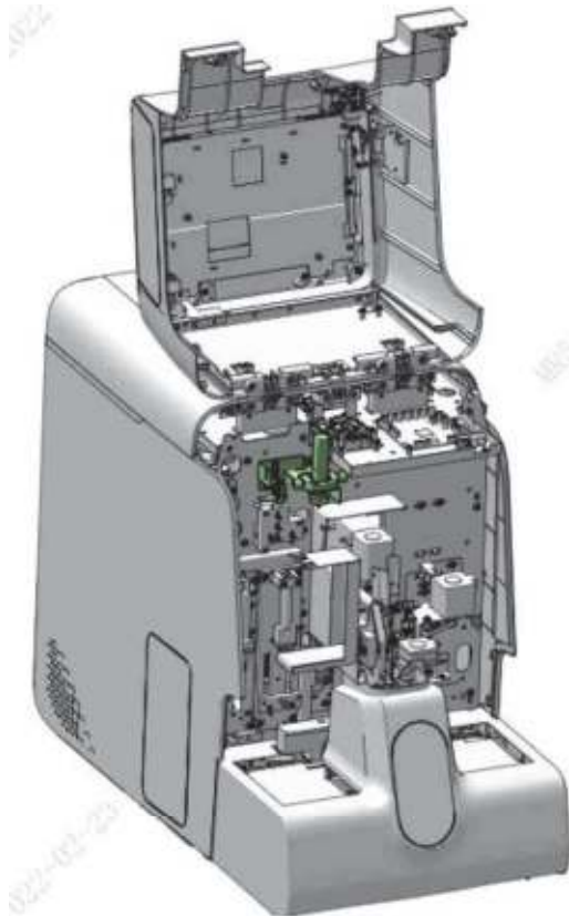
Figure7–569 Diagram of Location of the Flyorescence Dye Pump Asm (Exclude RET)
