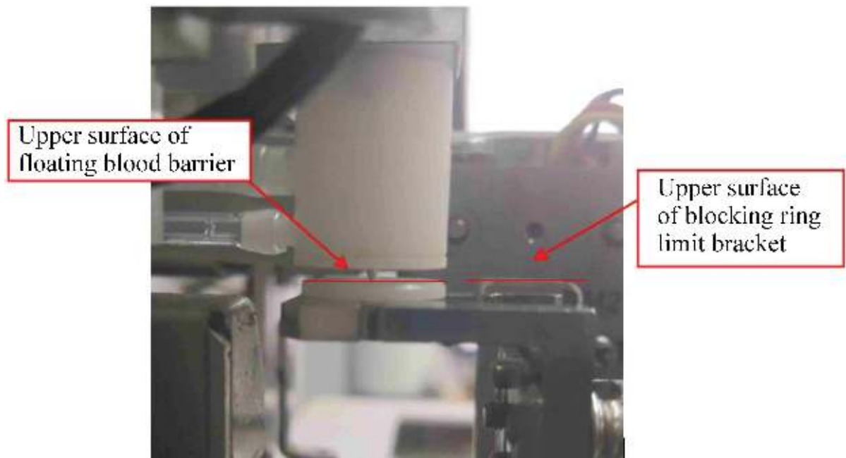
Figure3–38 Confirming the Blocking Ring Limit Bracket Position
