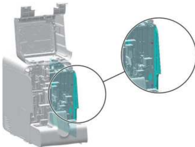
Figure7–436 Removing the right cover
