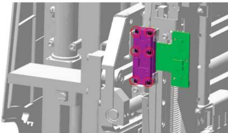
Figure7–90 Positions of the set screws of the ESR PD fixation block
