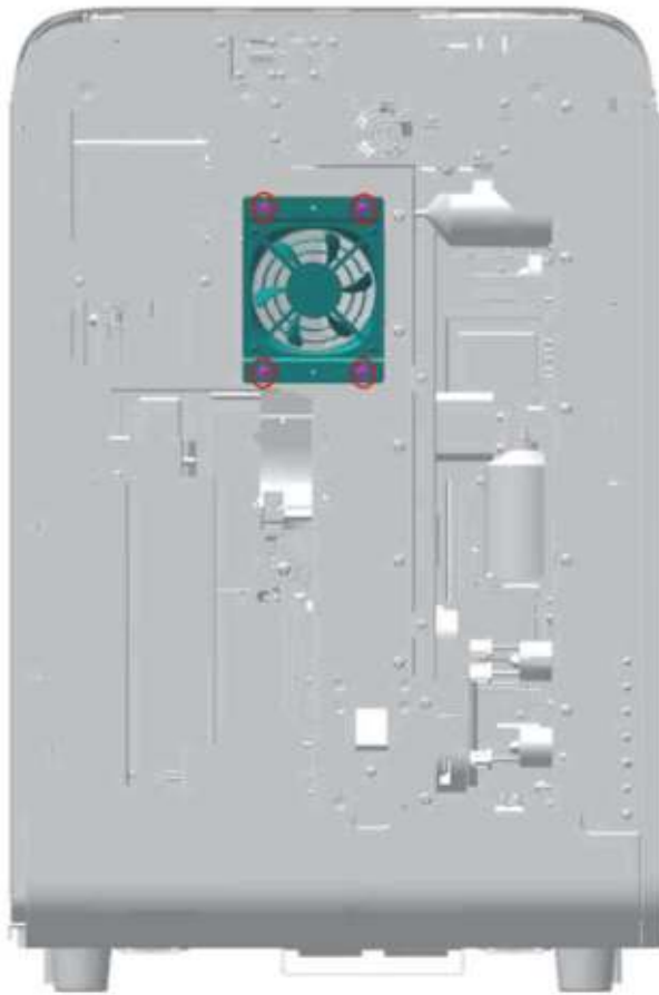
Figure7–633 Diagram of Removing the Fan Assembly
