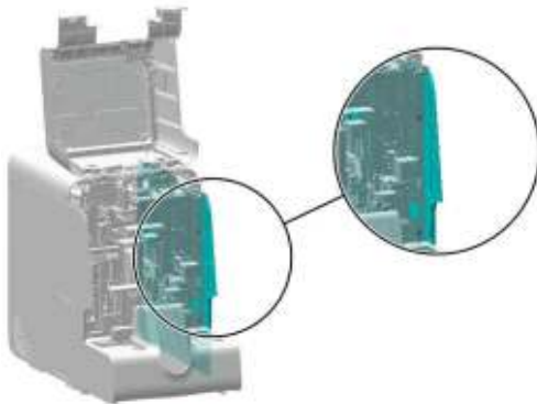
Figure7–69 Removing the right cover
