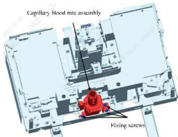
Figure7–334 Removing the capillary blood mix assembly
