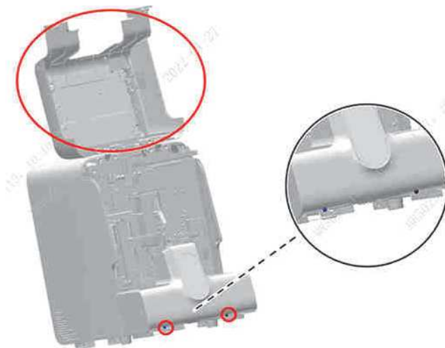
Figure7–295 Opening the front cover
