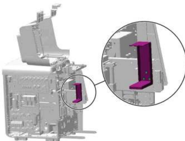
Figure7-117 Removing the dye bag support
