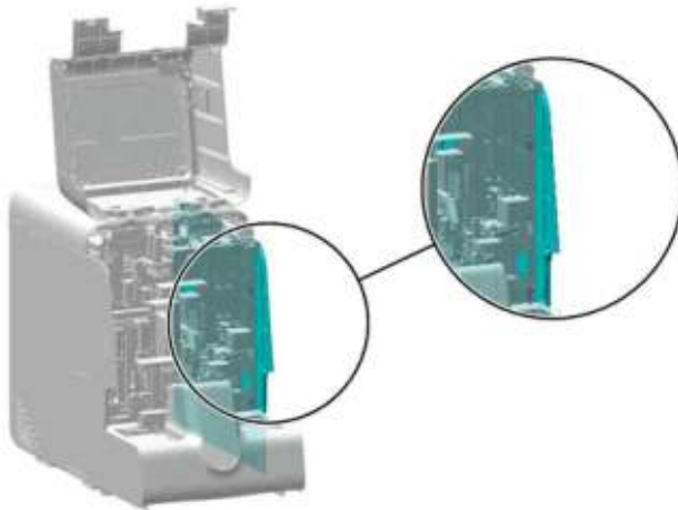
Figure7–121 Removing the right cover
