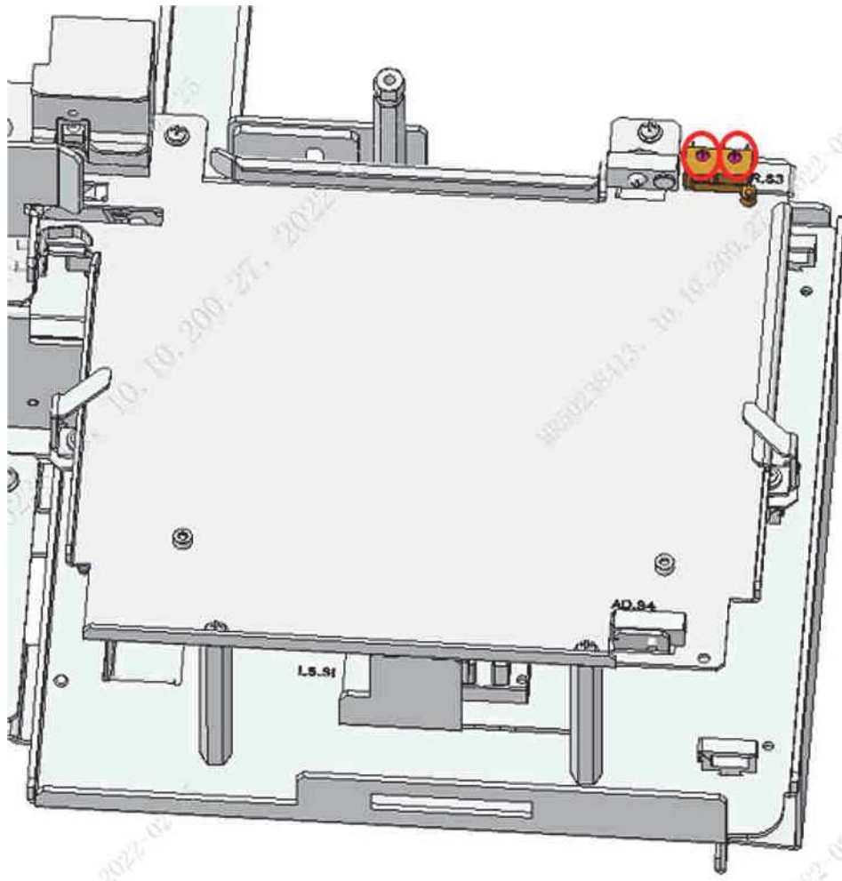
Figure7–294 Removing the SWITCH micro switch minimum DIP
