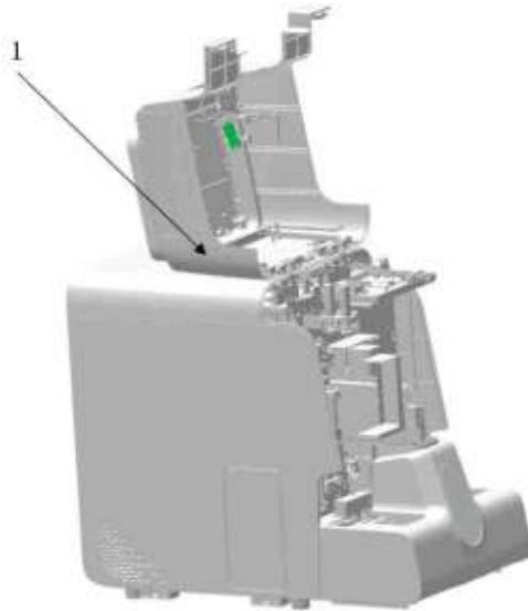
Figure7–9 Figure 2 - Maintenance Procedure of the Switch Key Board PCBA
