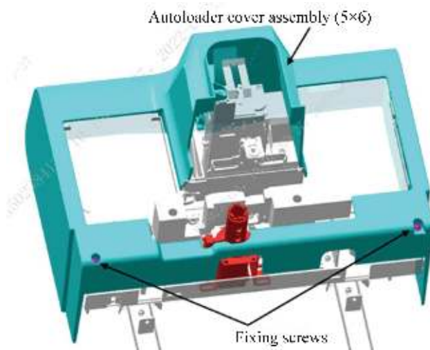
Figure7–297 Removing autoloader front cover assembly (5x6)
