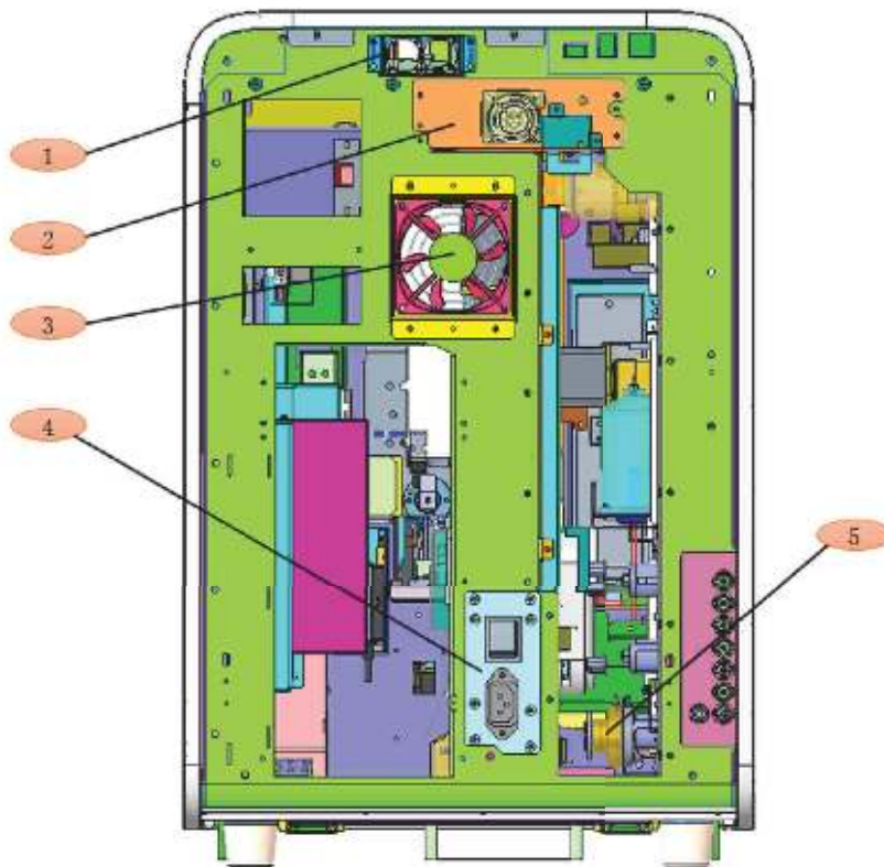
Figure2–10 Rear View of the Analyzer (Rear Cover Open)
