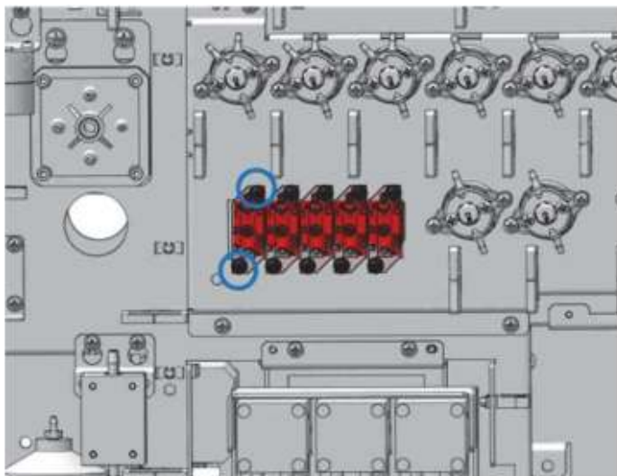
Figure7–496 Positions of the set screws of the LVM valve assembly of two-way
