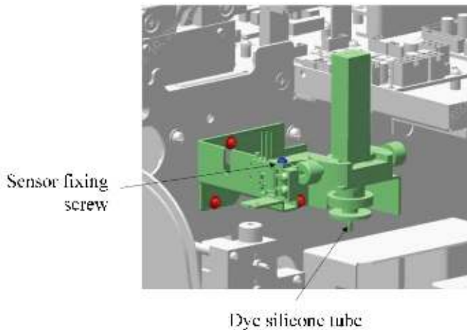
Figure7–584 Diagram of Removing the Rubber Tube of Flyorescence Dye Pump Asm (Exclude RET)
