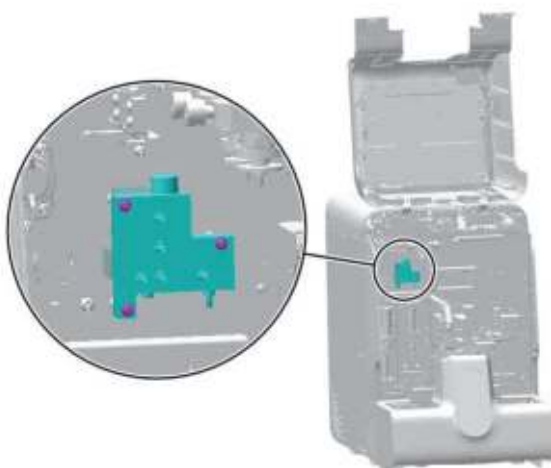
Figure7-477 Positions of the set screws of the air tank assembly
