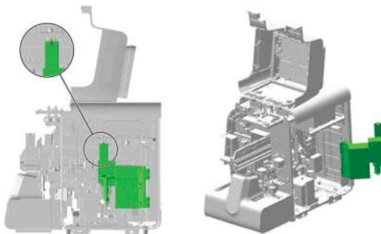
Figure7-140 Opening the right cover assembly
