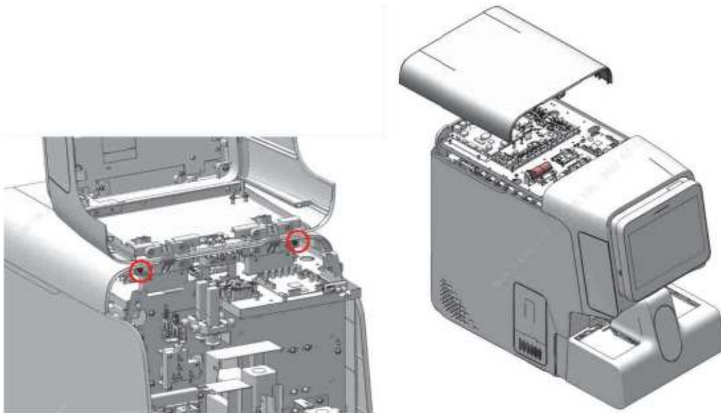
Figure7–538 Removing the covers
