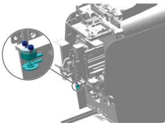
Figure7–150 Opening the front cover
