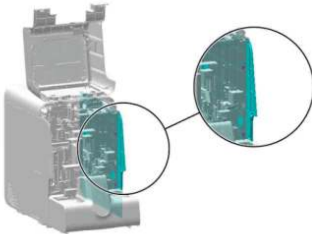
Figure7-126 Removing the right cover
