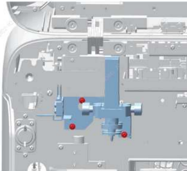
Figure7–578 Diagram A of Screw Fixing Location of the Flyorescence Dye Pump Asm (Exclude RET)
