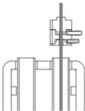
Figure7–41 Check position of the sampling probe relative to the reaction bath
