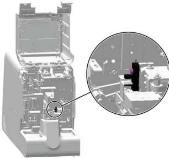
Figure7–85 Removing the sensor
