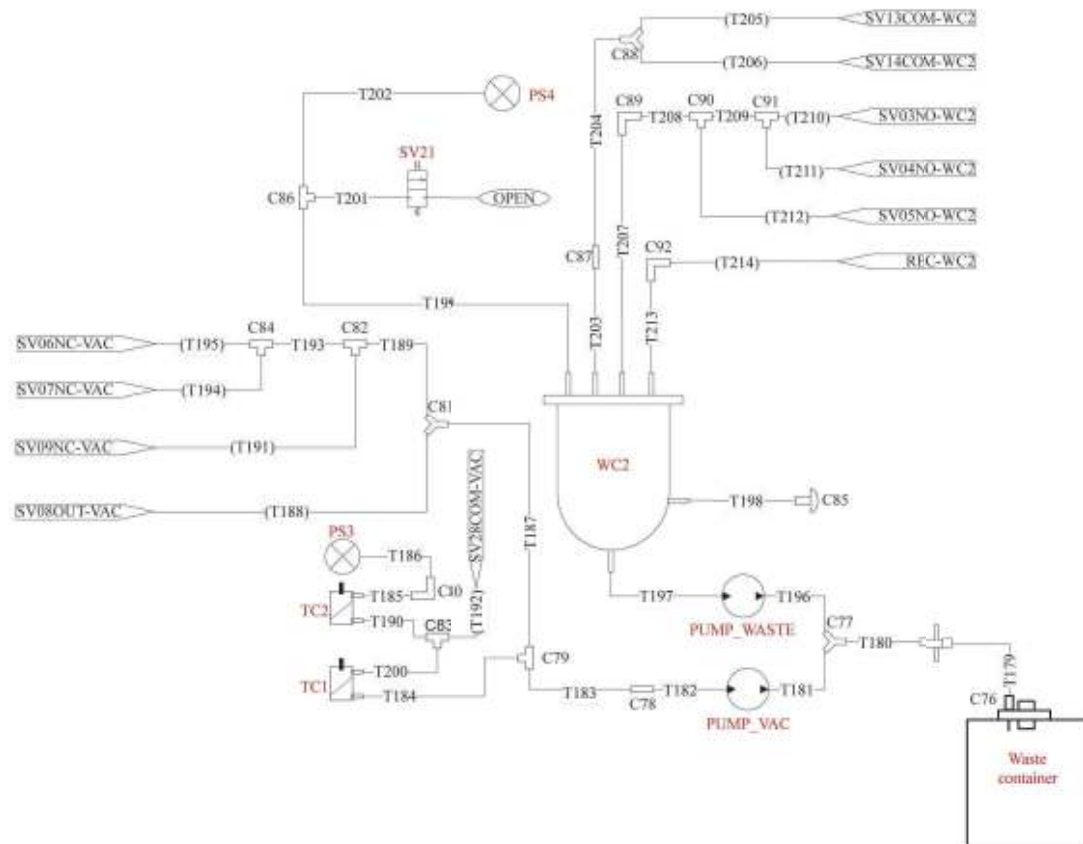
Figure2–35 HGB Measurement Waste Channel
