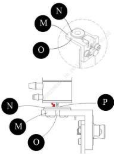
Figure7–53 Diagram of AL Aspiration Position Adjustment Acceptance Standards
