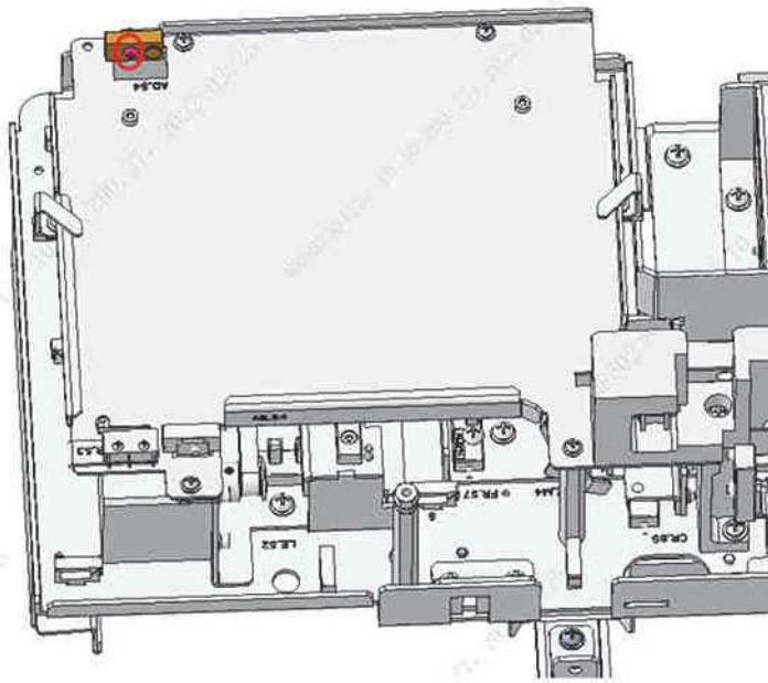
Figure7–285 Removing the PHOTOELEC detector 900nm 400mm conn
