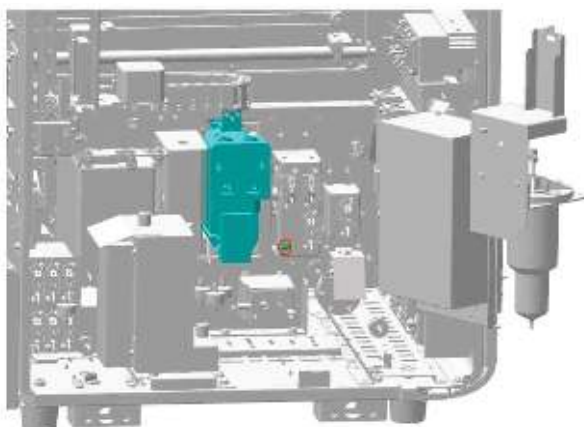
Figure7-369 Diagram of Removing the Grounding Screws of Reaction Bath Assembly
