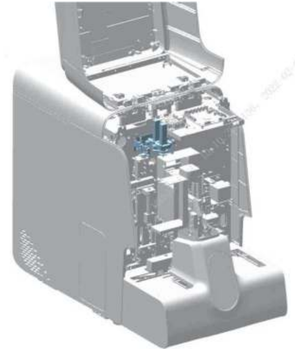
Figure7–568 Diagram A for Location of Flyorescence Dye Pump Assembly (Include RET)
