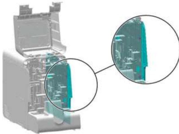
Figure7-131 Removing the right cover
