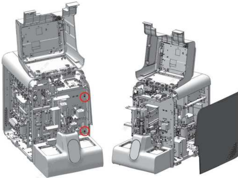
Figure7–505 Removing the covers
