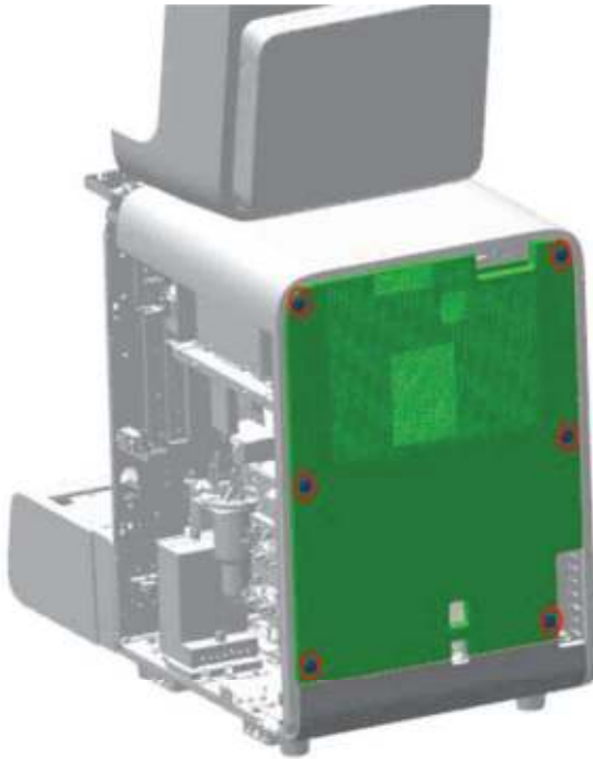
Figure7-659 Diagram B of Removing the Rear Cover Fastening Screws
