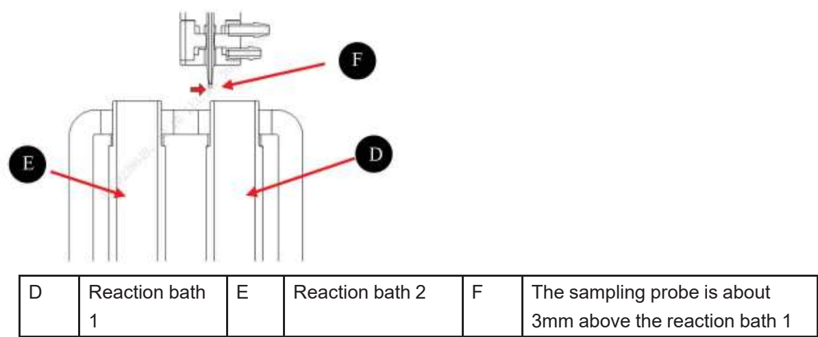
Figure7–38 Sampling probe To Default Adjust Pos. of reaction bath
