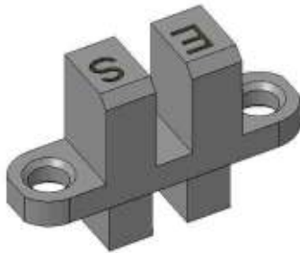
Figure7–104 Photo of Location of Photoelectric Position Sensor (SEN7) in Mix Assembly
