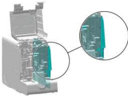
Figure7-410 Removing the right cover
