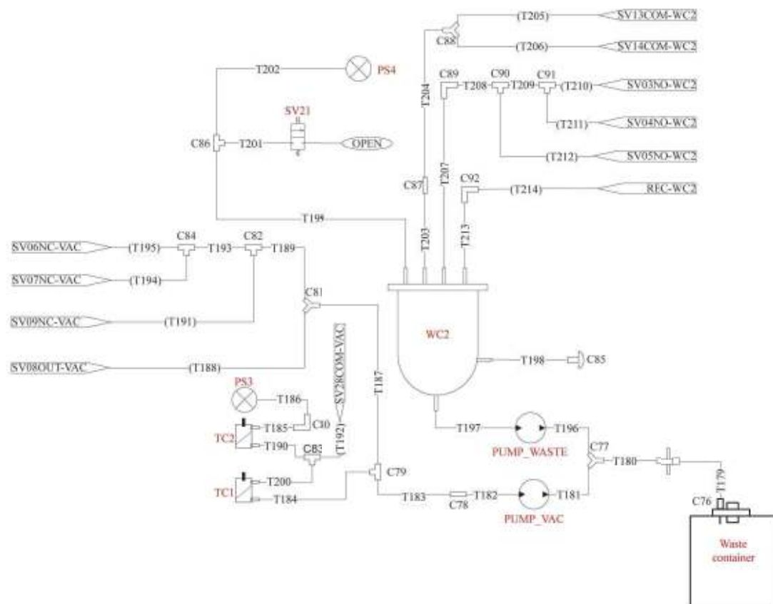
Figure2–37 RBC Measurement Waste Channel
