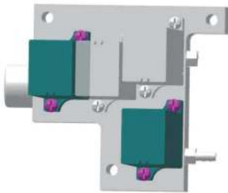
Figure7–492 Diagram of Removing the Two LVM Valve Assembly of two-way
