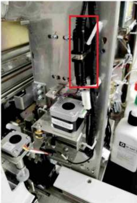
Figure7–186 Removing the scanner wire
