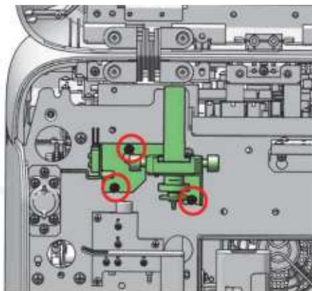
Figure7–585 Diagram of Screw Fixing Location of the Flyorescence Dye Pump Asm (Exclude RET)
