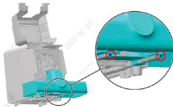
Figure7–345 Opening the front cover
