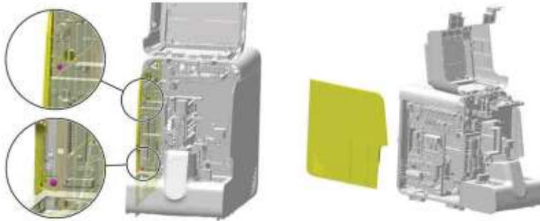
Figure7–420 Diagram of Removing the Left Cover
