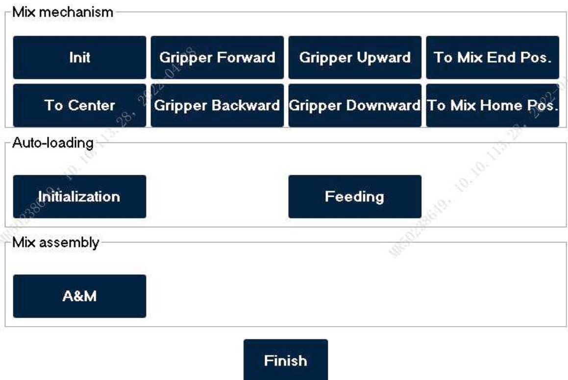
Figure7–357 Observing the Mixing Gripper Position
