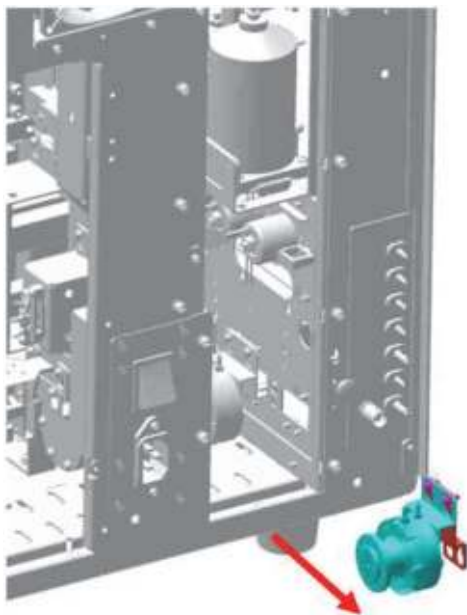
Figure7–471 Removing the metering pump assembly from the back
