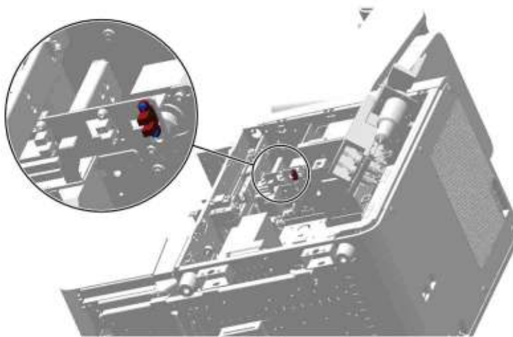
Figure7–125 Positions of the set screws of the photoelectric position sensor (SEN4)
