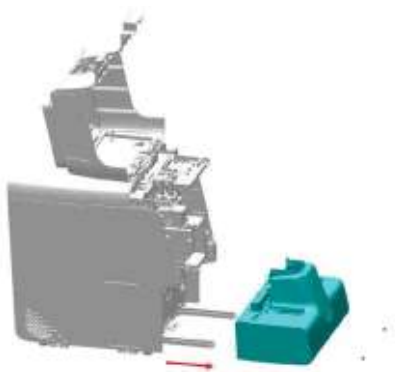
Figure7-177 Figure 2 - Removing the autoloader
