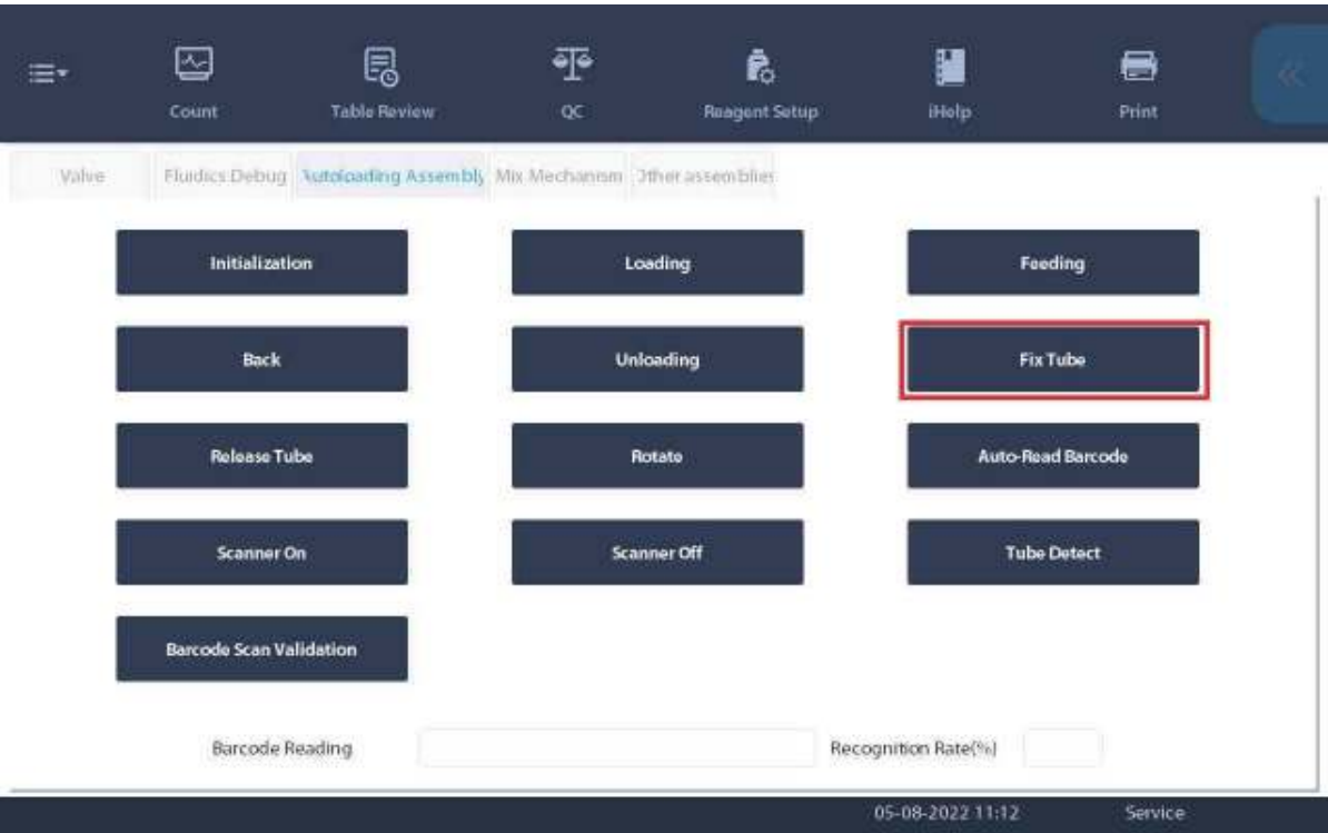
Figure7–241 Autoloader Assembly Self-test Interface
