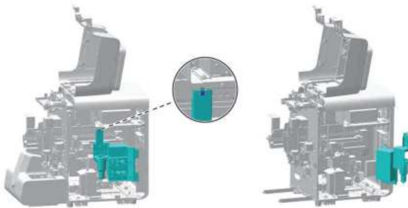
Figure7–500 Opening the right cover assembly
