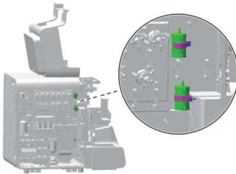
Figure7–441 Positions of the set screws of the isolation chamber
