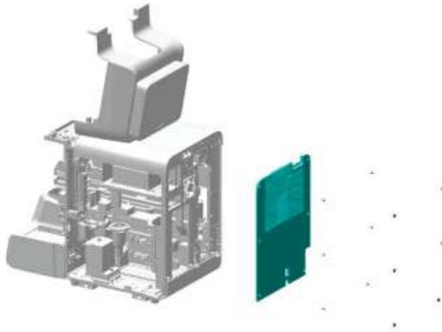
Figure7–23 Removing procedure of the rear panel
