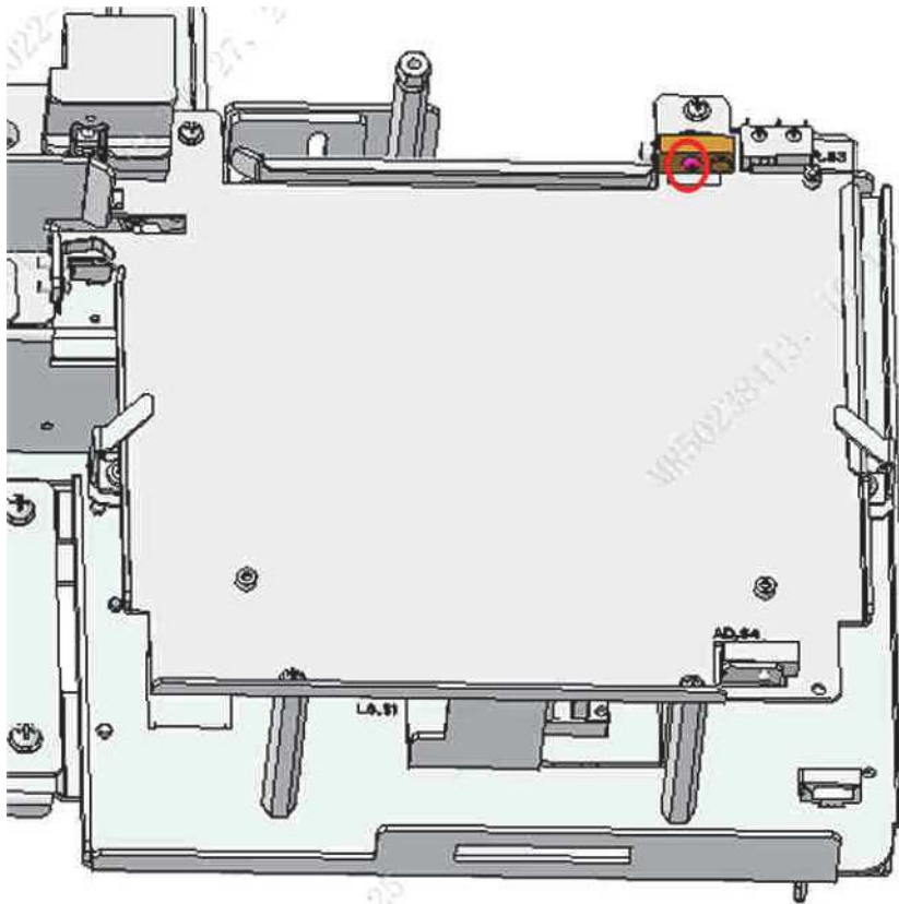
Figure7–268 Removing the PHOTOELEC emitter 940nm 400mm conn
