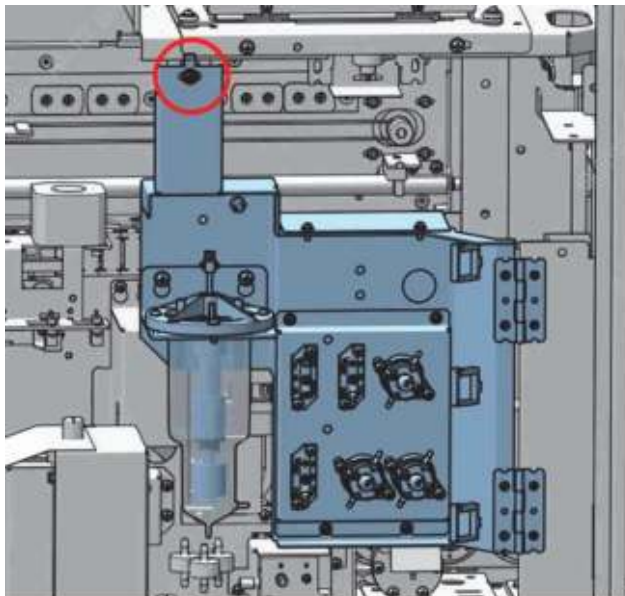
Figure7-484 Diagram A of Location of the Right Hinge Fixing Screw
