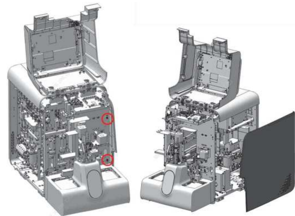
Figure7-494 Diagram B of Removing the Right Cover
