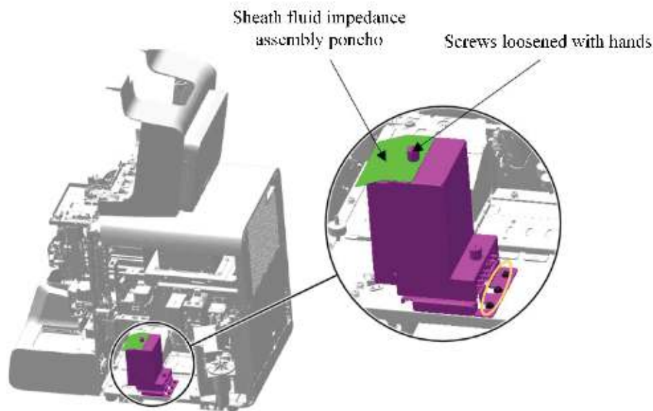
Figure7–375 Diagram of Removing the Sheath Fluid Impedance Assembly (FRU)
