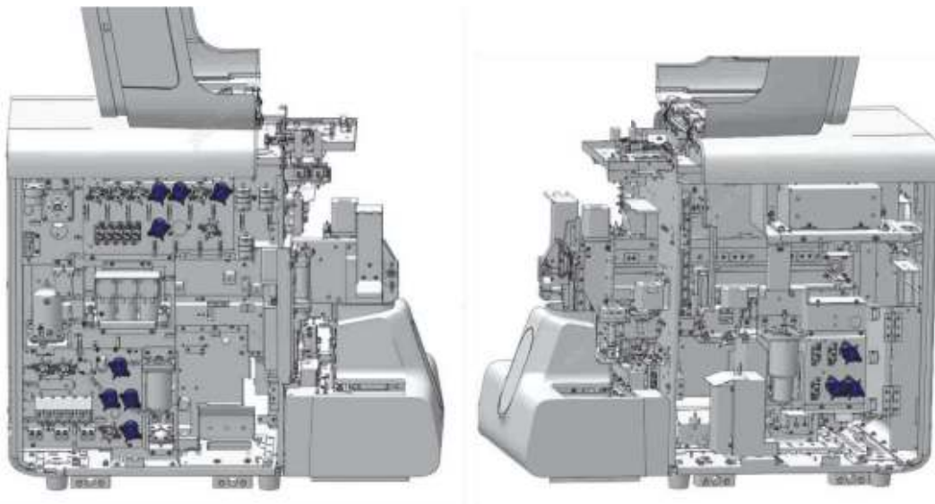
Figure7–524 Diagram C of Location of Two-way Valve (PEIZH)
