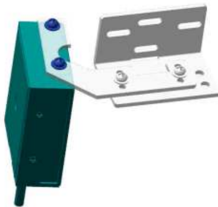
Figure7–187 Removing the scanner from the scanner assembly
