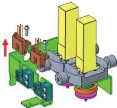
Figure7–573 Diagram of Removing the Transmissive Sensor (Exclude RET)
