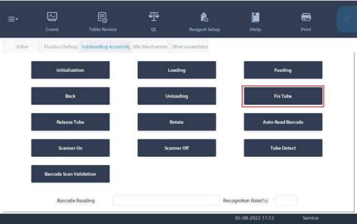
Figure7–310 Autoloader Assembly Self-test Interface
