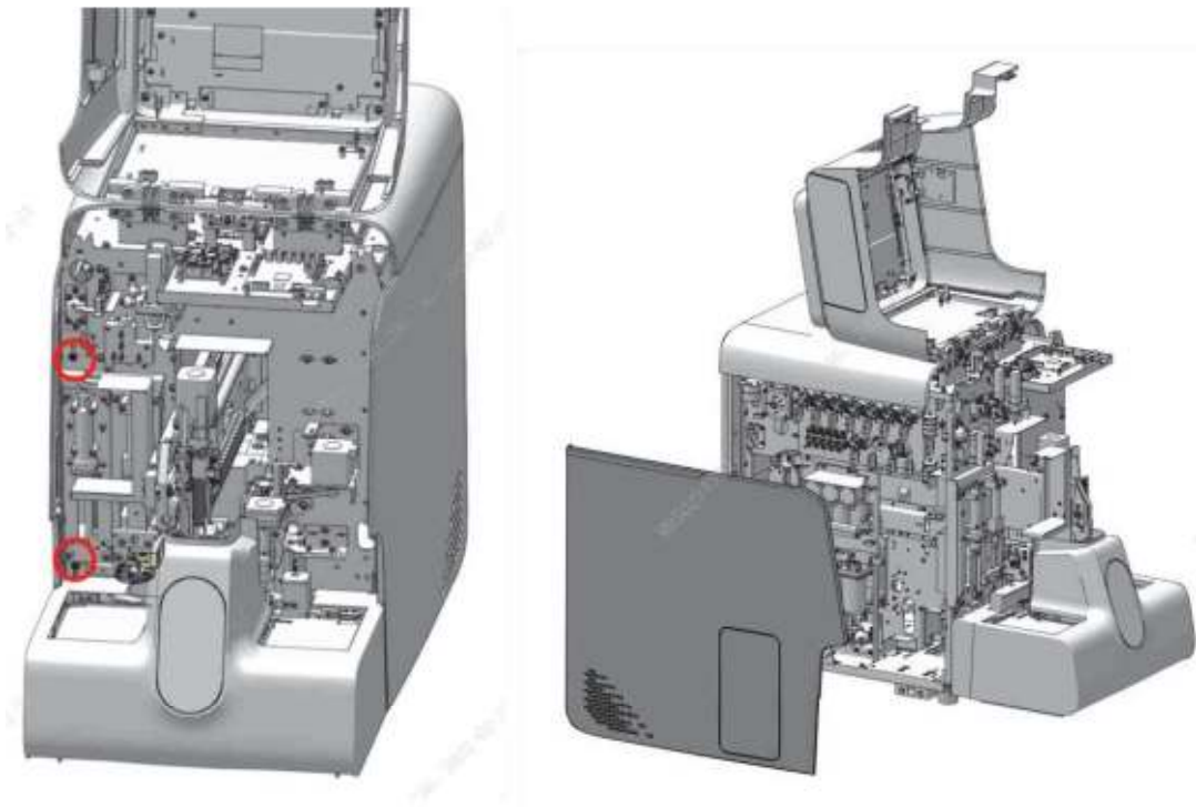
Figure7–517 Removing the covers
