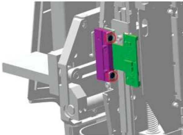
Figure7–91 Positions of the set screws of the ESR LED fixation block
