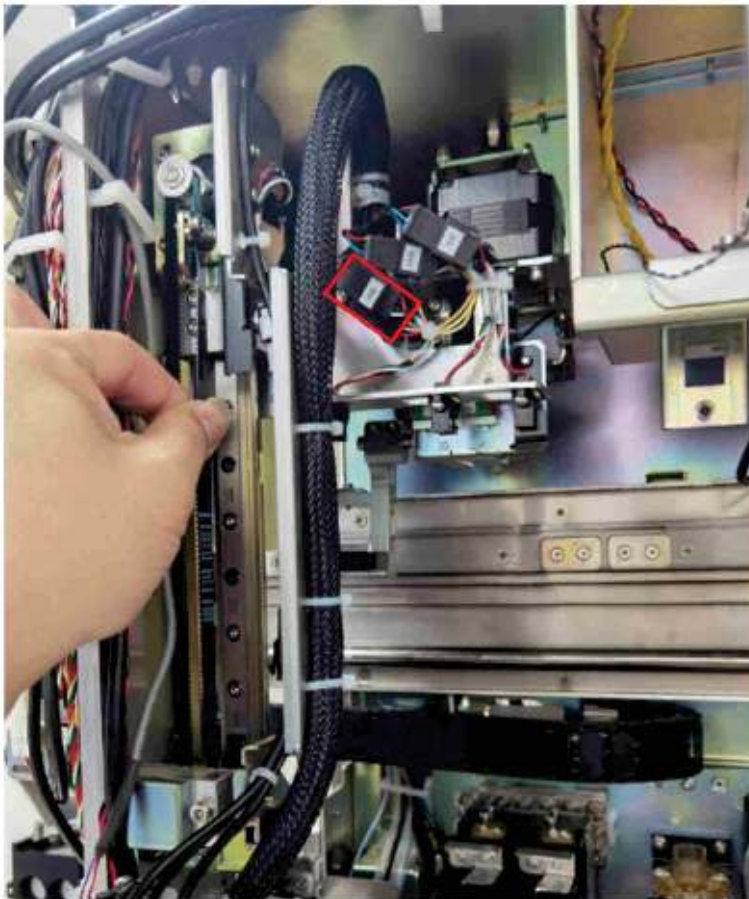
Figure7-129 Removing the photoelectric position sensor (SEN5) wire
