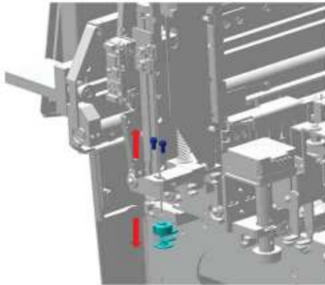
Figure7–155 Removing the probe wipe (closed-sampling)
