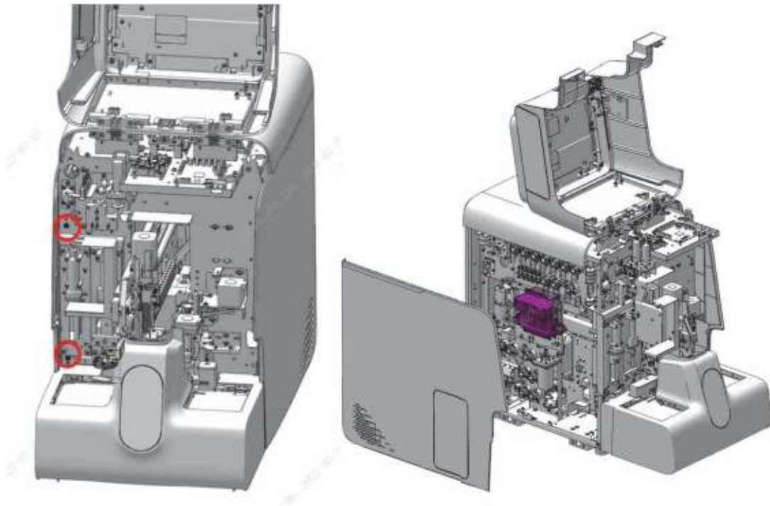
Figure7–541 Removing the covers
