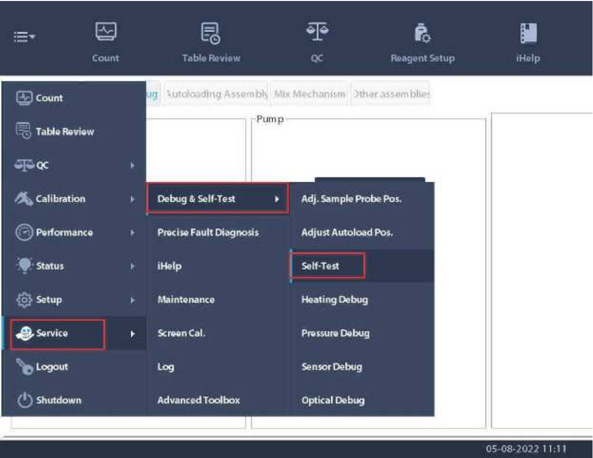
Figure7–452 Self-test screen entrance
