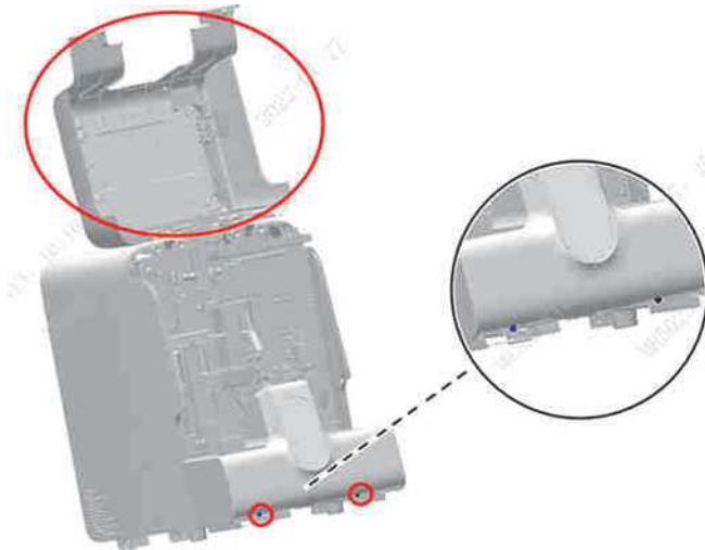
Figure7–331 Opening the front cover
