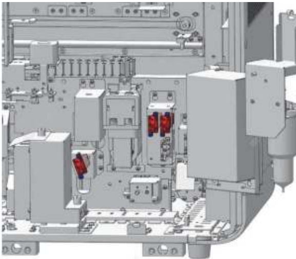
Figure7–507 Diagram B for Location of LVM Valve Assembly of two-way
