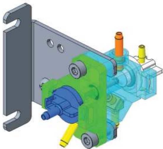
Figure7–379 Photo of sheath fluid count bath assembly
