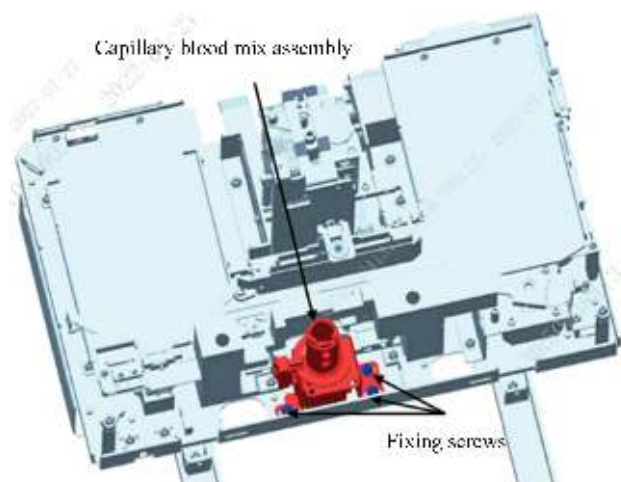
Figure7–223 Removing the capillary blood mix assembly
