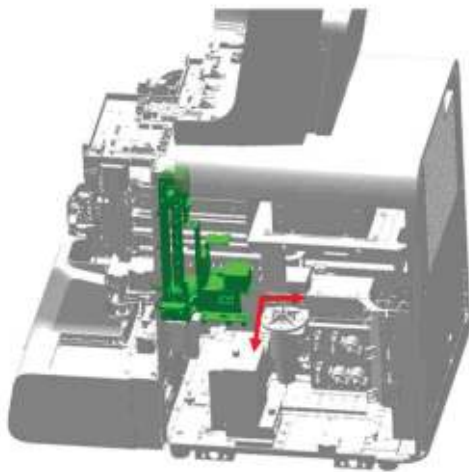
Figure7–167 Figure 2 - Removing the mix assembly
