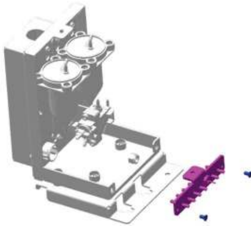
Figure7–384 Removing the connector mounting plate
