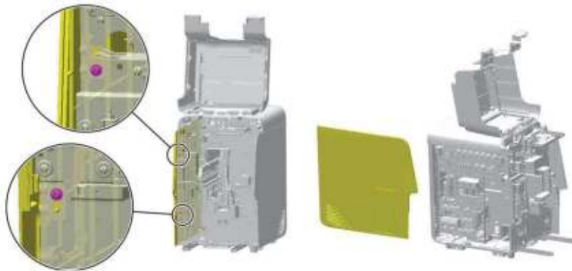
Figure7-444 Removing the left cover
