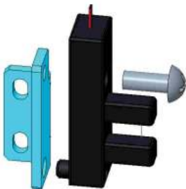
Figure7-79 Removing the detecting Sensor
