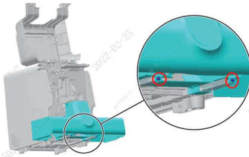
Figure7–216 Opening the front cover
