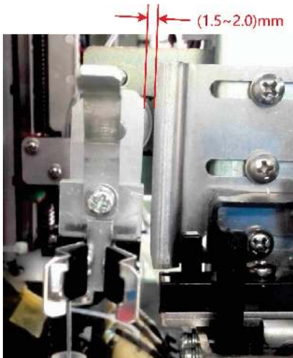
Figure7–319 Distance Requirements between the Mixing Gripper and Anti-Collision Bock
