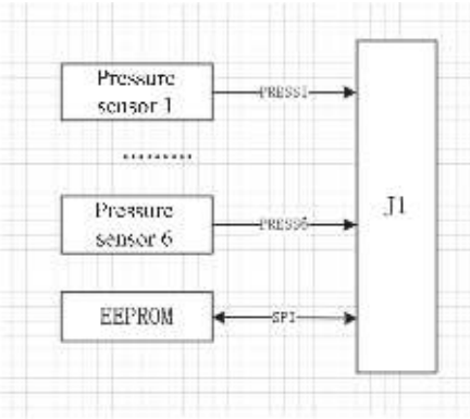
Figure7–596 Functional block diagram of the board
