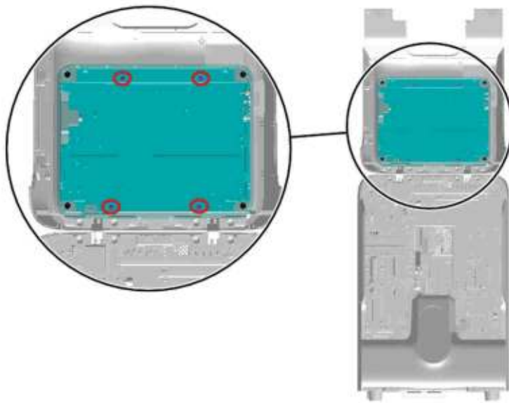
Figure7–16 Positions of the set screws of the screen cable cover
