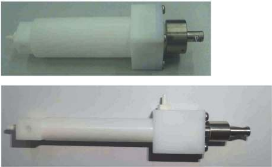
Figure2–18 Diluent syringe (upper) and sample injection syringe (lower)
