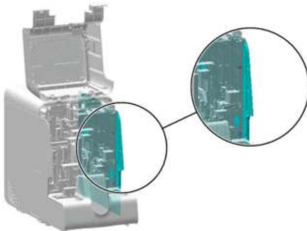
Figure7-135 Removing the right cover
