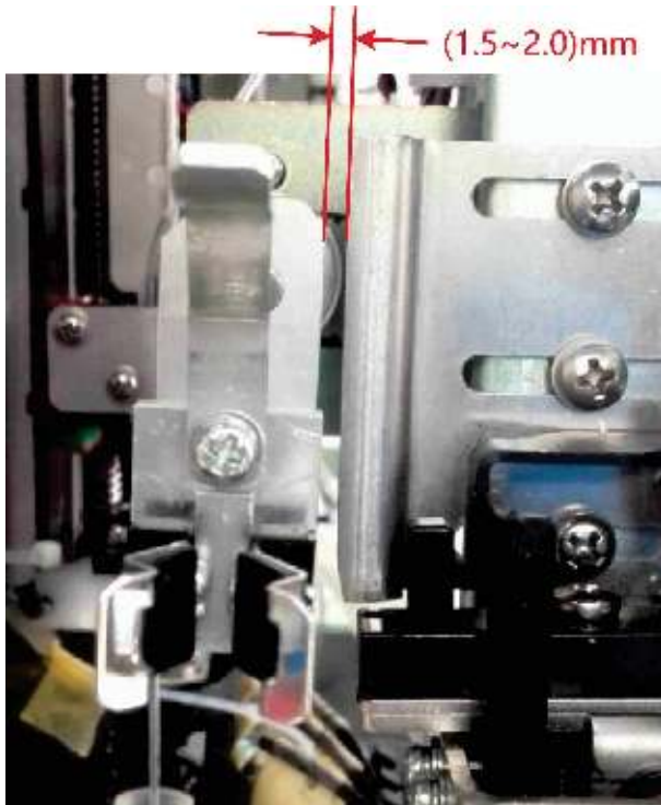
Figure7-361 Distance Requirements between the Mixing Gripper and Anti-Collision Bock
