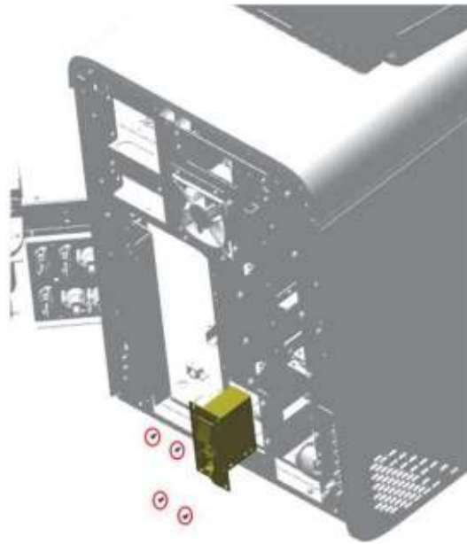
Figure7–666 Diagram of Removing the Power Switch Assembly
