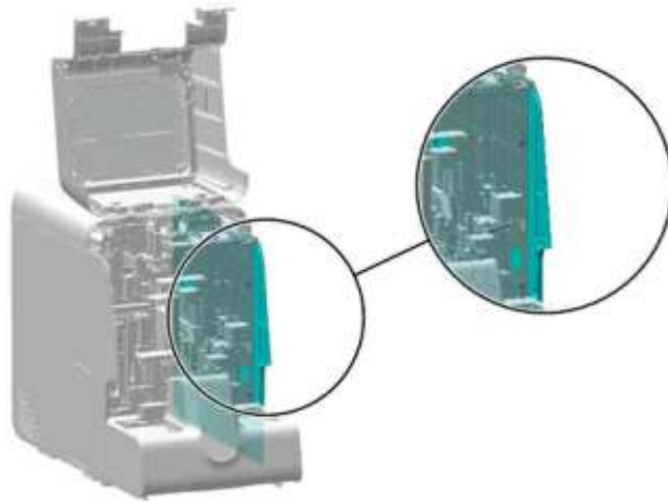
Figure7-139 Removing the right cover
