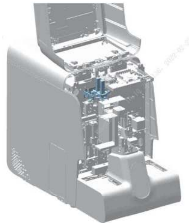
Figure7-562 Diagram of Removing the Flyorescence Dye Pump Assembly (Include RET)
