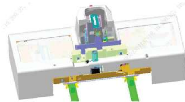
Figure7–302 Diagram of Location of Autoloader, Closed-Sampling Model (10x5) (Including Capillary Blood Mixing) in the Main Unit
