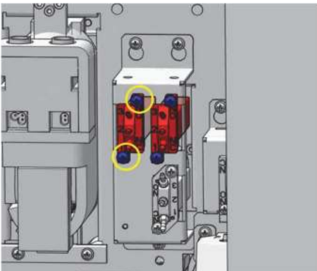
Figure7–508 Diagram for Fixing Screws of LVM Valve Assembly of two-way
