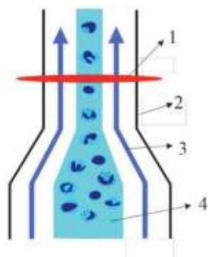
Figure2–42 Laser Facula of Flow Cell
