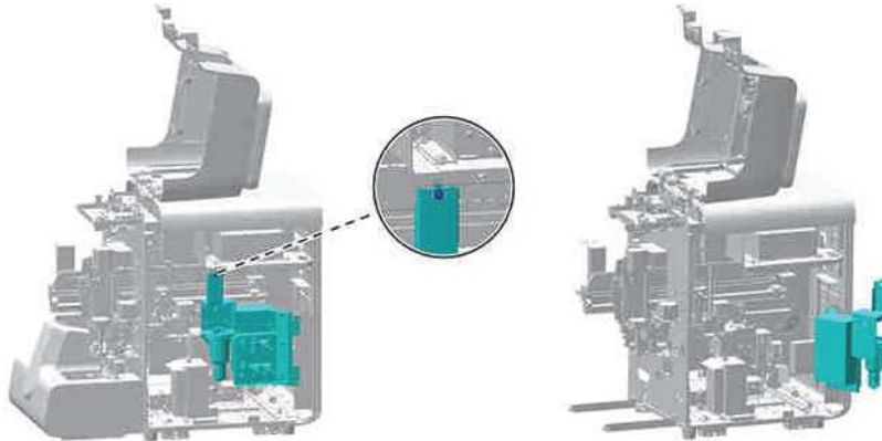
Figure7–559 Opening the right cover assembly
