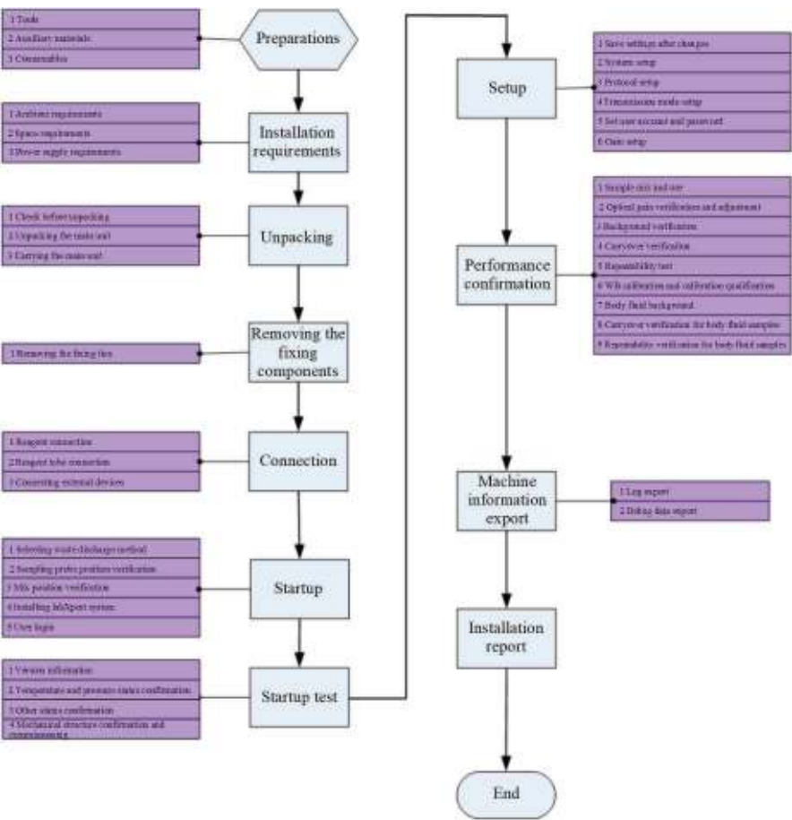
Figure3–1 Installation Flowchart
