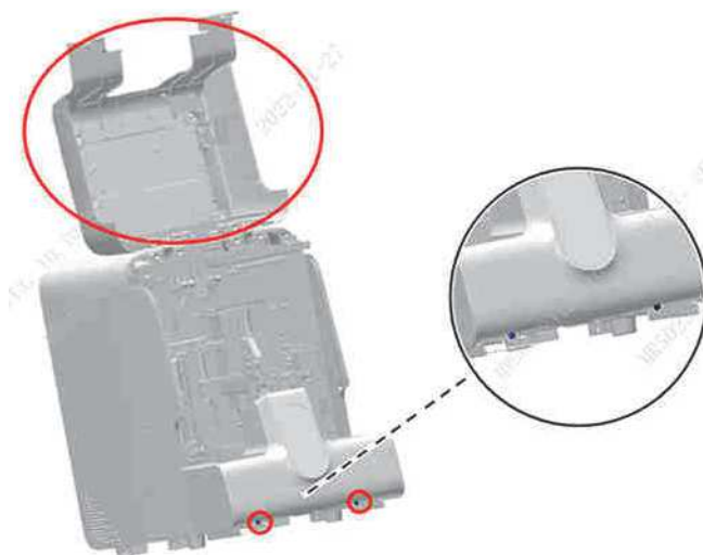
Figure7–269 Opening the front cover
