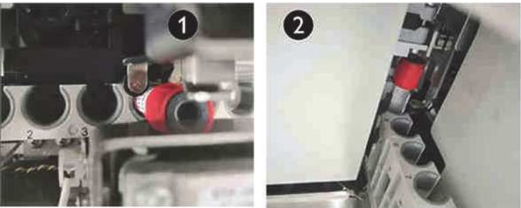
Figure7–200 Ideal Position of the Pincher Roller of the Rotatory Compressing Assembly Relative to the Tube Rack
