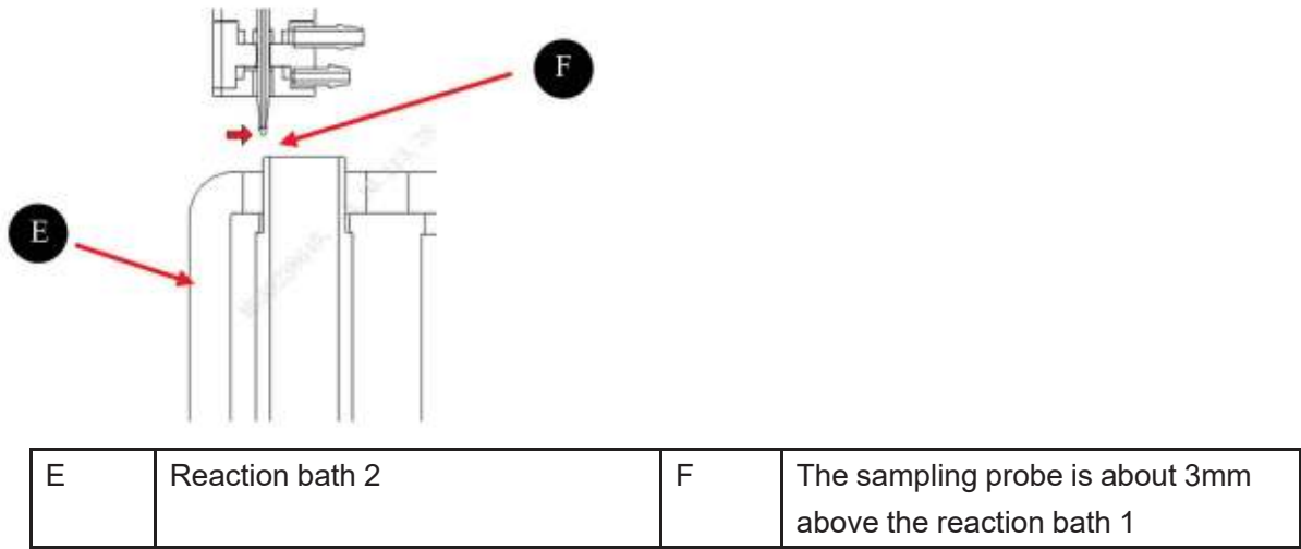
Figure7–43 Sampling probe To Default Adjust Pos. of reaction bath
