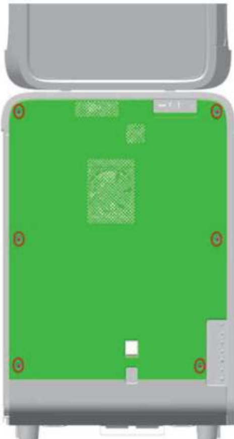
Figure7-659 Diagram B of Removing the Rear Cover Fastening Screws
