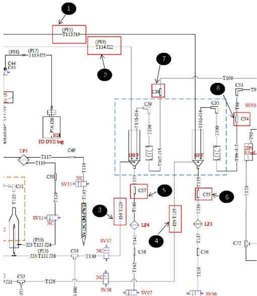
Figure7-368 Diagram of Reaction Bath Assembly Pipeline
