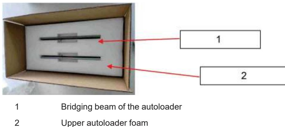
Figure3–9 Taking Out the Bridging Beam of the Autoloader
