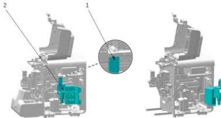
Figure7–25 Opening the right cover assembly
