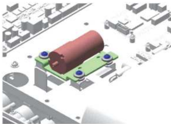
Figure7–539 Positions of the set screws of the air pump
