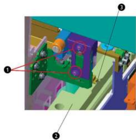
Figure7–162 Front/Rear Position Adjustment of the Hold Assembly
