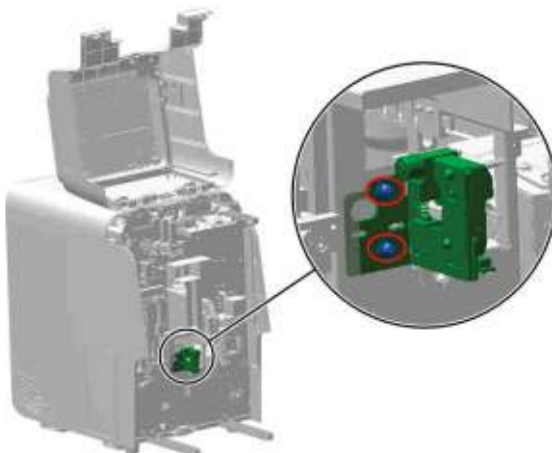
Figure7-160 Removing the stabilizing assembly
