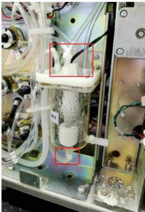
Figure7–421 Diagram of the Pipeline of Waste Cistern Assembly
