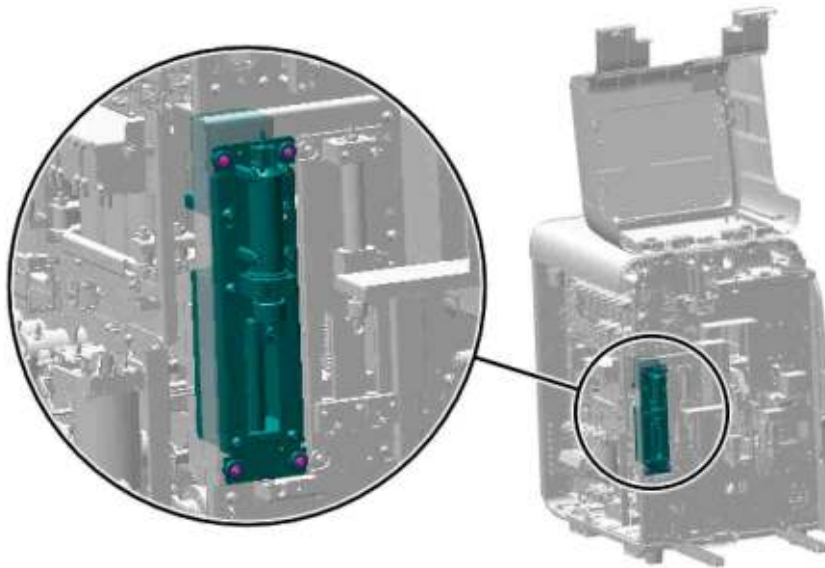
Figure7–109 Positions of the set screws of the 100ul lead screw driving syringe assembly
