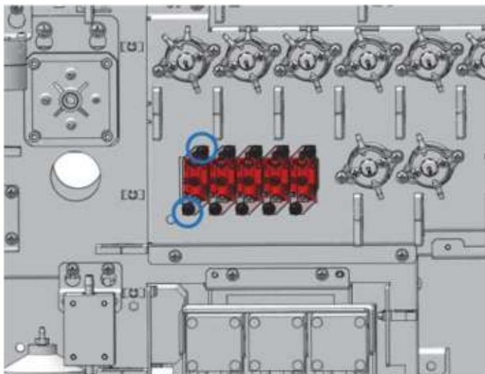
Figure7–535 Positions of the set screws of the LVM valve assembly of two-way
