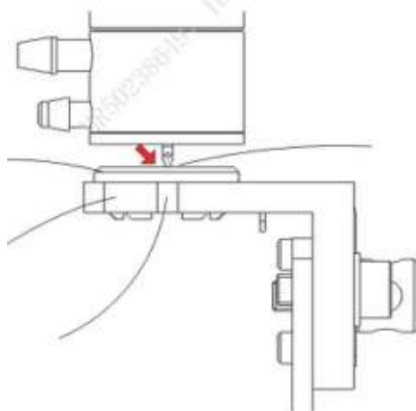
Figure7–195 Observing Sampling Probe Position
