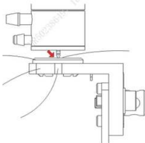
Figure7–237 Observing Sampling Probe Position
