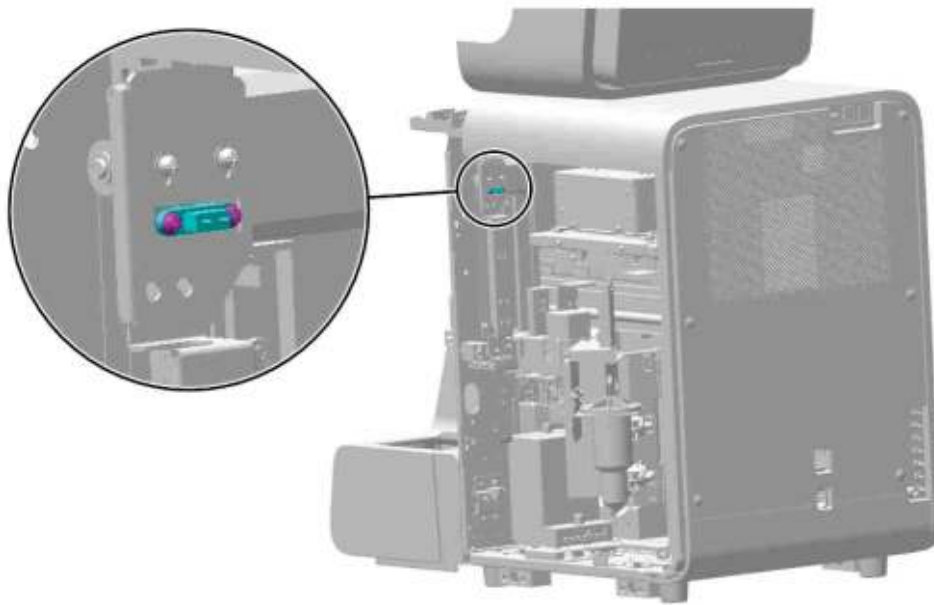
Figure7–138 Positions of the set screws of the photoelectric position sensor (SEN7)
