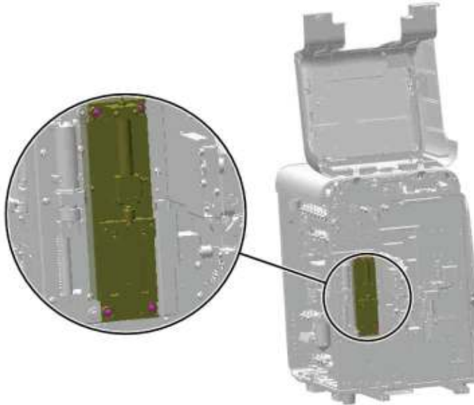
Figure7–118 Positions of the set screws of the 250ul syringe assembly
