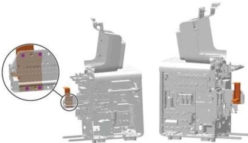
Figure7–24 Removing procedure of the dye bag assembly
