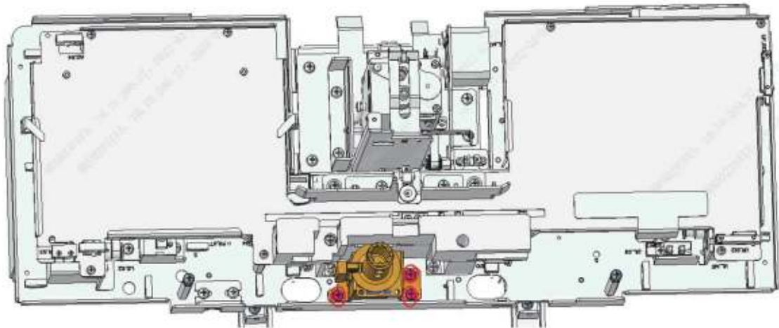
Figure7–219 Removing the capillary blood mix assembly
