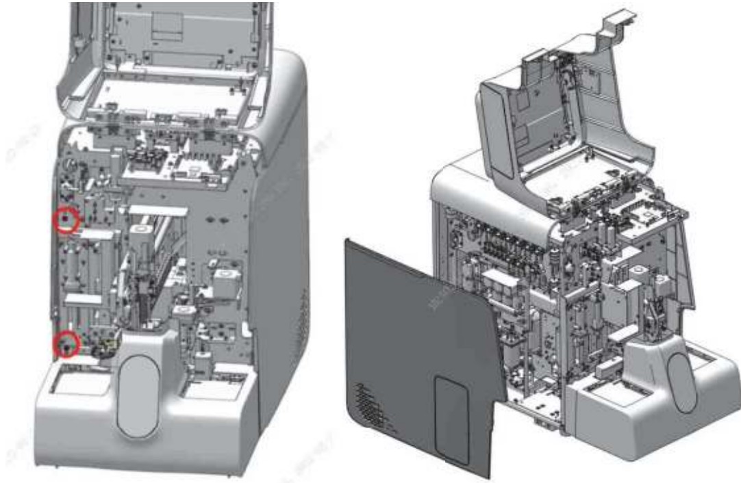
Figure7–533 Diagram B of Removing the Right Cover
