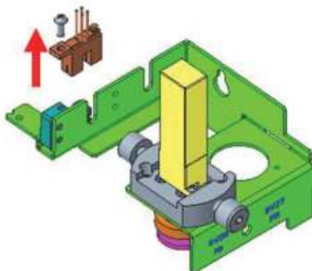
Figure7–573 Diagram of Removing the Transmissive Sensor (Exclude RET)
