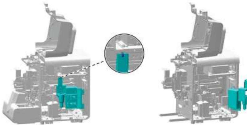
Figure7-71 Opening the right cover assembly
