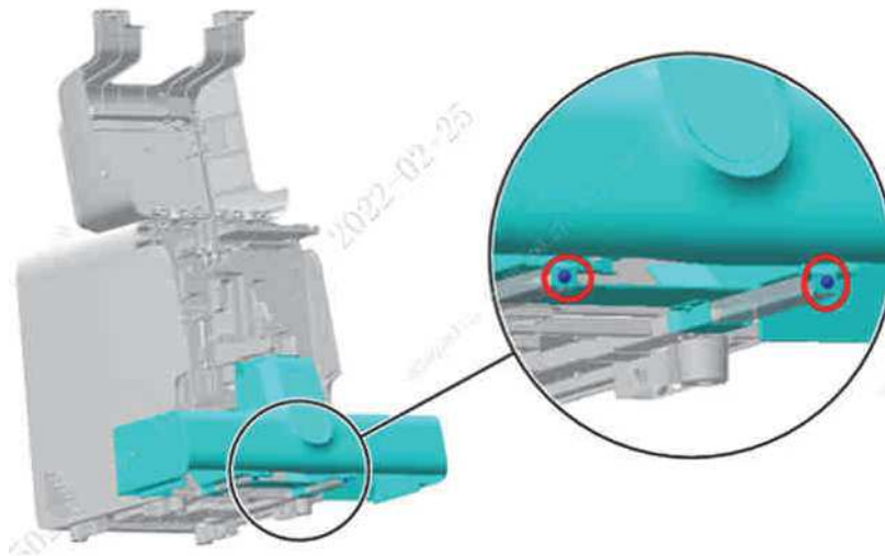
Figure7–265 Opening the front cover
