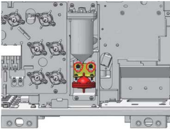
Figure7–555 Set screws of the filter assembly bracket
