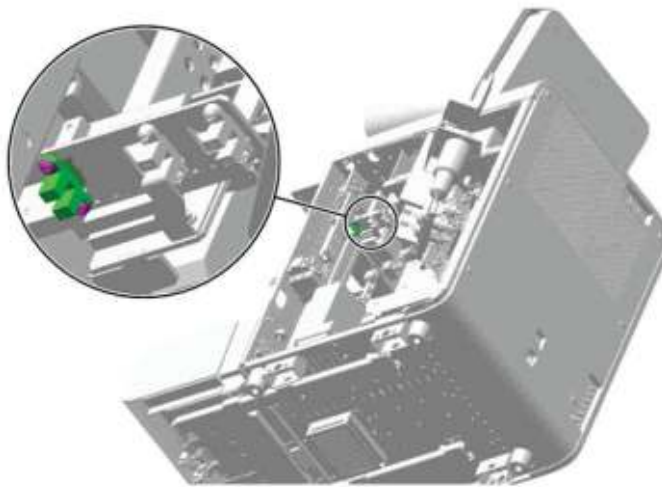
Figure7–130 Positions of the set screws of the photoelectric position sensor (SEN5)
