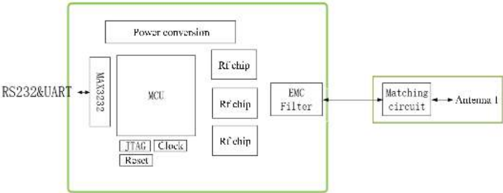
Figure7–618 Functional block diagram of the board
