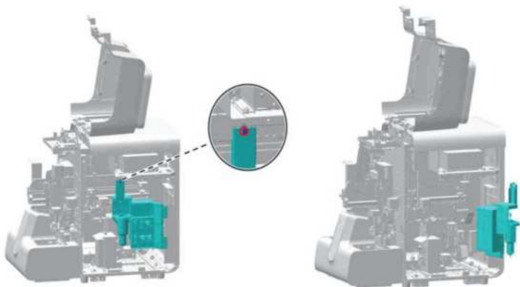
Figure7–661 Opening the right cover assembly
