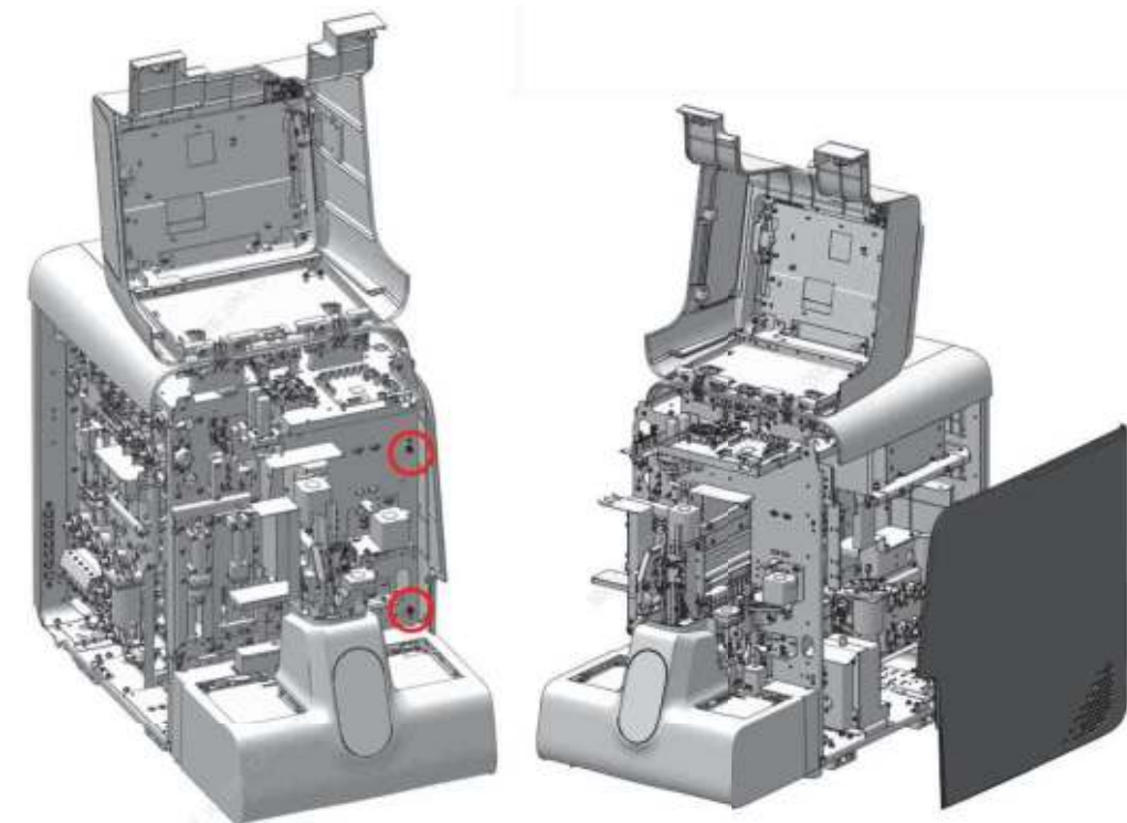
Figure7–533 Diagram B of Removing the Right Cover
