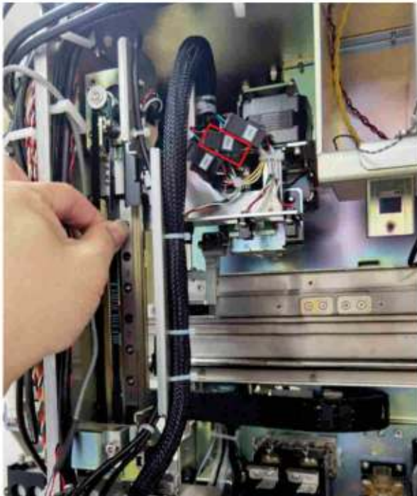
Figure7-142 Removing the photoelectric position sensor (SEN23) wire
