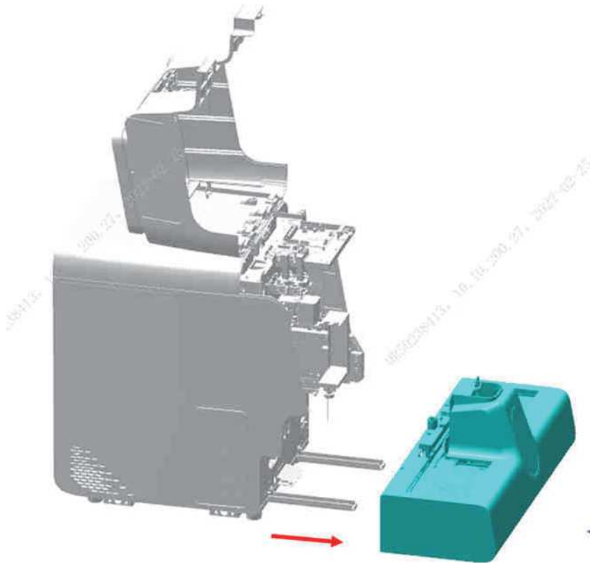
Figure7–292 Removing the autoloader assembly
