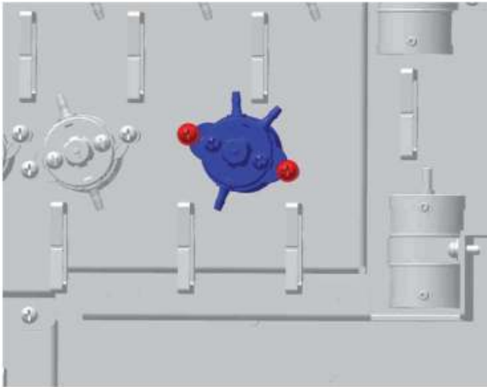
Figure7–529 Positions of the set screws of the high-pressure 3 way value
