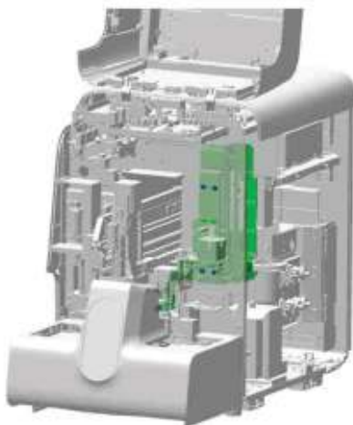
Figure7-166 Figure 1 - Removing the mix assembly
