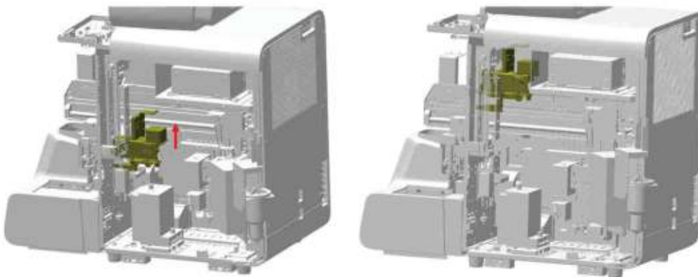
Figure7-128 Binding after lifting the mix Y-direction Assembly
