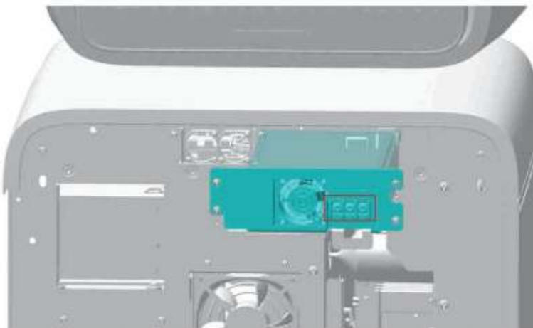
Figure7-663 Figure B of Removing Power Input End Wire
