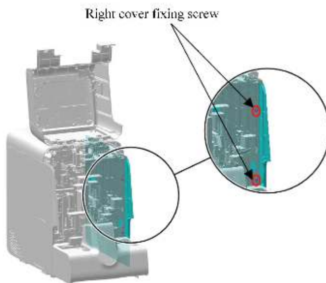
Figure7–396 Removing the right cover
