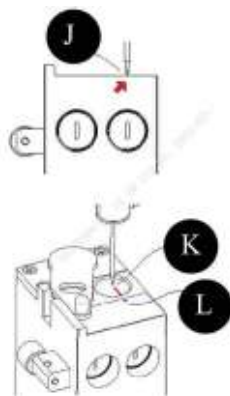
Figure7–51 Diagram of Observe Position
