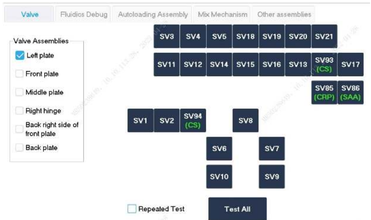
Figure7–520 Valve Self-Test screen
