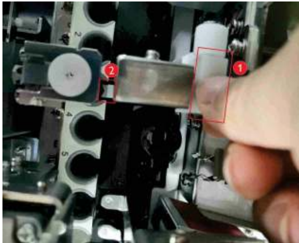
Figure7–351 Ideal Position of the Pincher Roller of the Hold Assembly Relative to the Tube Rack
