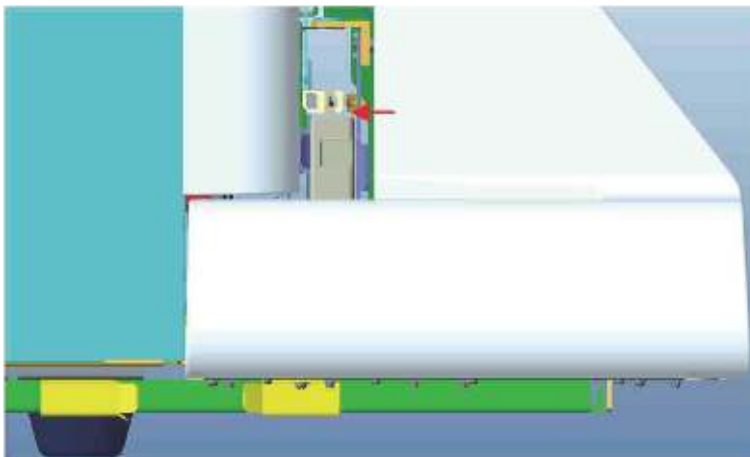
Figure7–360 Confirming the Mixing Gripper Height Position
