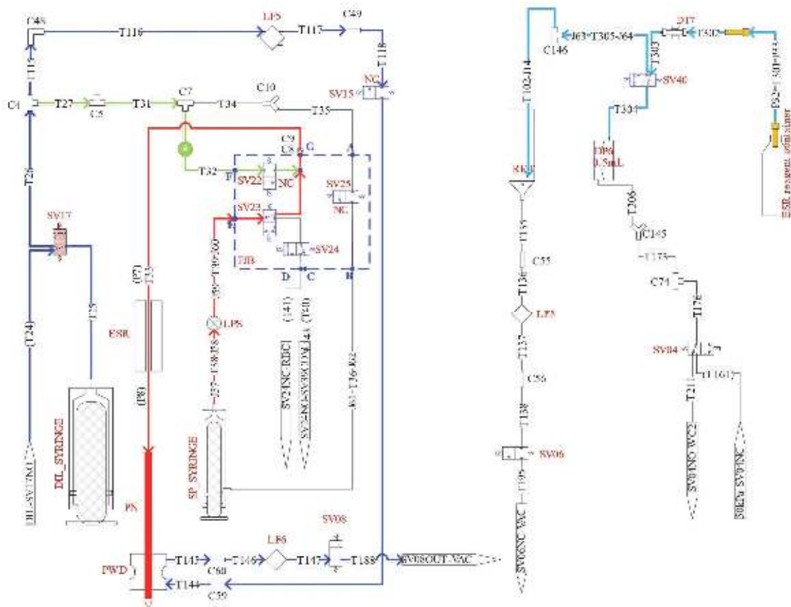
Figure2-38 ESR Measurement Channel
