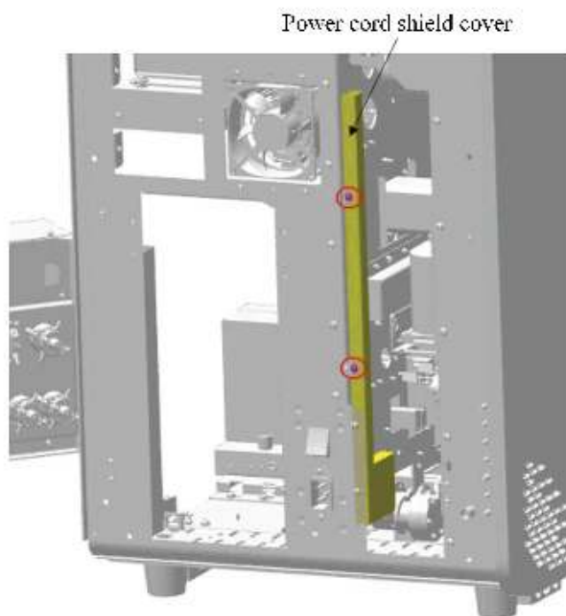
Figure7-665 Figure B of Removing Power Cord Shielding Cover
