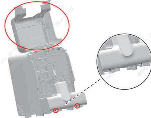
Figure7–278 Opening the front cover
