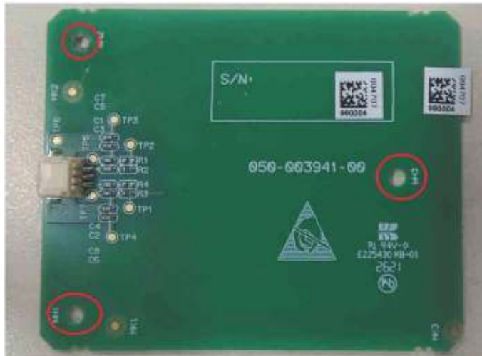
Figure7–627 Diagram of RFID Antenna Screw Installation Positions
