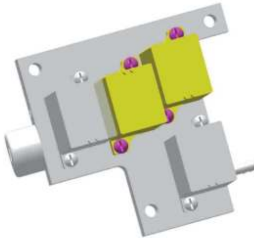
Figure7–482 Diagram of Removing the LVM Fluid Valve Body
