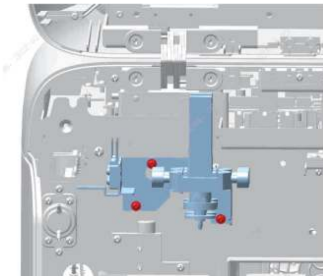
Figure7–564 Diagram of Screw Fixing Location of the Flyorescence Dye Pump Asm (Include RET)
