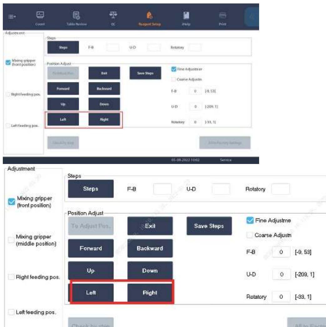
Figure3–46 Mixing Gripper (Front Position) Interface
