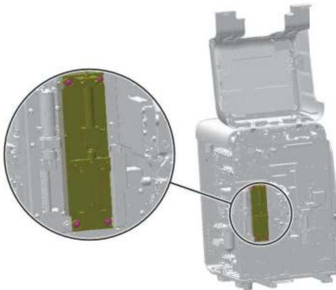
Figure7–458 Positions of the set screws of the 250ul syringe assembly
