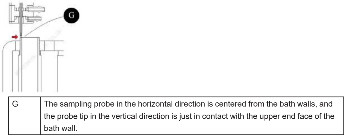
Figure7–44 Adjustment Instructions of Sample Probe to the DIFF Bath Front and Rear Positions and Vertical Height
