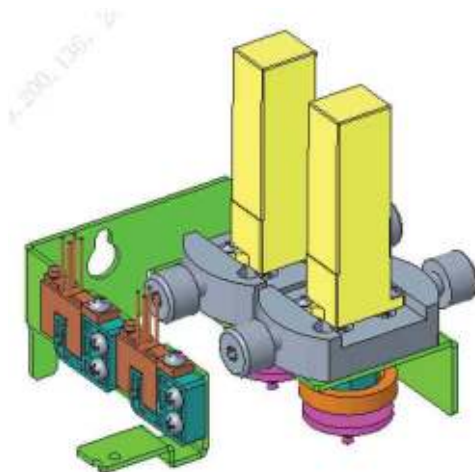
Figure7–561 Photo of Flyorescence Dye Pump Asm (Include RET)
