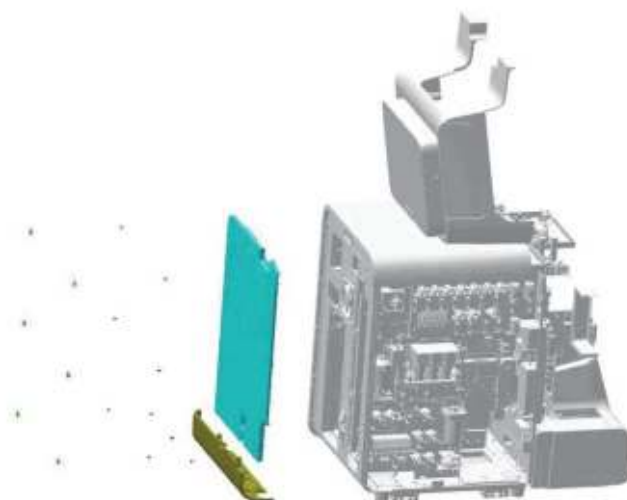
Figure7–469 Diagram of Removing the Rear Cover and Bottom Cover
