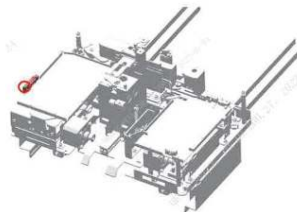
Figure7–259 Diagram of Removing PHOTOELEC Photosensor Reflective 940nm
