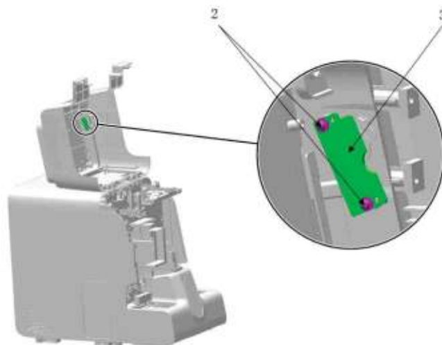
Figure7–9 Figure 2 - Maintenance Procedure of the Switch Key Board PCBA
