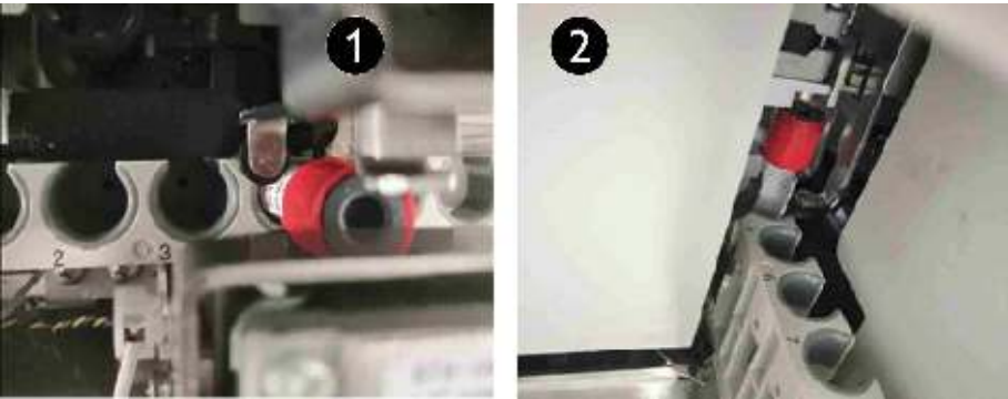
Figure7–311 Ideal Position of the Pincher Roller of the Rotatory Compressing Assembly Relative to the Tube Rack
