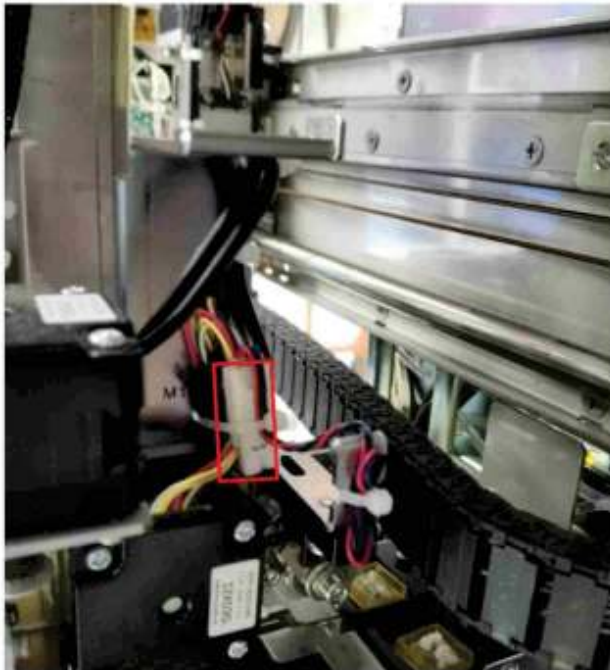
Figure7–82 Removing the detecting sensor wire
