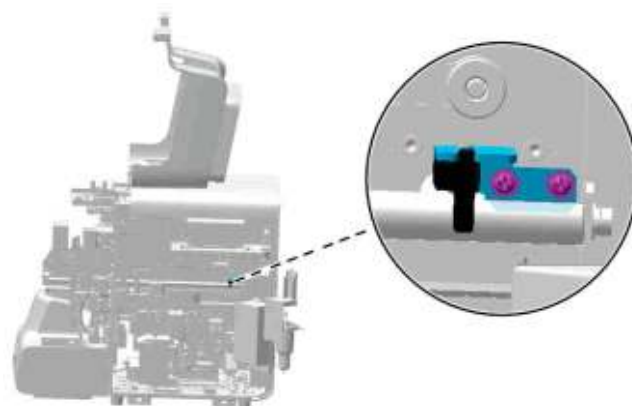
Figure7-73 Removing the small assembly of Y-direction initial position sensor
