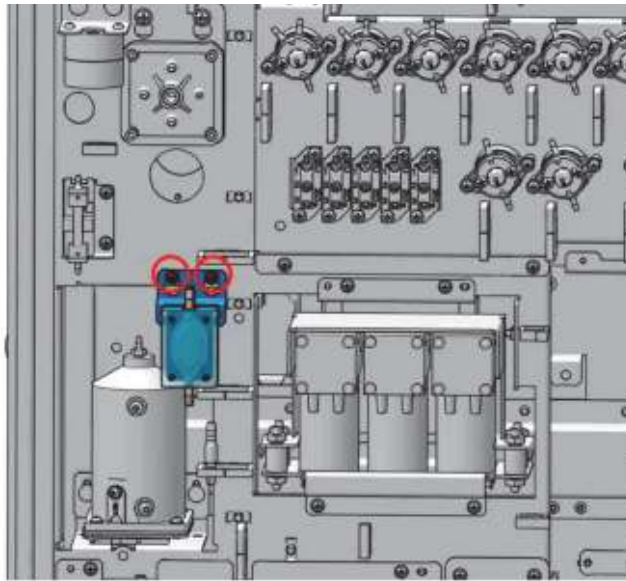
Figure7–546 Positions of the set screws of the sheath fluid filter assembly
