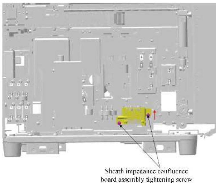
Figure7–501 Diagram of Removing the Sheath Impedance Confluence Board Assem (FRU)
