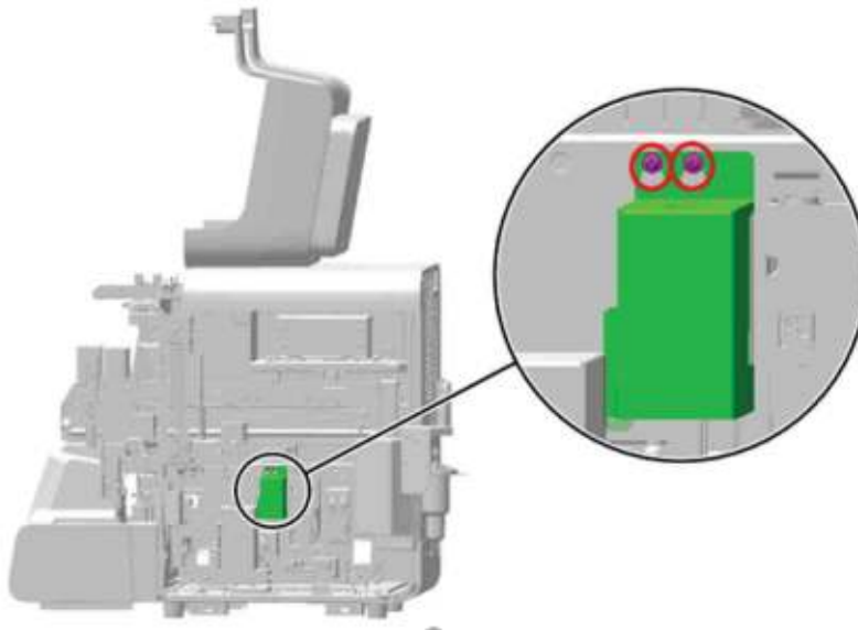
Figure7–404 Positions of the set screws of the HGB bath assembly shielding cover
