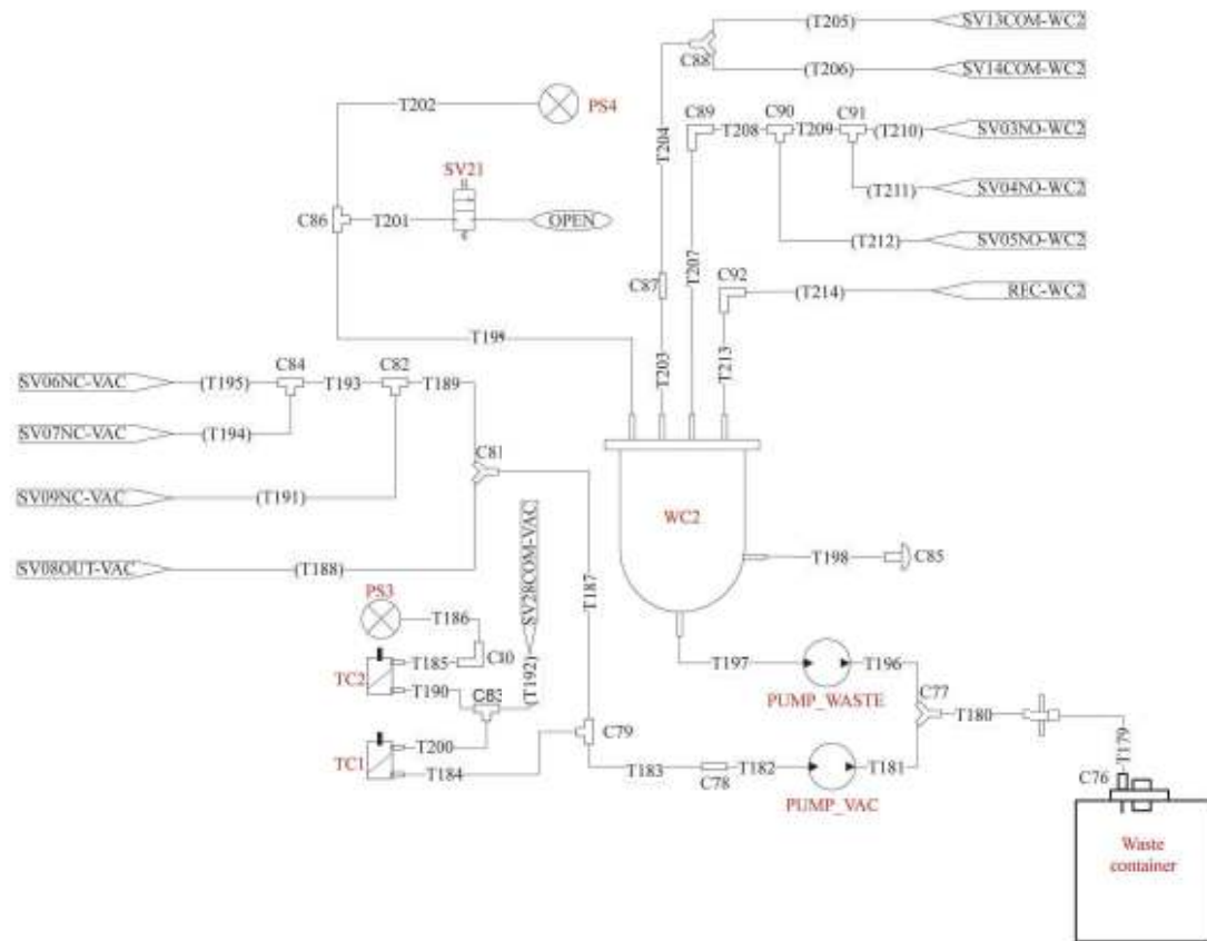
Figure2–32 RET Measurement Waste Channel
