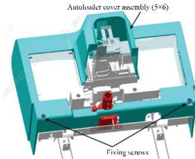
Figure7–333 Removing autoloader front cover assembly (5x6)
