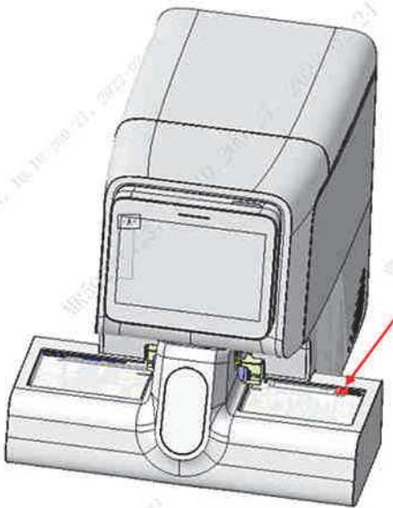
Figure7-263 Diagram of Location of PHOTOELEC Emitter 940nm 400mm conn in the Main Unit
