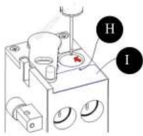
Figure7–48 Default Adjust Position of Sample Probe CT-WB Position
