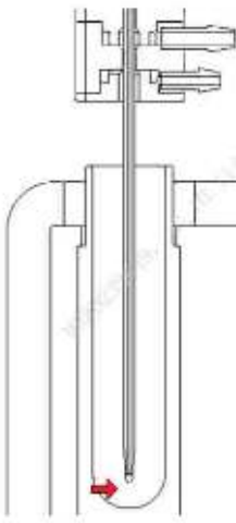
Figure7–46 Check Position of the Sample Probe Relative to the DIFF Bath
