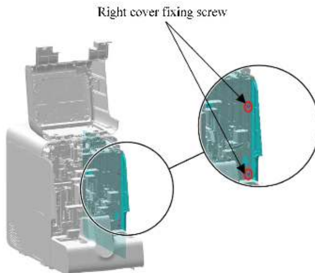
Figure7–649 Diagram of Removing the Right Cover
