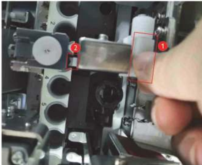
Figure3–42 Ideal Position of the Finger Pressure Block of the Hold Assembly Relative to the Tube Rack
