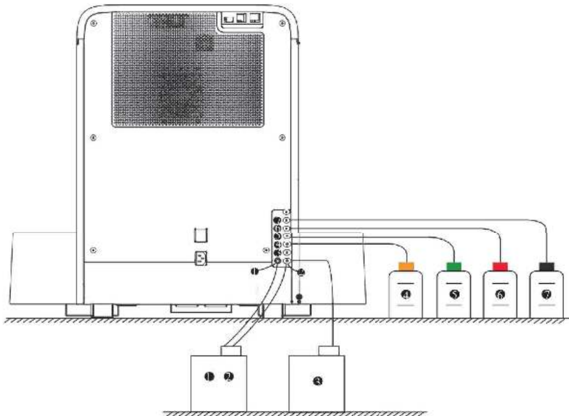
Figure3–14 Reagent Connection - Lyse, Diluent, Waste
