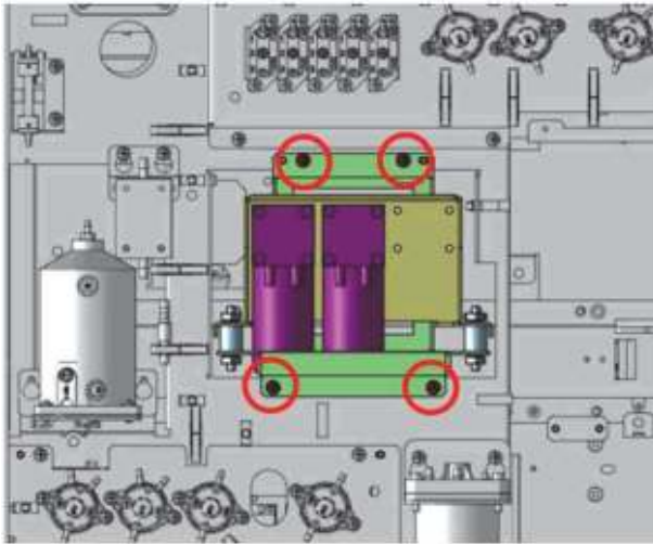
Figure7–542 Positions of the Fixing Screws of the Waste Pump Assembly
