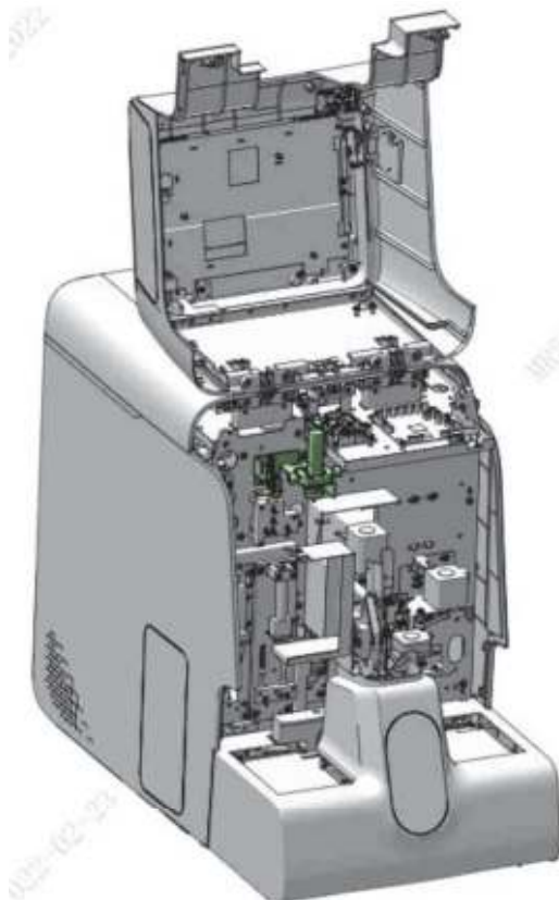
Figure7–583 Diagram of Removing the Flyorescence Dye Pump Asm (Exclude RET)
