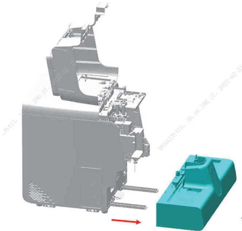
Figure7–328 Removing the 10x5 closed autoloader (FRU)
