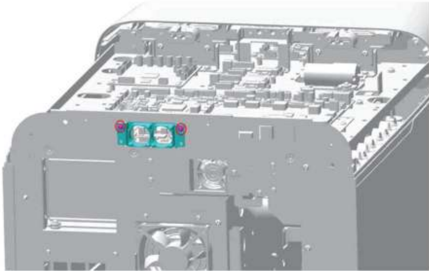
Figure7–639 Diagram of Removing the Board Fan Assembly
