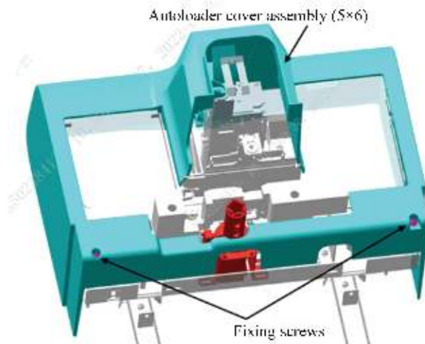
Figure7–258 Removing autoloader front cover assembly (5x6)
