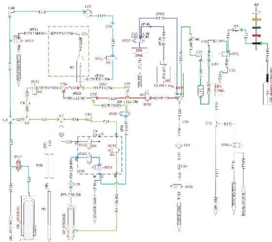
Figure2–31 RET Measurement Channel
