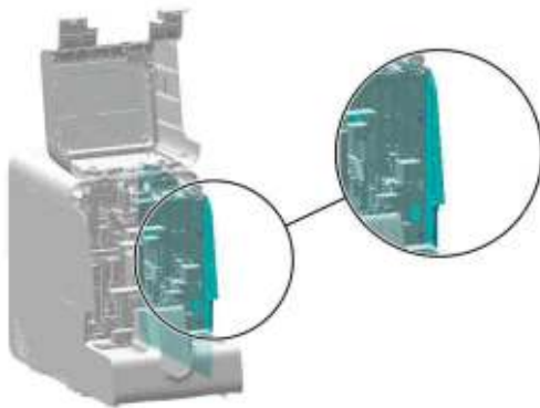
Figure7–373 Removing the right cover
