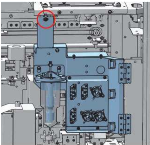
Figure7–506 Diagram A for Locations of Right Bath Subassembly Fixing Screws
