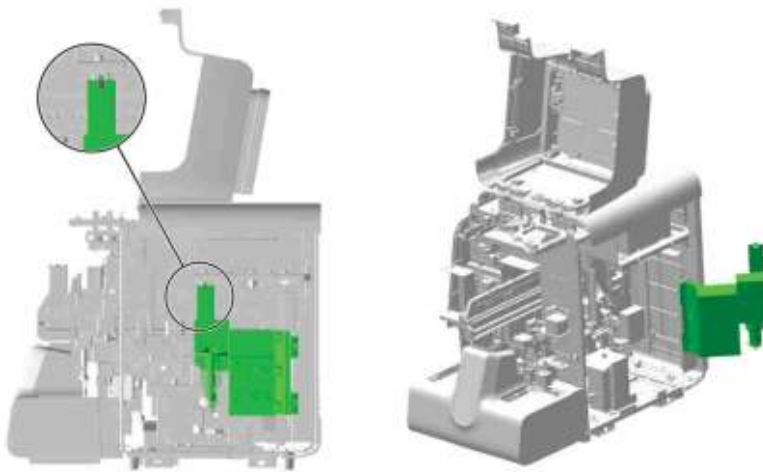
Figure7-136 Opening the right cover assembly
