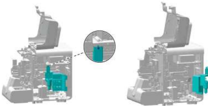
Figure7-76 Opening the right cover assembly
