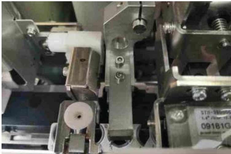
Figure7–315 Observing the Mixing Gripper Position
