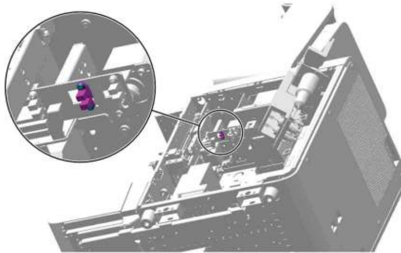
Figure7–143 Positions of the set screws of the photoelectric position sensor (SEN23)
