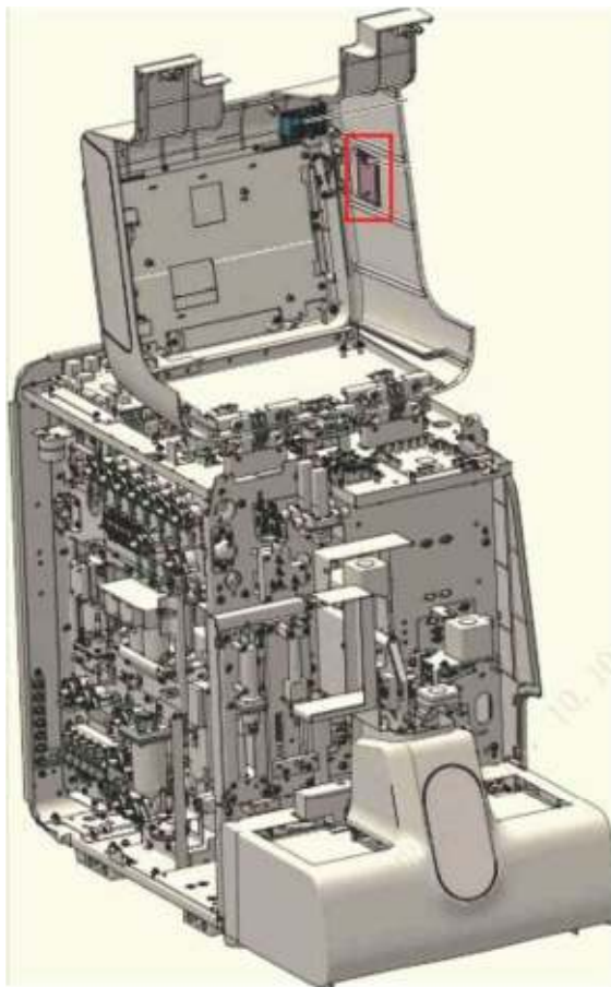
Figure7–626 Opening the front cover
