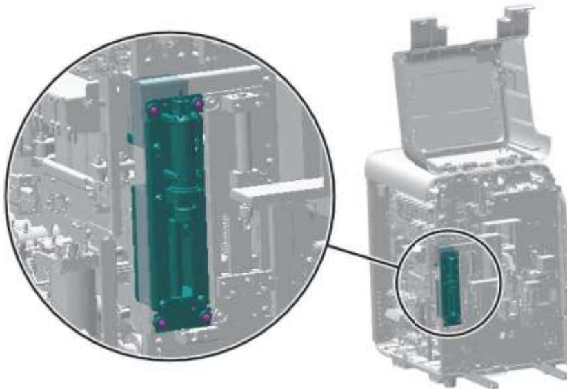
Figure7–451 Positions of the set screws of the 100ul lead screw driving syringe assembly
