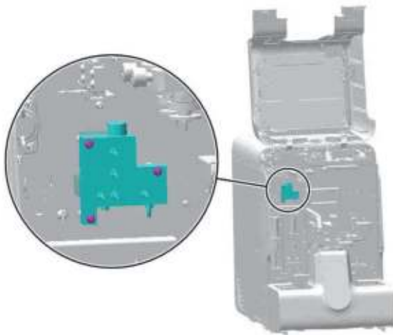
Figure7–481 Positions of the set screws of the air tank assembly
