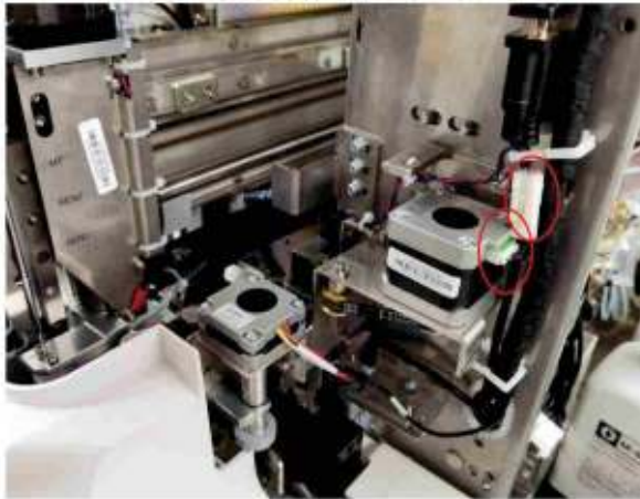
Figure7-178 Removing the wire for the rotary fixing assembly
