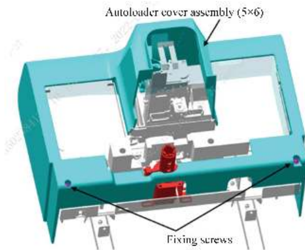
Figure7–222 Removing autoloader front cover assembly (5x6)
