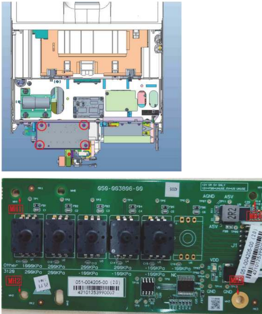
Figure7–602 Positions of screws of air pressure detection board
