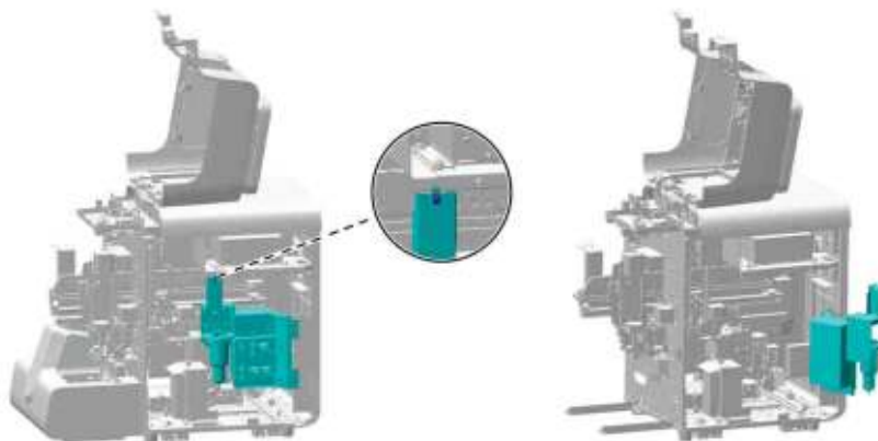
Figure7–374 Diagram of Opening the Right Cover
