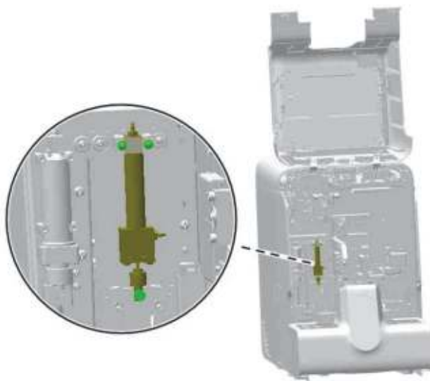
Figure7–463 Positions of set screws of Mindray 250 \mu L syringe (with connector)
