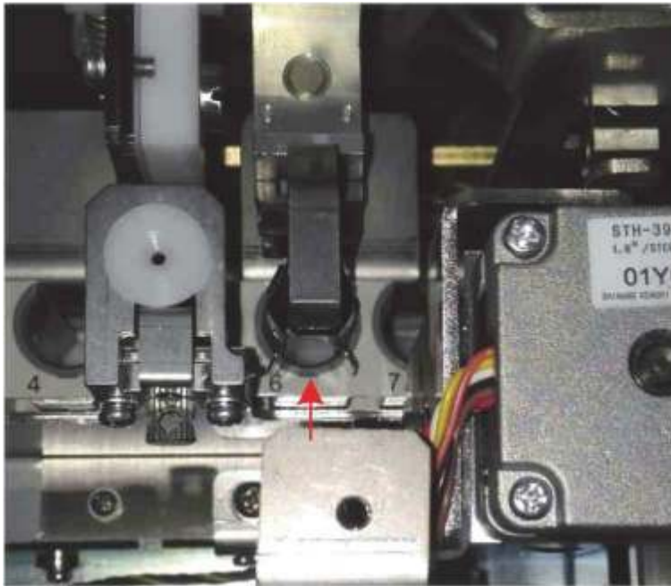
Figure7–359 Observing the Mixing Gripper Position
