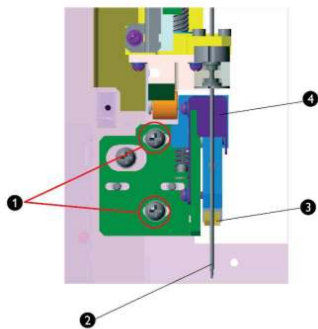
Figure7–161 Left/Right Position Adjustment of the Hold Assembly
