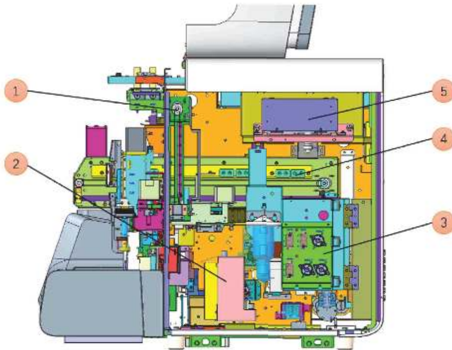
Figure2–6 Right Side of the Analyzer (Right Cover Open)
