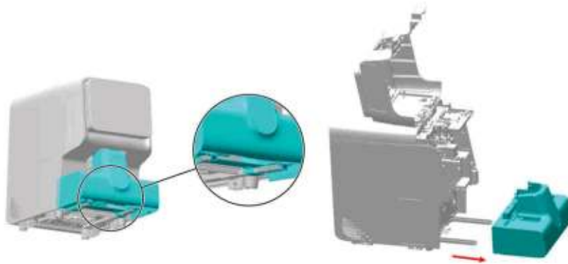
Figure7-115 Removing the autoloader
