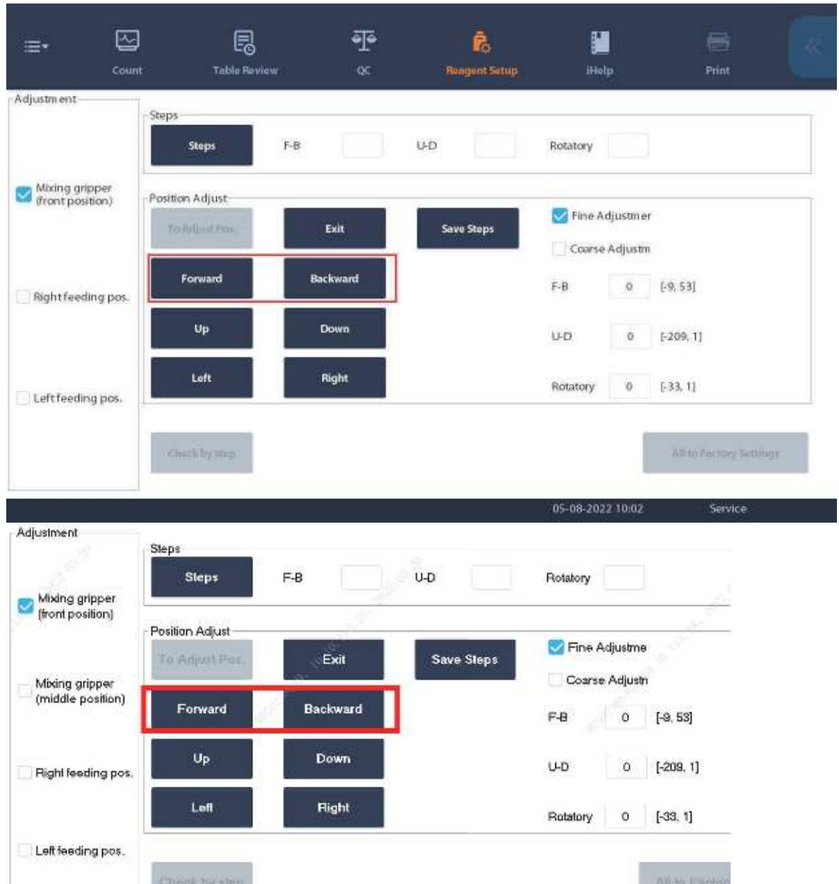
Figure3–47 Mixing Gripper (Front Position) Interface
