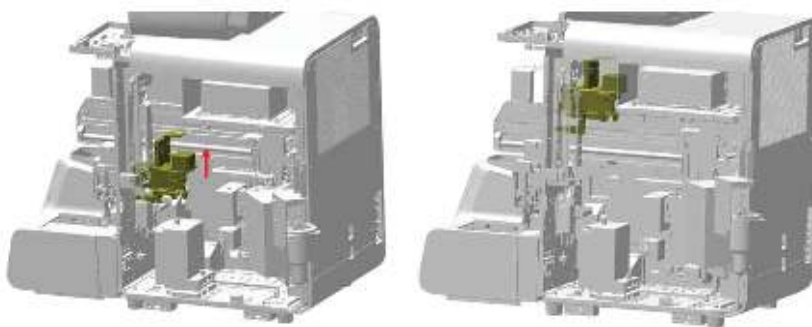
Figure7–83 Binding after lifting the mix Y-direction Assembly
