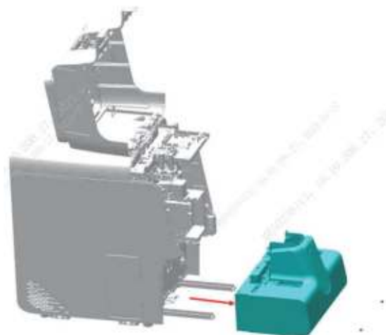
Figure7–193 Removing the 5x6 closed autoloader (including capillary blood mixing) FRU)
