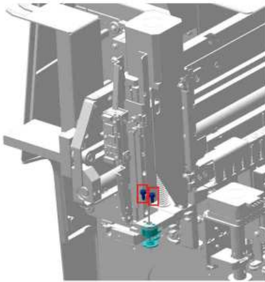
Figure7–151 Removing the probe wipe (closed-sampling)
