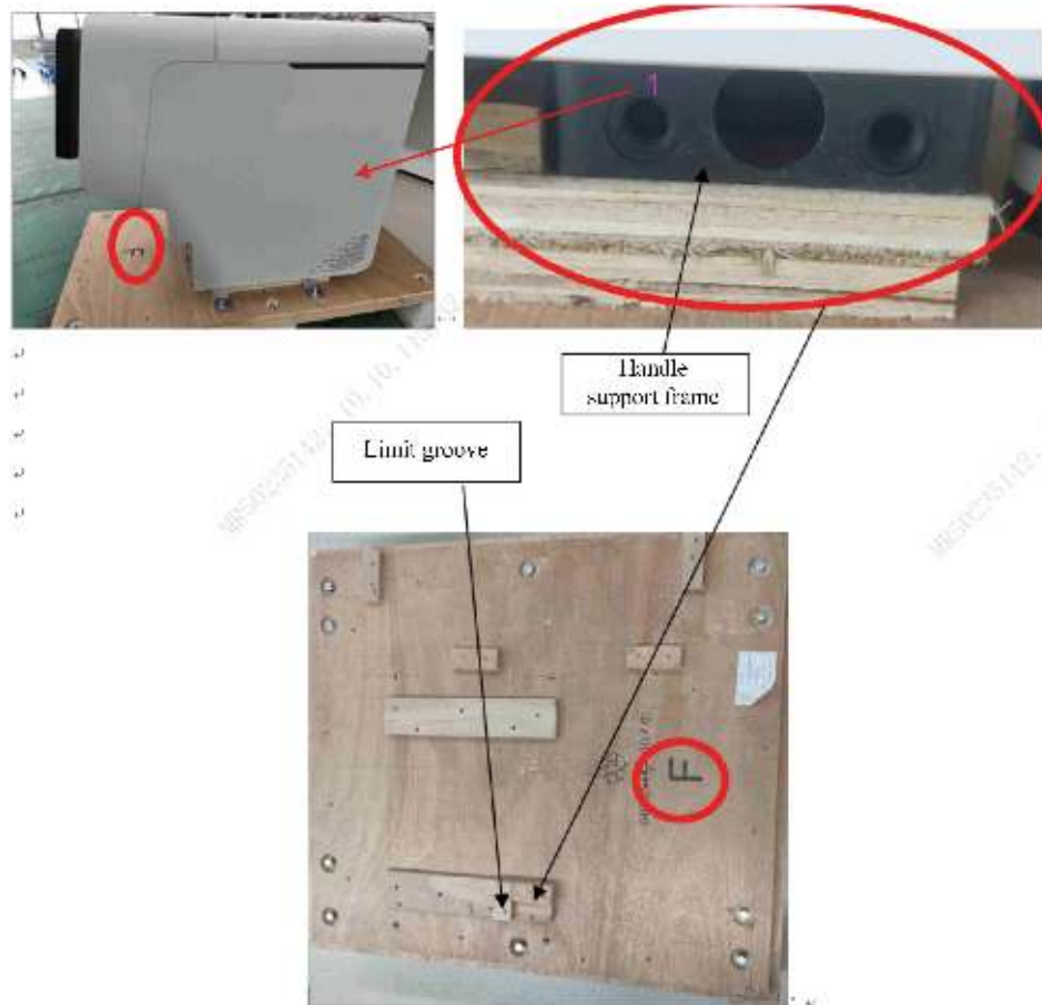
Figure9–12 Placing the Main Unit (Analyzer)
