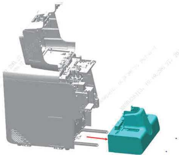
Figure7–270 Removing the autoloader assembly
