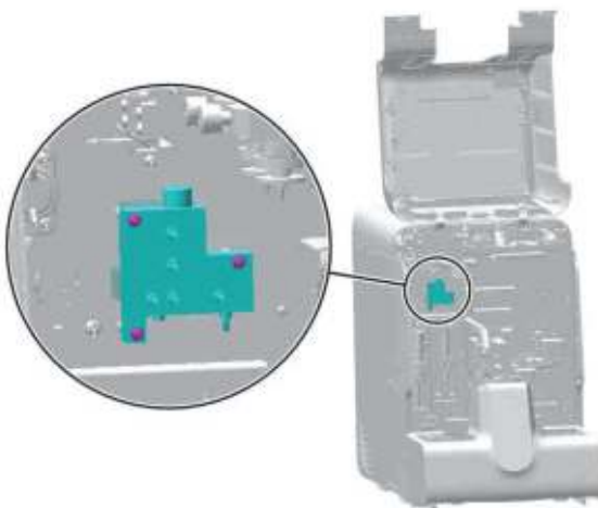
Figure7–491 Positions of the set screws of the air tank assembly
