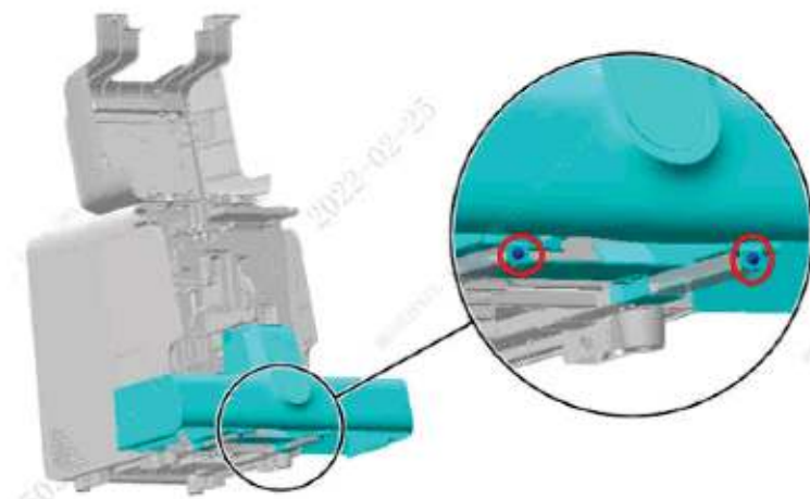
Figure7–303 Opening the front cover
