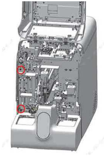
Figure7–548 Diagram of Removing the Left Cover
