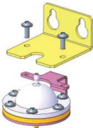
Figure7–556 Removing the filter assembly (injection)
