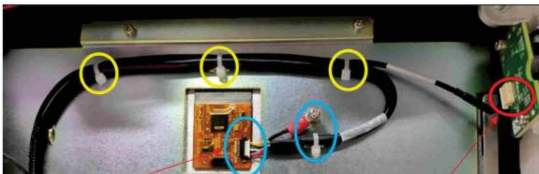
Figure7–12 Touch screen cable and switch key cable
