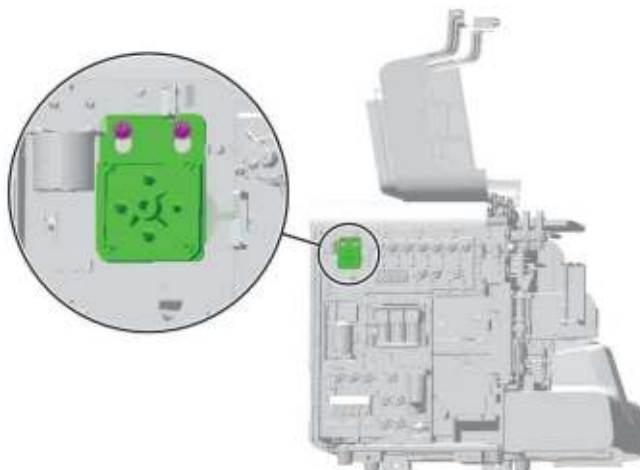
Figure7–434 Positions of the set screws of the air tank assembly
