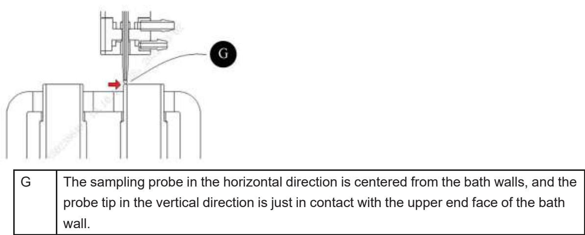
Figure7–39 Adjustment instructions of sampling probe to the reaction bath front and rear positions and vertical height
