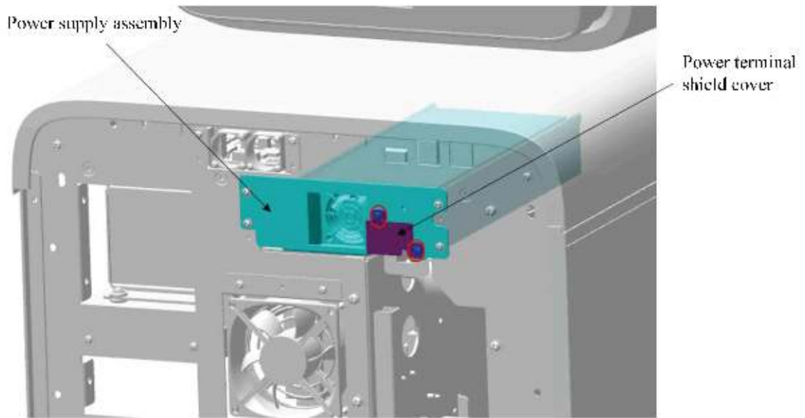
Figure7-663 Figure B of Removing Power Input End Wire
