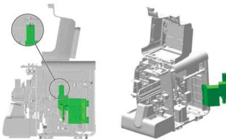
Figure7–122 Opening the right cover assembly
