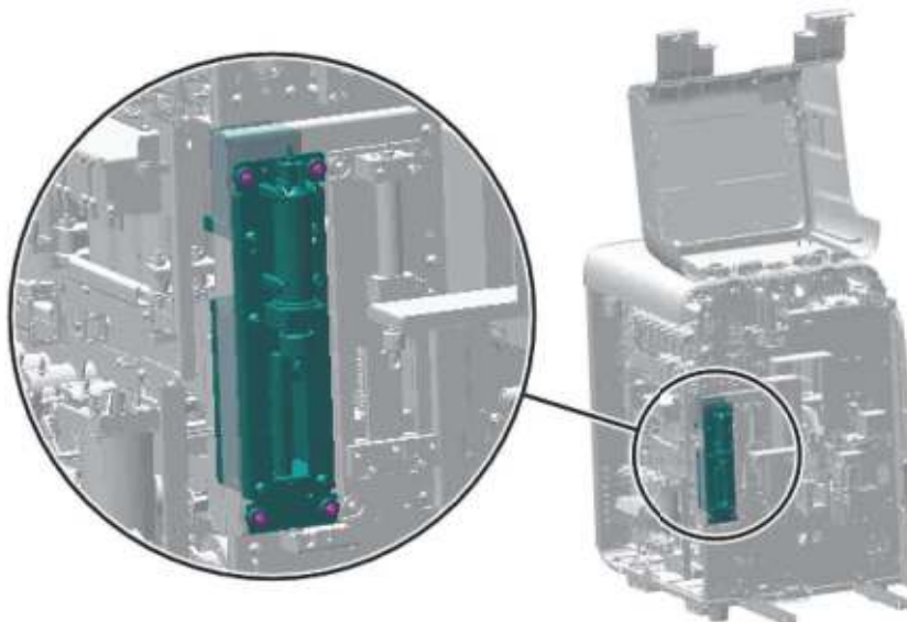
Figure7-445 Positions of the set screws of the 100ul lead screw driving syringe assembly
