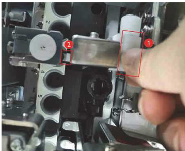
Figure7–198 Ideal Position of the Pincher Roller of the Hold Assembly Relative to the Tube Rack
