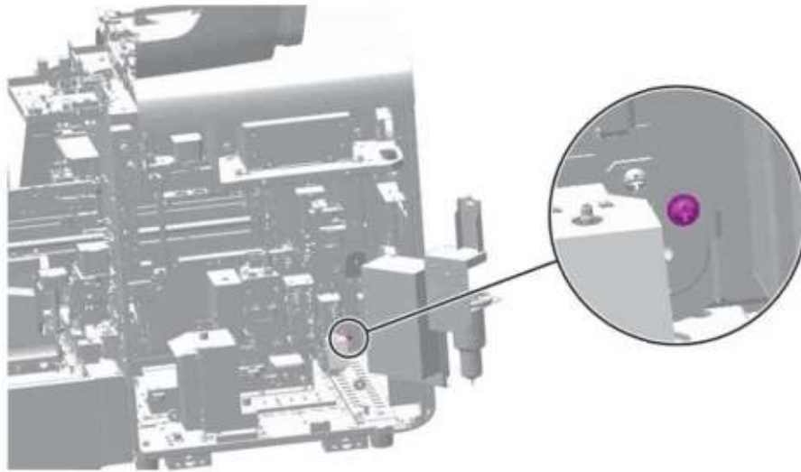
Figure7-665 Figure B of Removing Power Cord Shielding Cover
