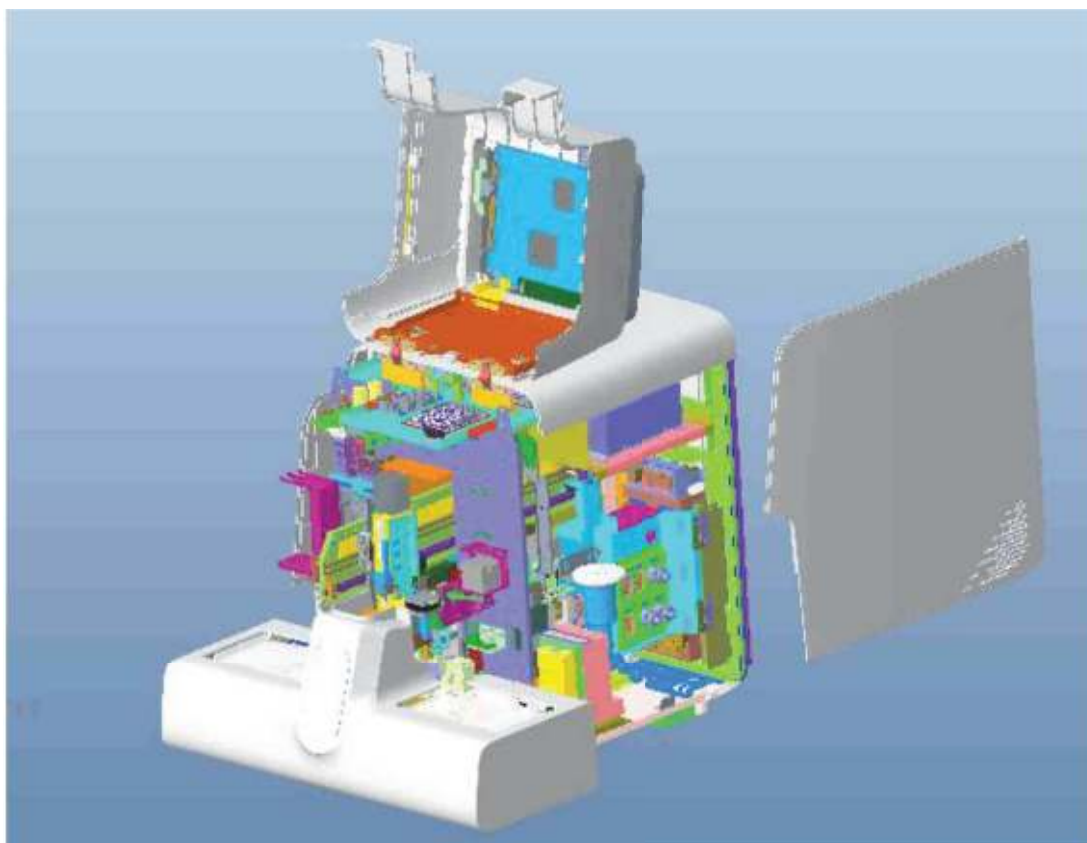
Figure7-600 Opening the front cover
