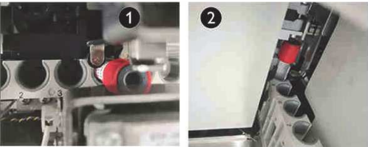
Figure7–242 Ideal Position of the Pincher Roller of the Rotatory Compressing Assembly Relative to the Tube Rack
