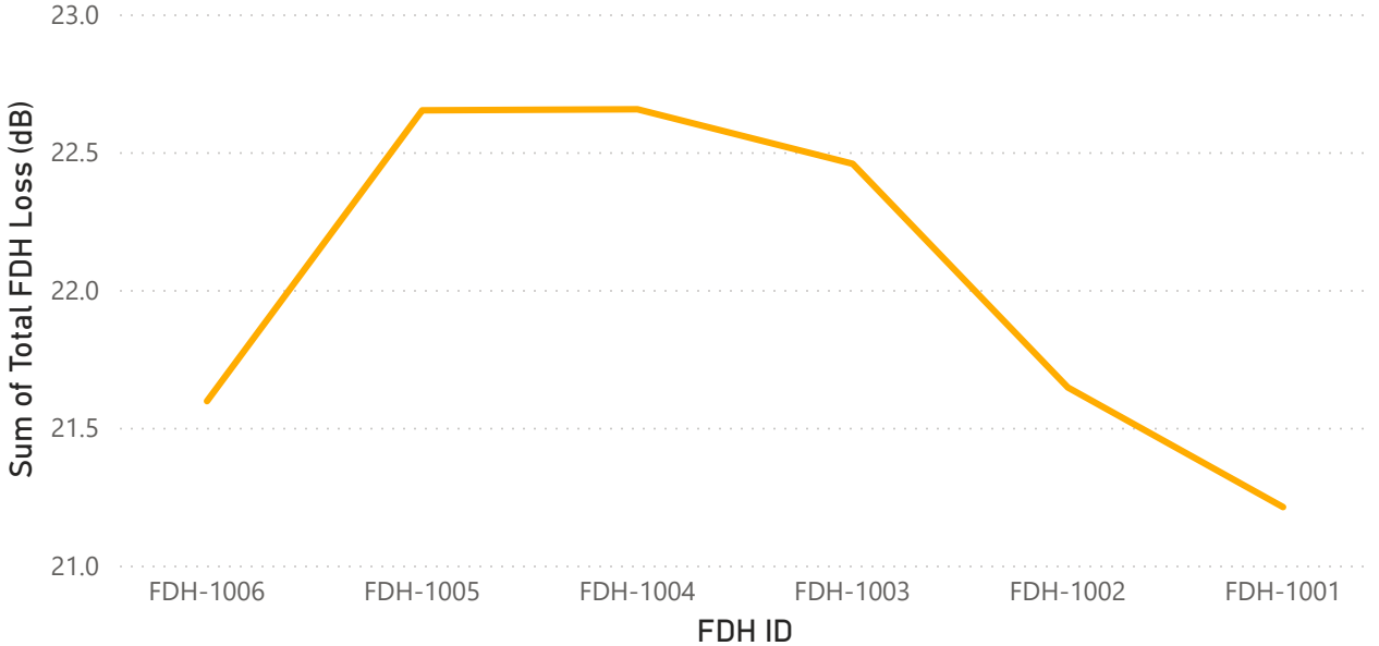
FDH Link Loss Analysis (dB)
