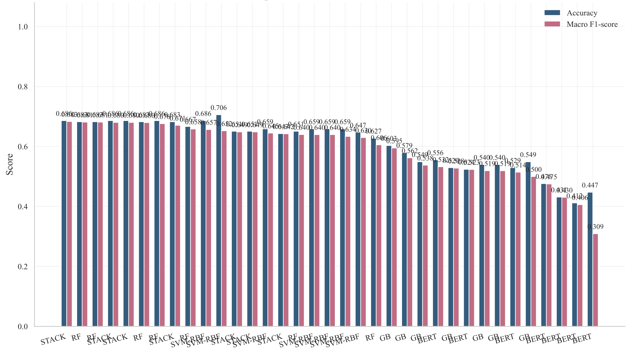
Performance Comparison of Models on LIAR Dataset (Test Set)
