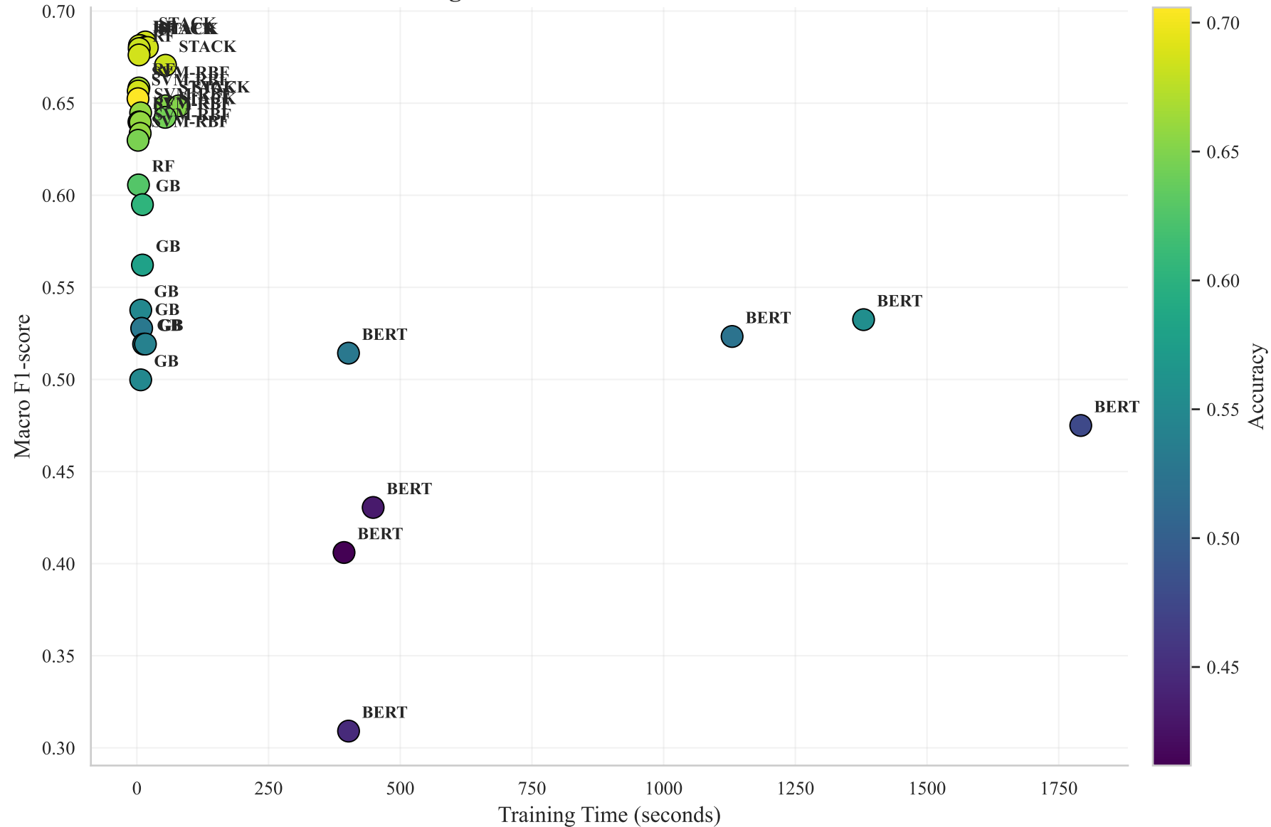
Training Time vs Macro F1-score Trade-off
