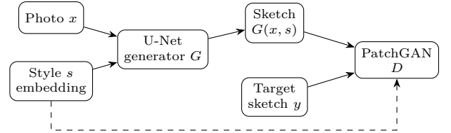
Fig. 4. Task 4 conditional GAN. The style embedding enters both G and D (dashed); D outputs a map of local real/fake scores.
