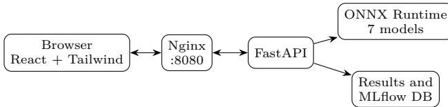
Fig. 37. Deployment: two Docker Compose services; model and result files are mounted read-only into the backend.
