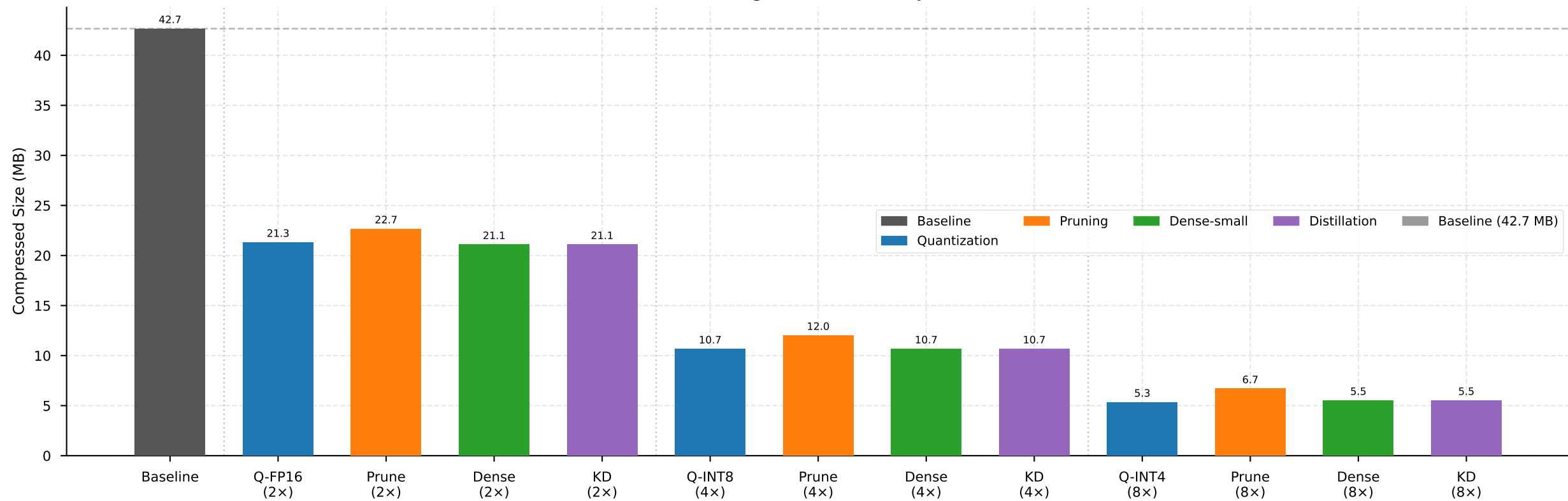
Model Storage Size After Compression
