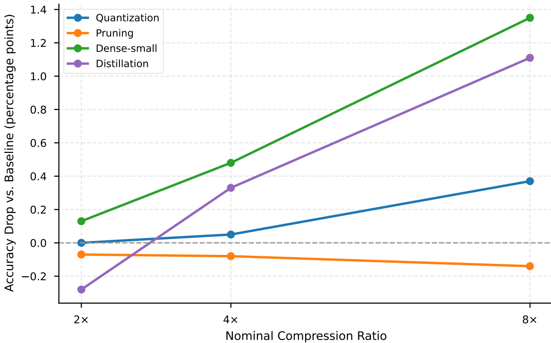
Accuracy Degradation Under Compression
