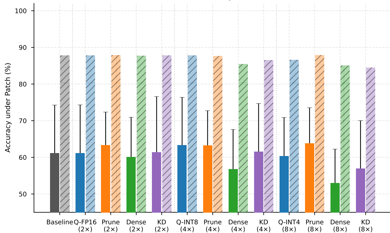
Universal Attack — Side-8 patch (6.25% area)
