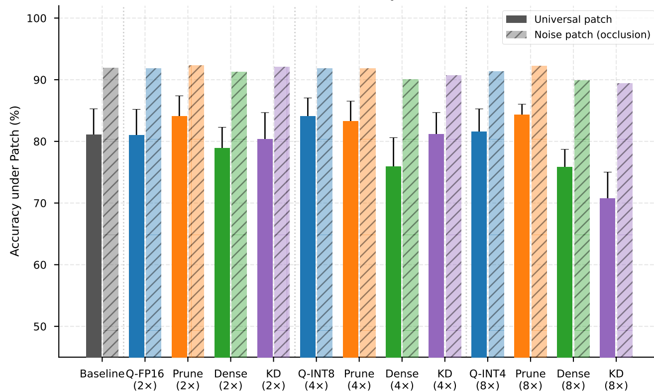
Universal Attack — Side-5 patch (2.4% area)
