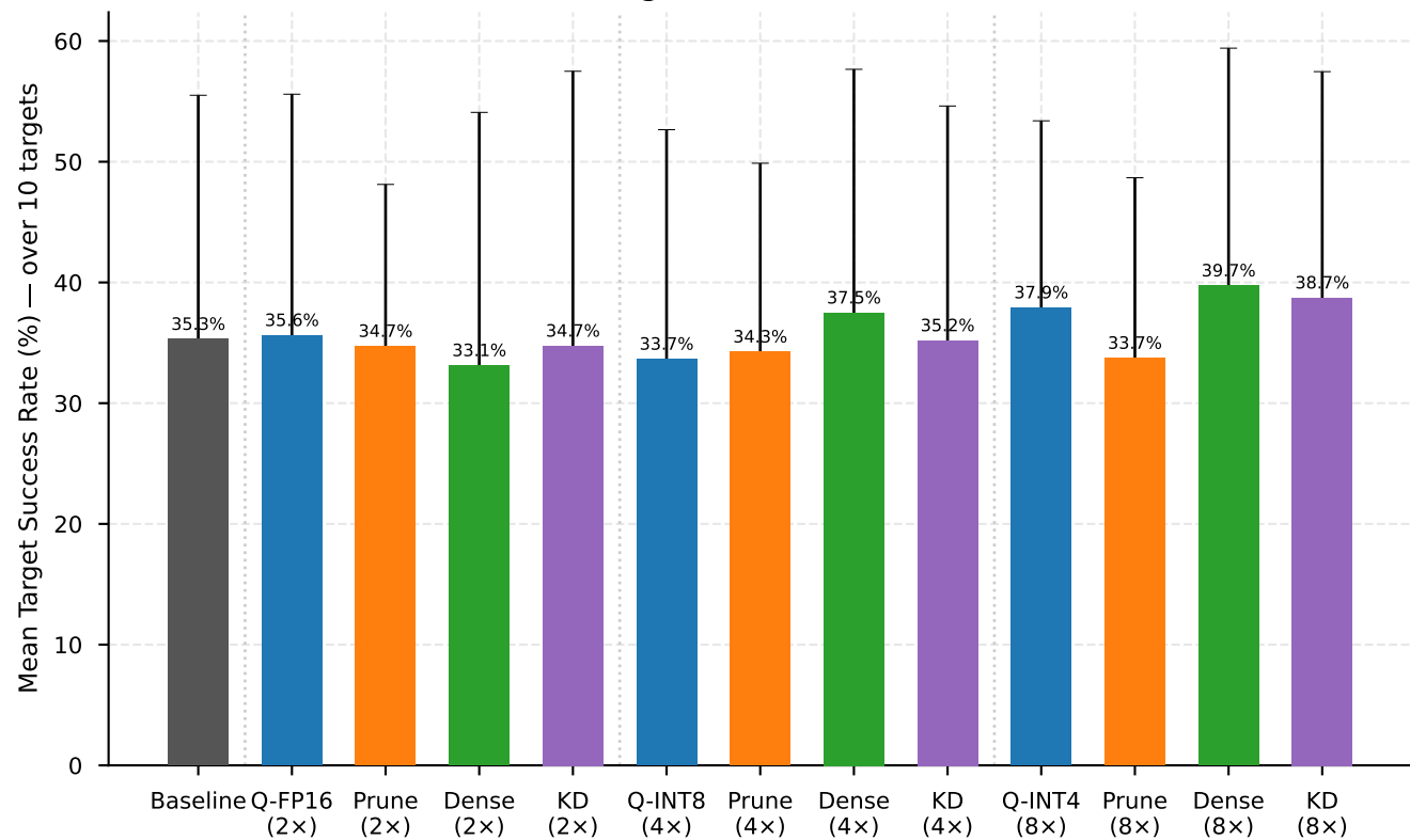
Universal Patch Target Success — Side-8 (6.25% area)
