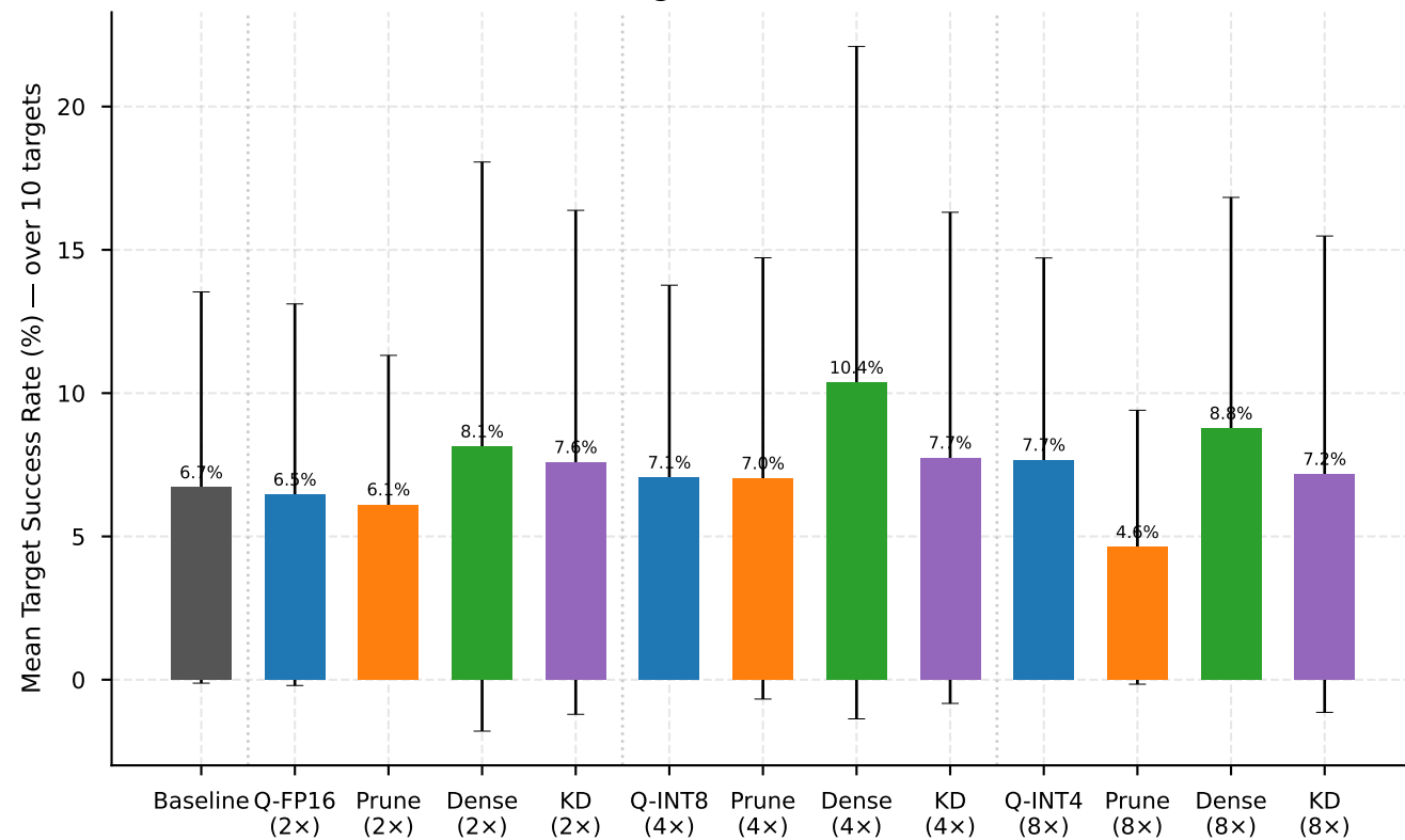
Universal Patch Target Success — Side-5 (2.4% area)
