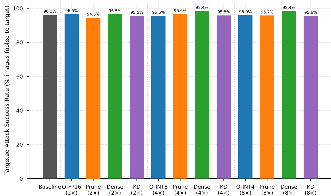
LaVAN Targeted — Side-8 (6.25% area)
