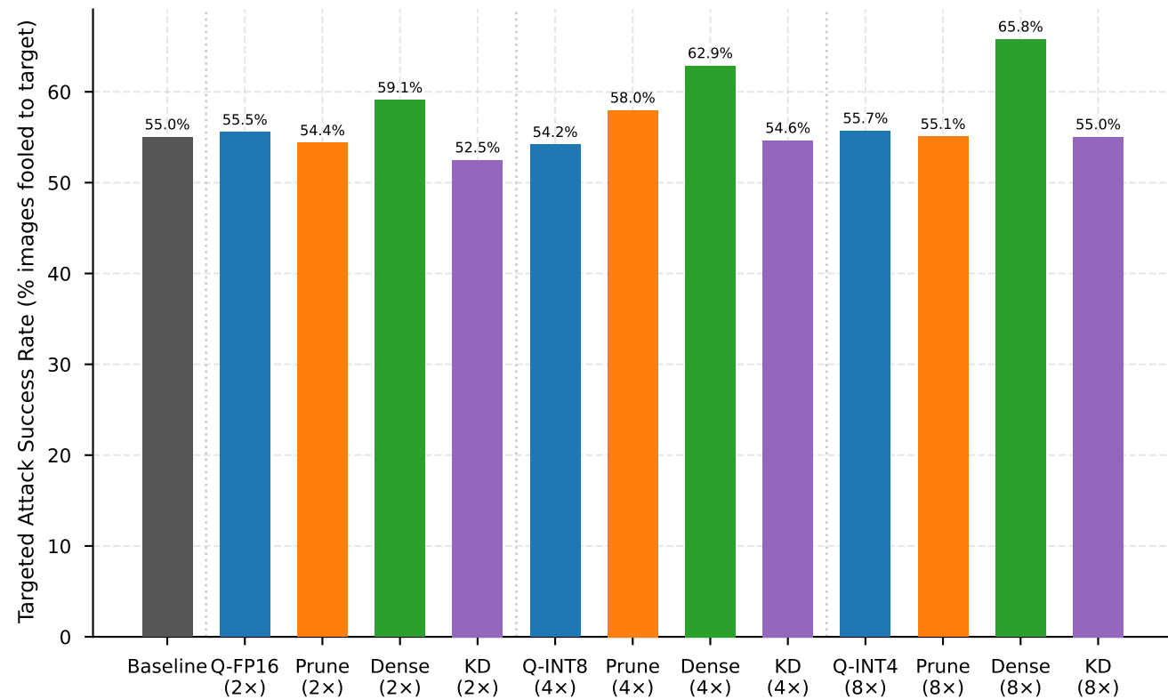
LaVAN Targeted — Side-5 (2.4% area)
