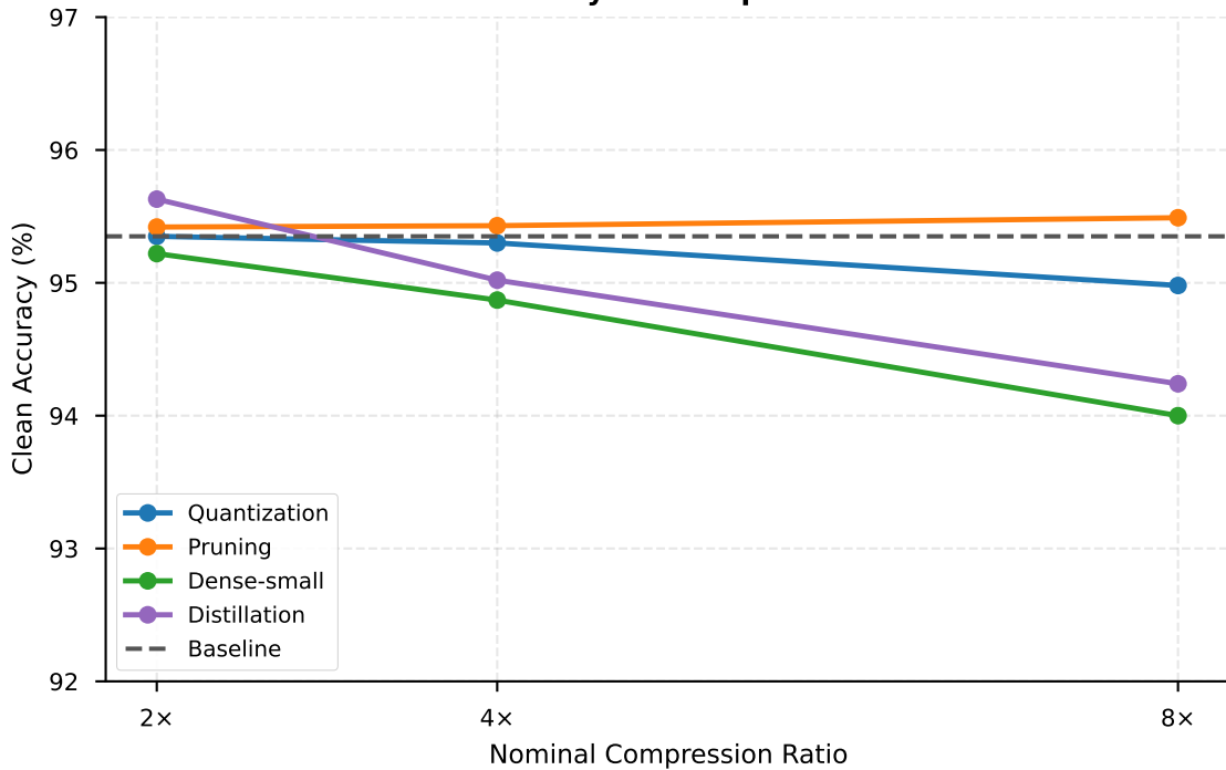
Clean Accuracy vs. Compression Ratio
